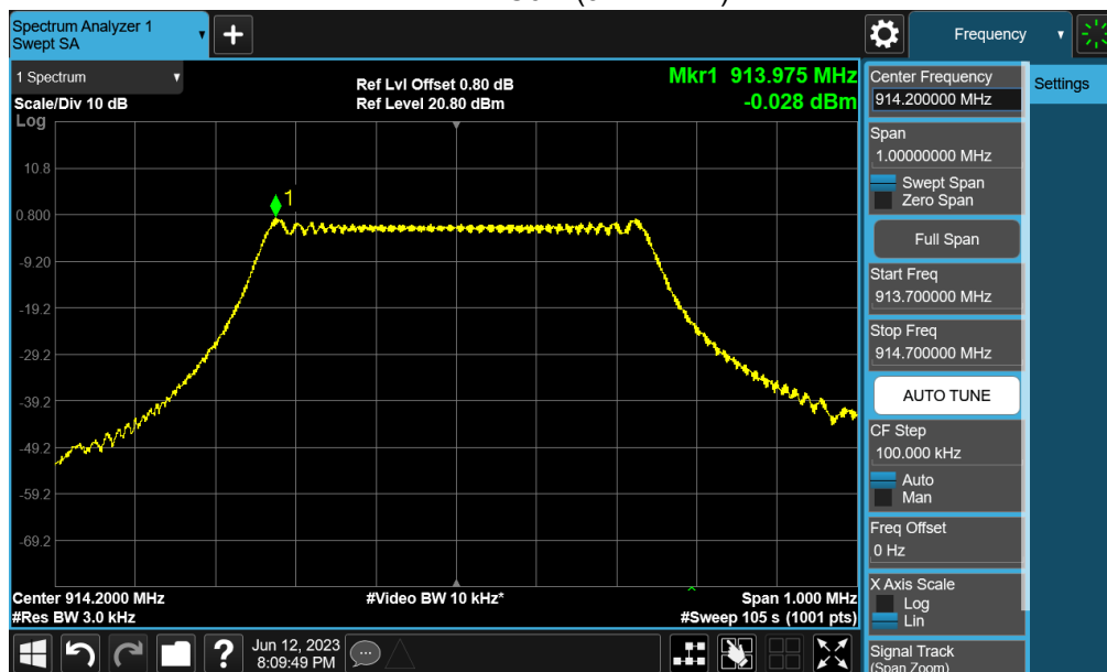
Mode 2 C671(914.2MHz)
