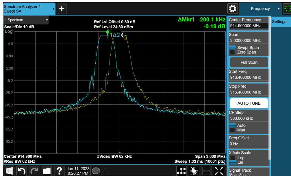
Channel63 914.9MHz
