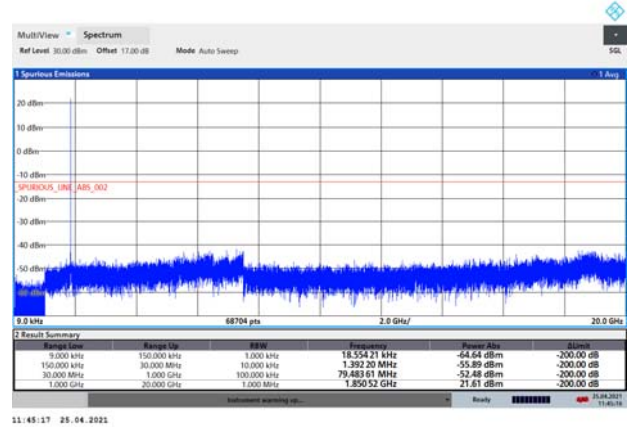
LTE Band 2 3MHz CH-Middle 9kHz~20GHz
