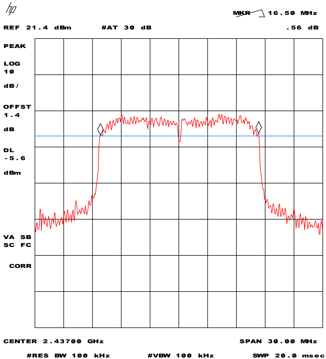
Plot 15 - Minimum 6 dB bandwidth at a transmission bit-rate of 24 Mbit/s.
