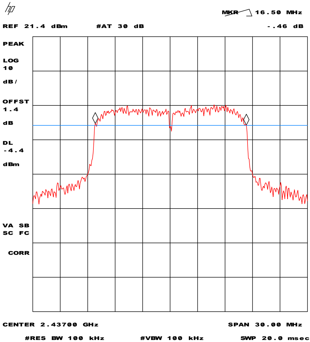
Plot 14 - Minimum 6 dB bandwidth at a transmission bit-rate of 12 Mbit/s.
