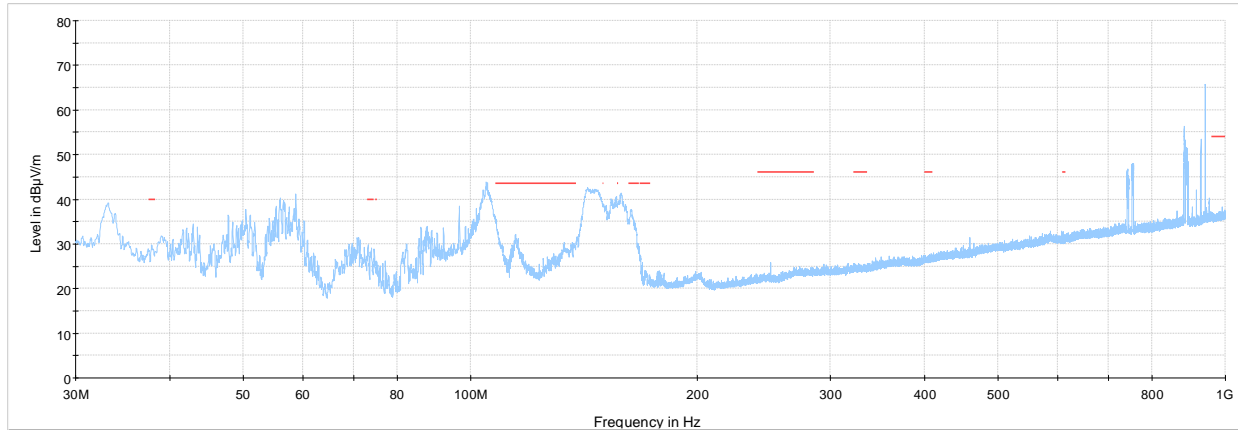
368533 30 MHz - 1 GHz collocation scenario 3 Preview Result 1-PK+ FCC 15.209 and RSS-Gen Restricted bands average limits
