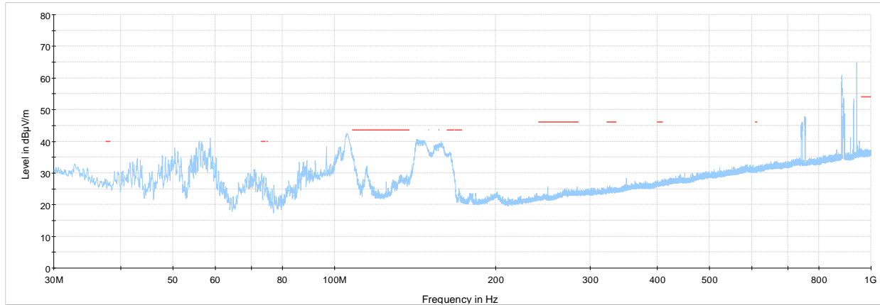
368533 30 MHz - 1 GHz collocation scenario 2
