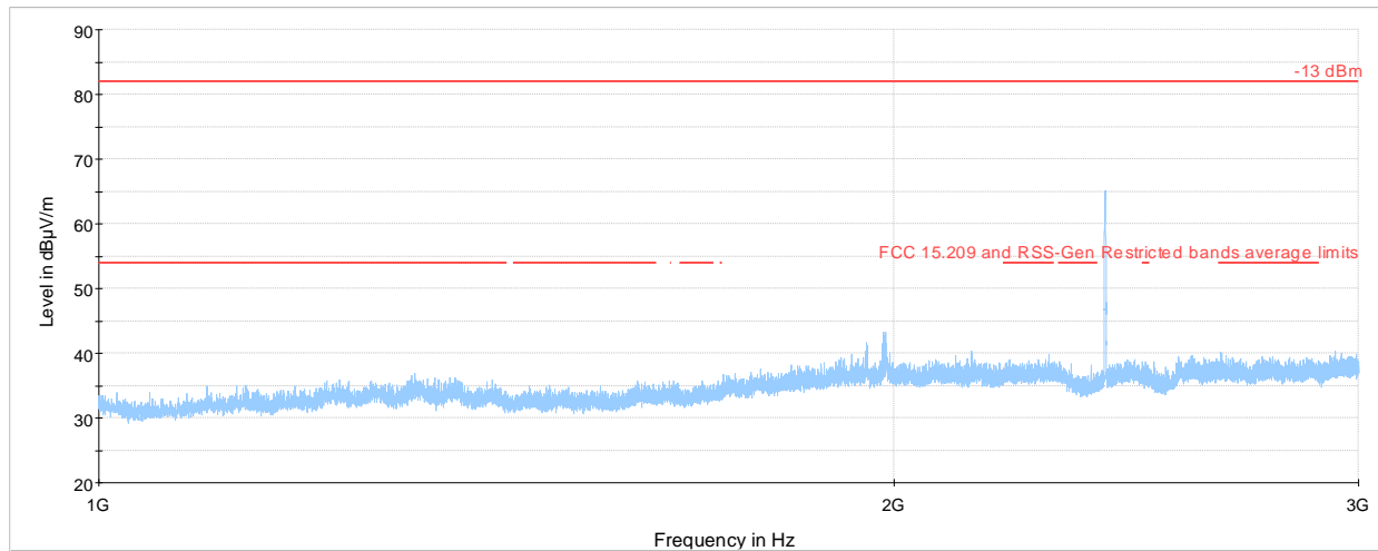
368533 1 - 3 GHz collocation scenario 4 Preview Result 1-PK+ FCC 15.209 and RSS-Gen Restricted bands average limits -13 dBm
