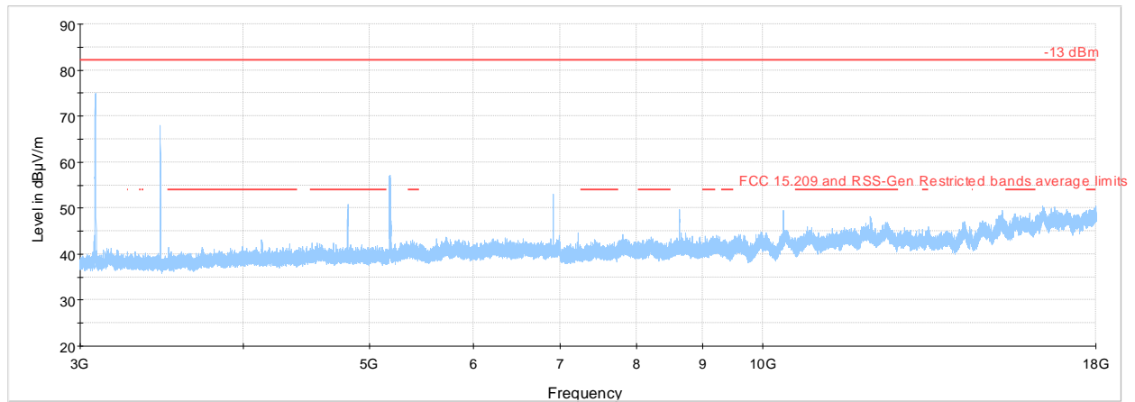
368533 3 - 18 GHz collocation scenario 1 Preview Result 1-PK+ -13 dBm FCC 15.209 and RSS-Gen Restricted bands average limits
