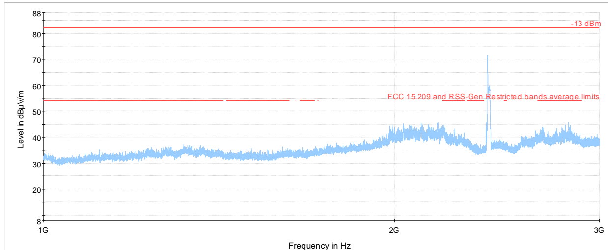
368533 1 - 3 GHz collocation scenario 3 Preview Result 1-PK+ FCC 15.209 and RSS-Gen Restricted bands average limits -13 dBm
