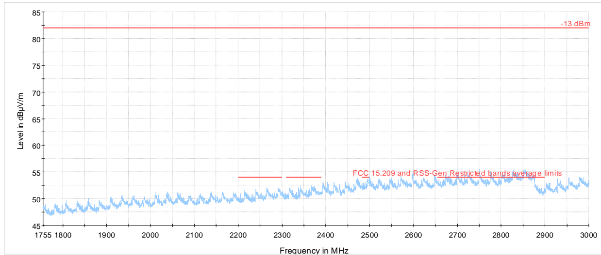
368533 1.755 -3 GHz collocation scenario 1 Preview Result 1-PK+ FCC 15.209 and RSS-Gen Restricted bands average limits -13 dBm
