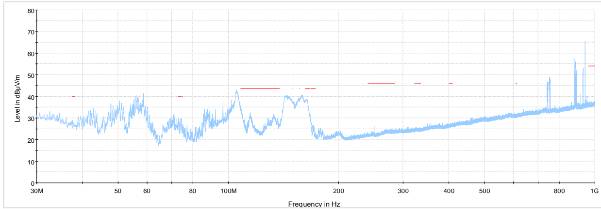
368533 30 MHz - 1 GHz collocation scenario 4 Preview Result 1-PK+ FCC 15.209 and RSS-Gen Restricted bands average limits
