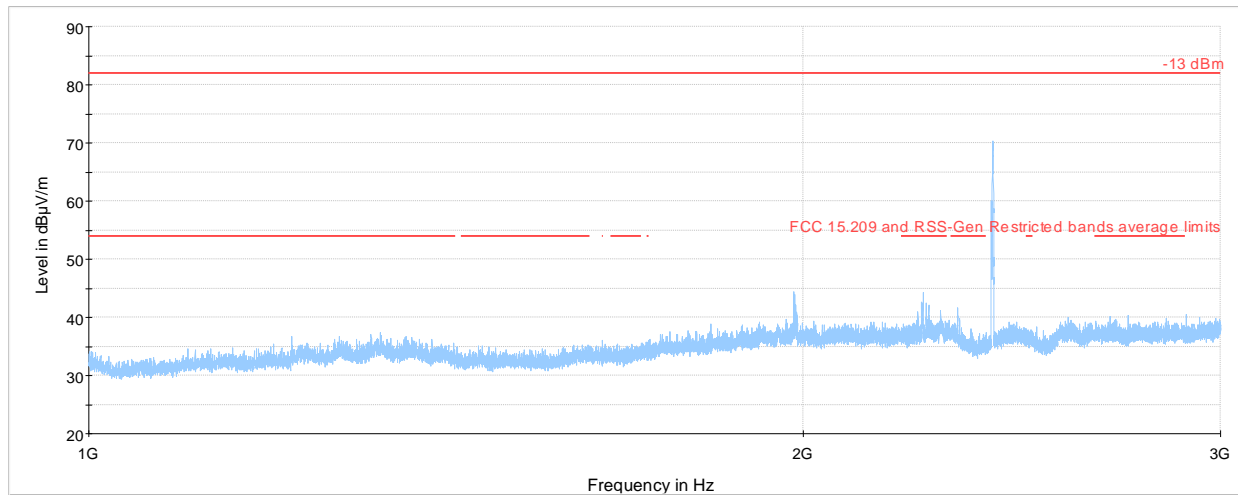
368533 1 - 3 GHz collocation scenario 2
