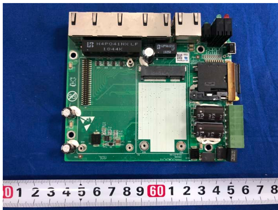
Main Board without RF module Top View
