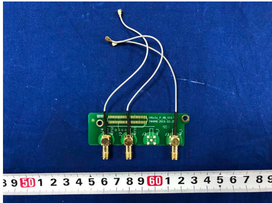
Antenna Connector Board Top View
