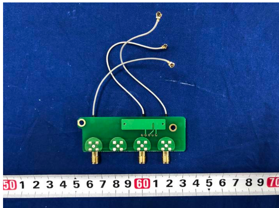
Antenna Connector Board Bottom View
