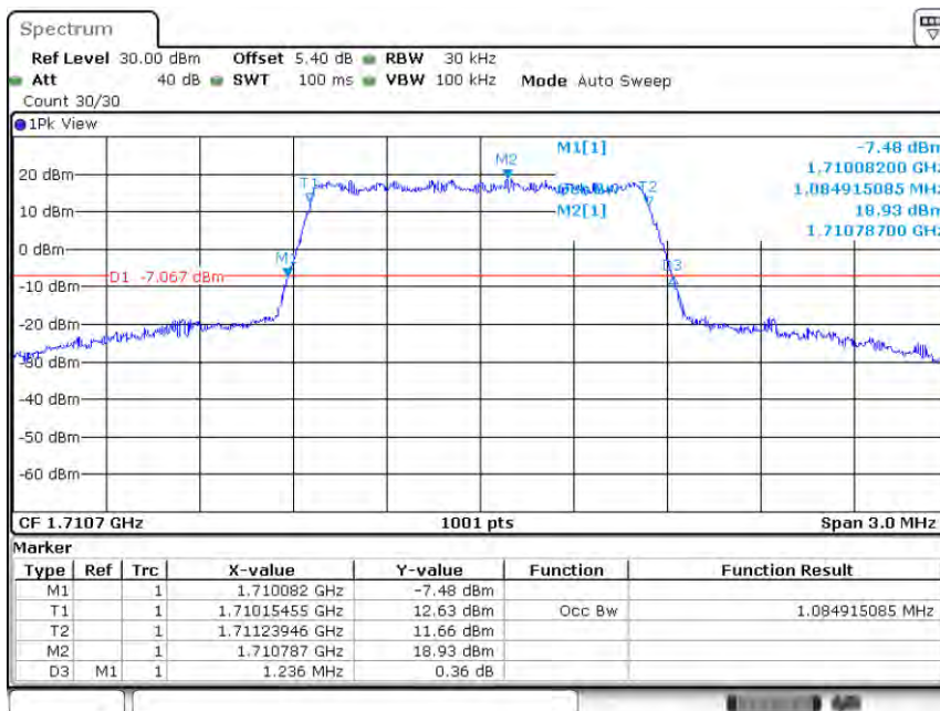
Band4-1.4MHz-QPSK-19957-6RB#0-1.085
