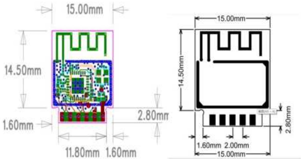
Figure 4 Module Dimensions
