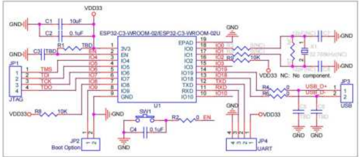
Figure 7 Application Circuit
