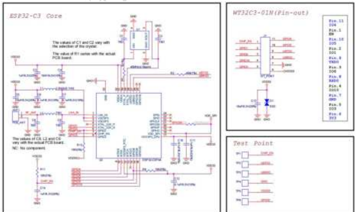
Figure 6 Module Schematics
