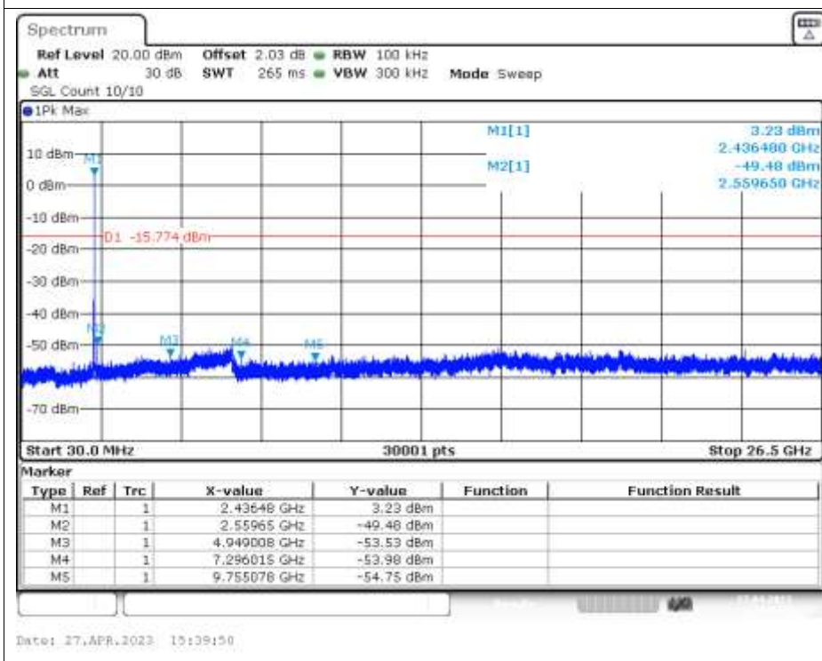
Tx. Spurious NVNT b 2437MHz Ant1 Emission
