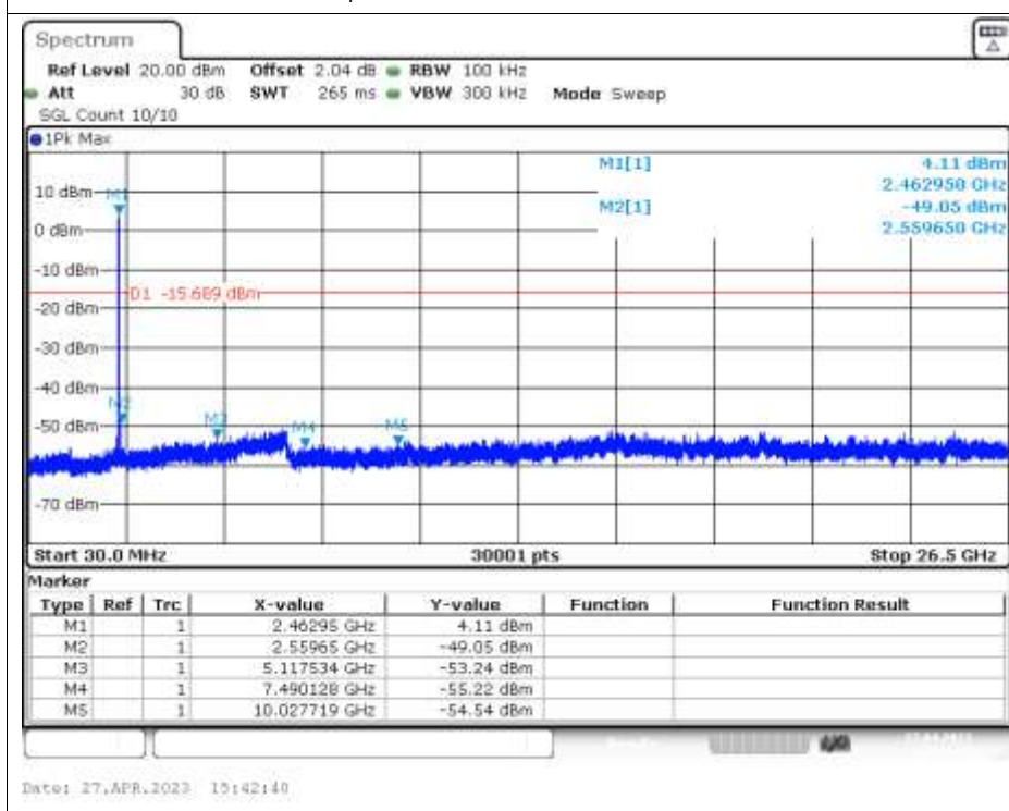
Tx. Spurious NVNT b 2462MHz Ant1 Emission
