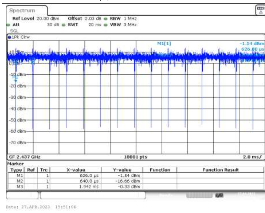
Duty Cycle NVNT n20 2437MHz Ant1
