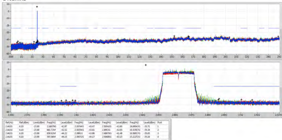
802.11ax HEW20_Nss1,(MCS0)_4TX 2462MHz
