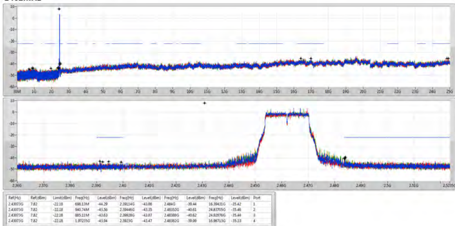
802.11g_Nss1,(6Mbps)_4TX 2462MHz
