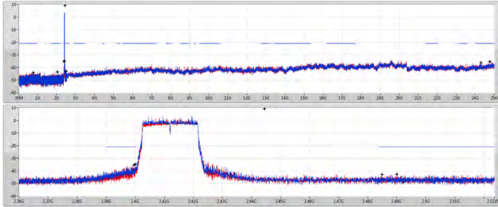
802.11ax HEW20_Nss2,(MCS0)_2TX
