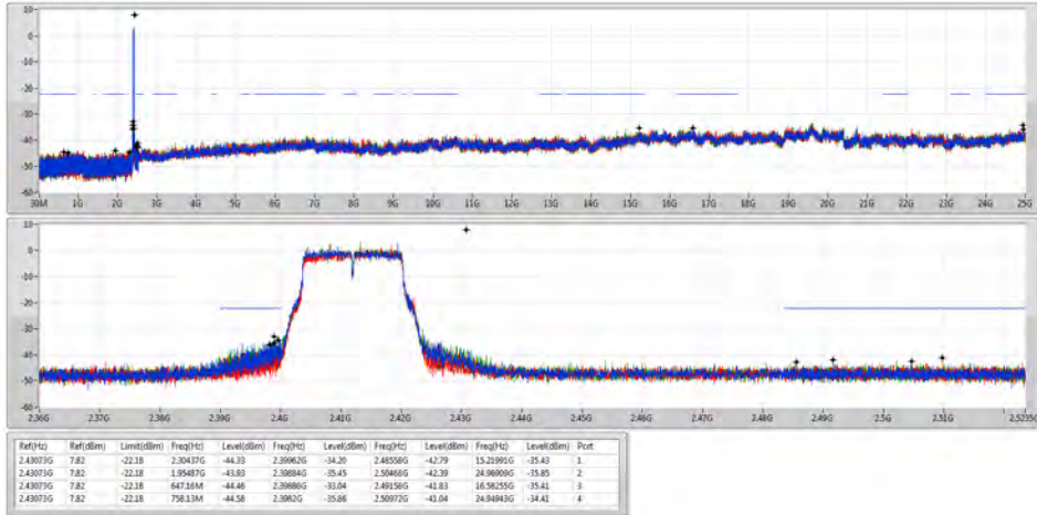
802.11g_Nss1,(6Mbps)_4TX 2412MHz
