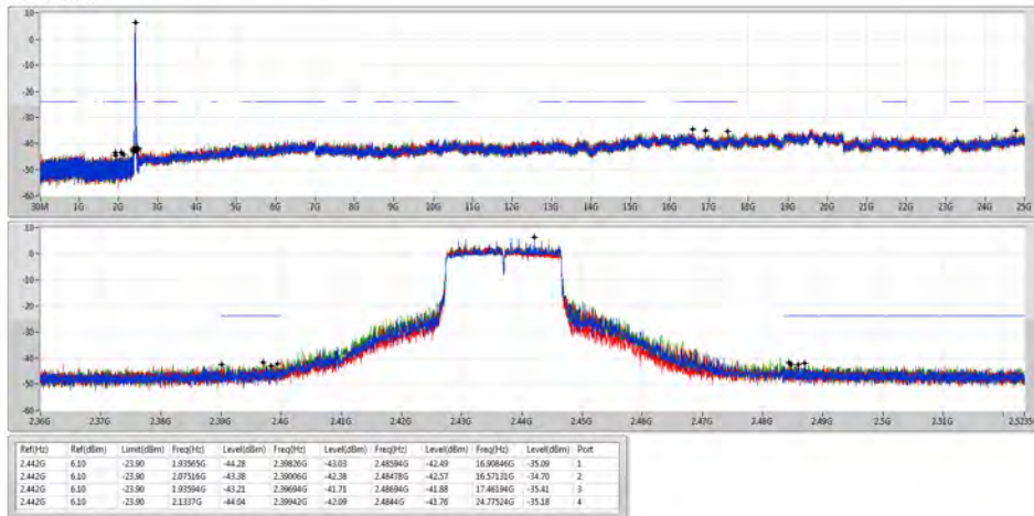
802.11ax HEW20_Nss1,(MCS0)_4TX 2437MHz
