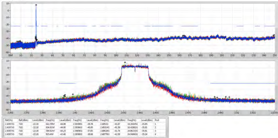
802.11g_Nss1,(6Mbps)_4TX 2437MHz
