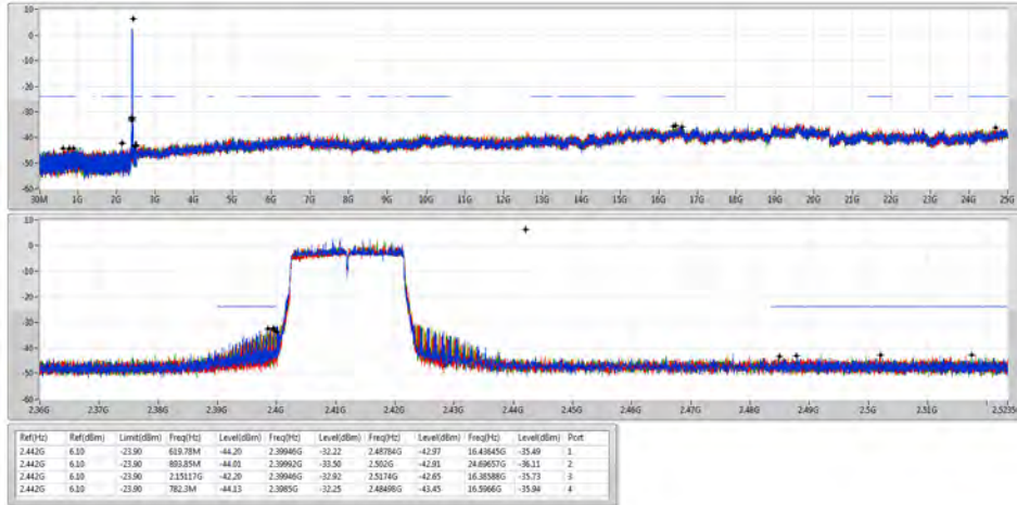
802.11ax HEW20_Nss1,(MCS0)_4TX 2412MHz
