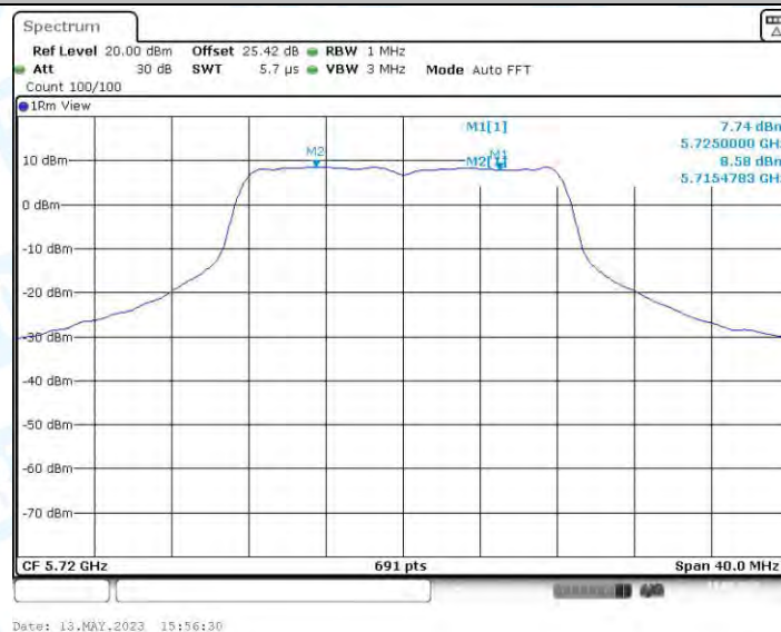
11A_Ant4_5720_UNII-2C
