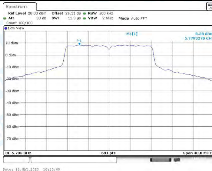
11A_Ant4_5785
