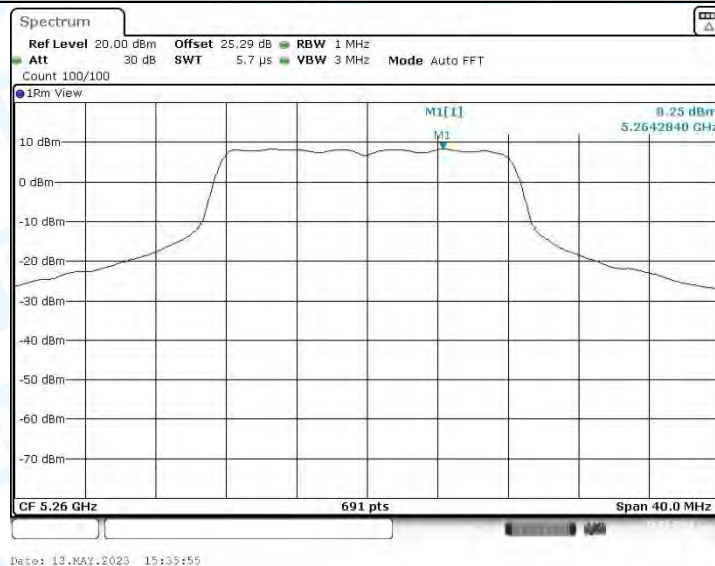
11A_Ant4_5260
