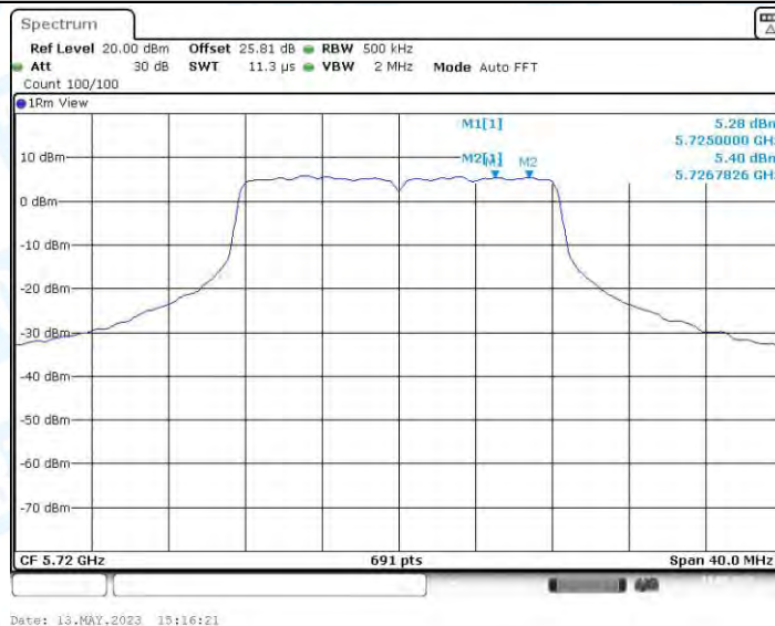
11A_Ant3_5720_UNII-3
