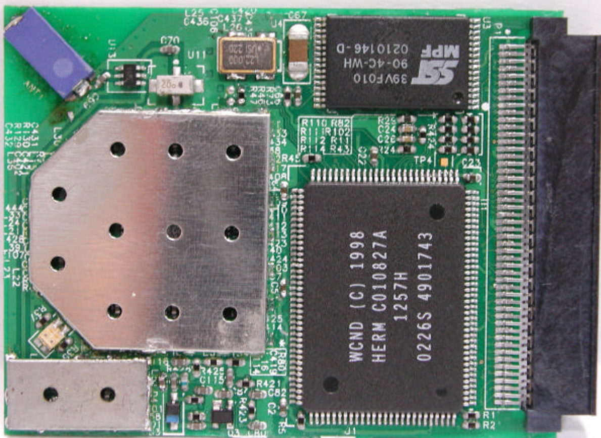
Internal Photo of USI 802.11b CompactFlash Card
