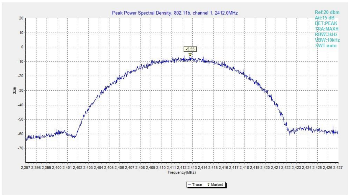
Fig.B.3.1 Power Spectral Density(802.11b,Ch1)
