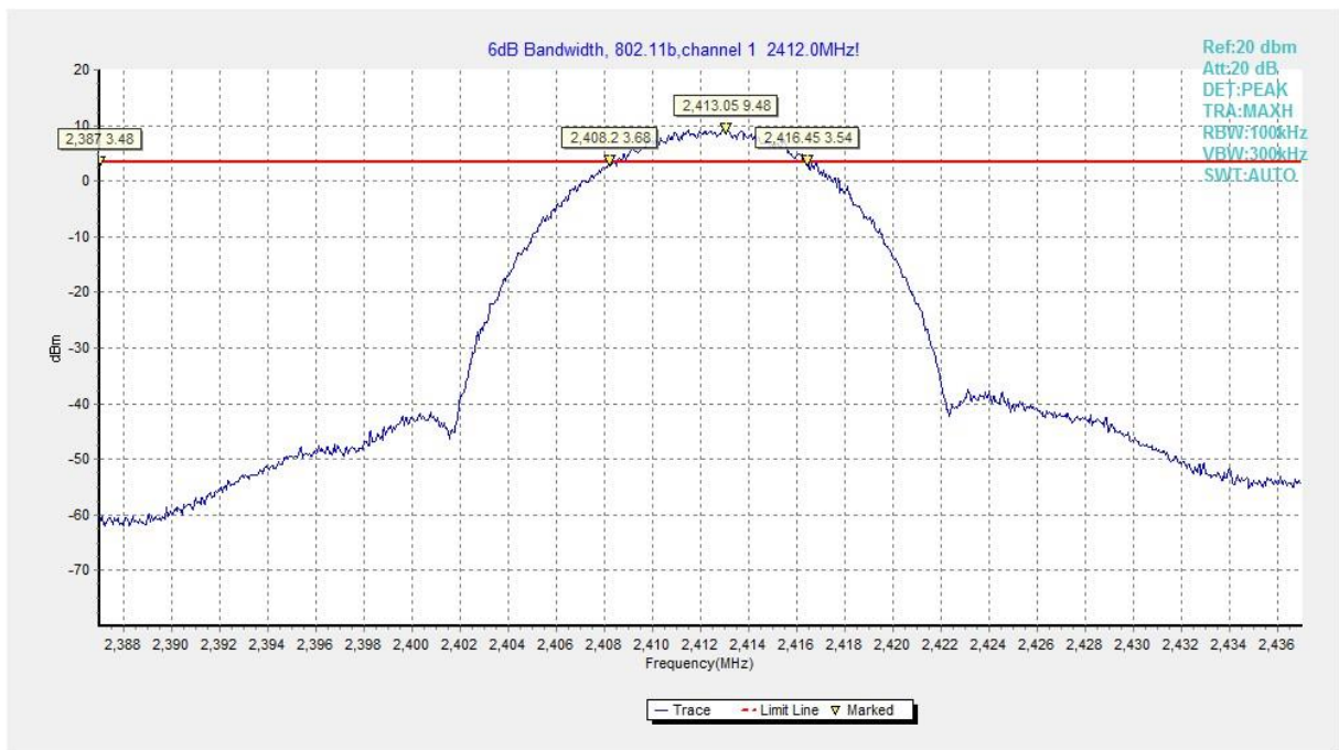
Fig.B.4.1 Occupied 6dB Bandwidth(802.11b,Ch 1)
