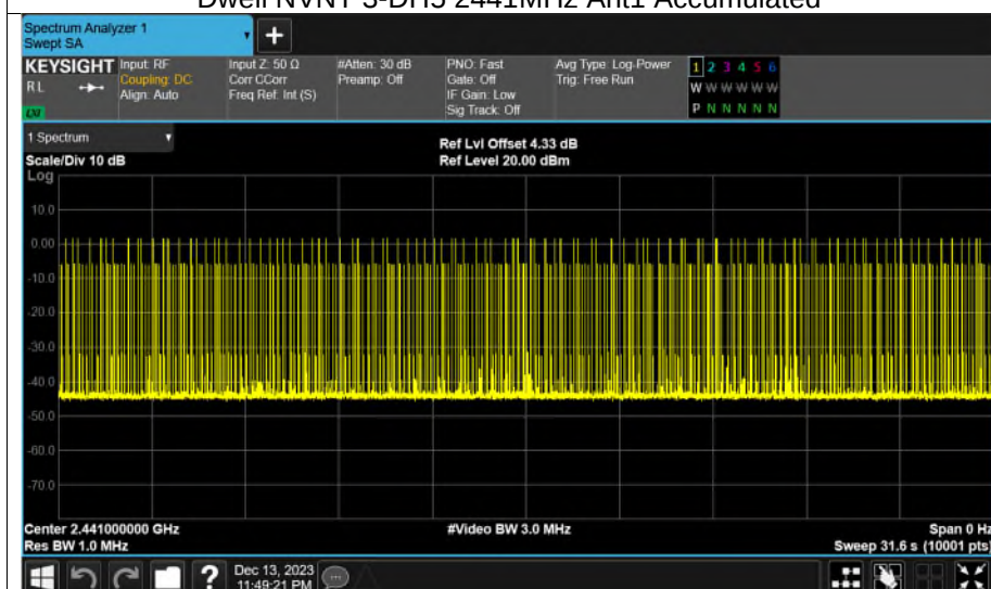
Dwell NVNT 3-DH5 2441MHz Ant1 Accumulated
