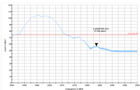
802.11b-Channel 11 Peak
