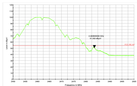
802.11b-Channel 11 Average
