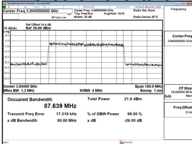
Band77-Part27_90MHz_CP_OFDM_SCS30kHz_16QAM_RB245_0_Chain1_CH656000
