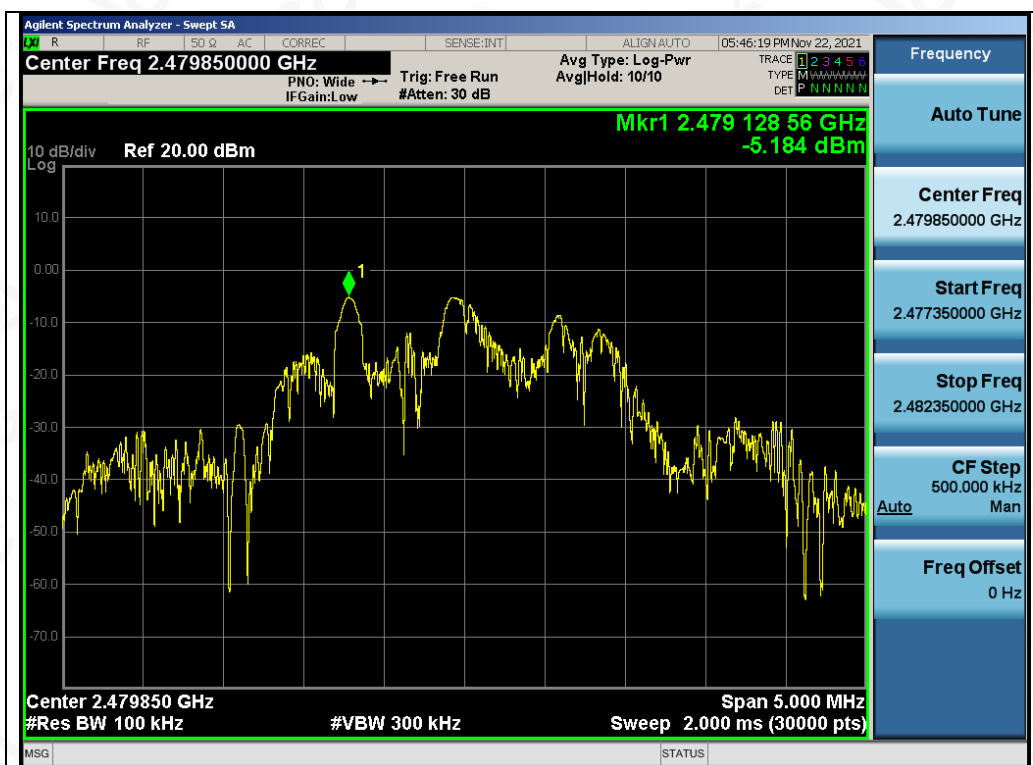
Test_Graph_ANT1_2479.85_Reference Level
