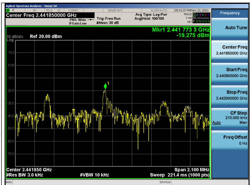
Test_Graph_LE2M_ANT1_2441.85_2Mbps_PSD
