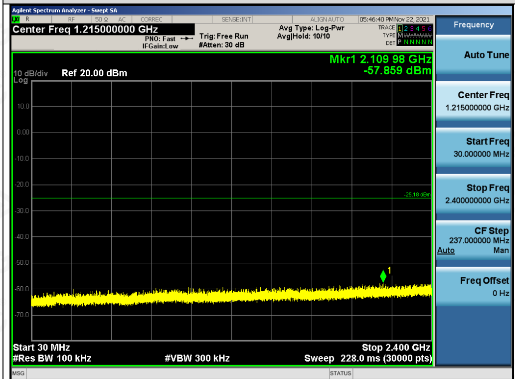
Test_Graph_ANT1_2479.85_Lower Band Emissions
