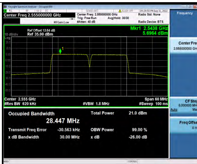
7C-15MHz-15MHz-16QAM-16QAM-LOW-75RB#0-75RB#0
