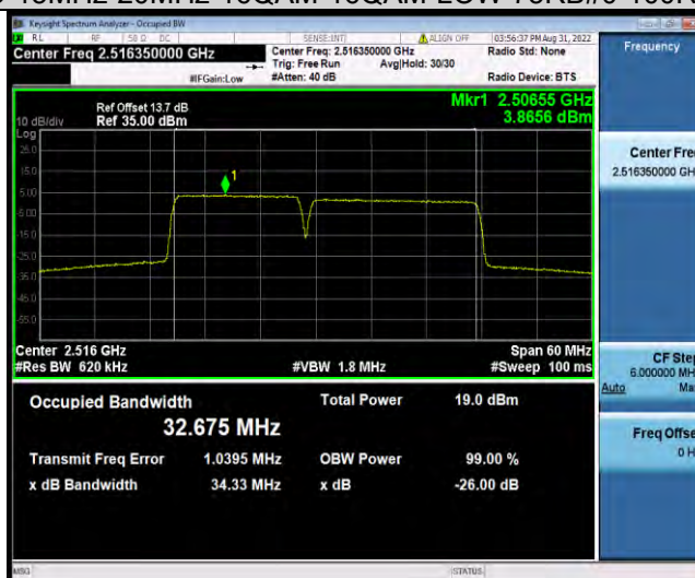
7C-15MHz-20MHz-16QAM-16QAM-MID-75RB#0-100RB#0
