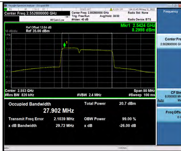
7C-10MHz-20MHz-16QAM-16QAM-LOW-50RB#0-100RB#0
