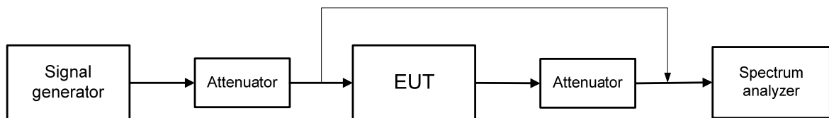
Figure 7.1.1 AGC Threshold level test setup
