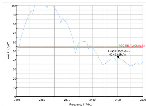
802.11b-Channel 11: Average
