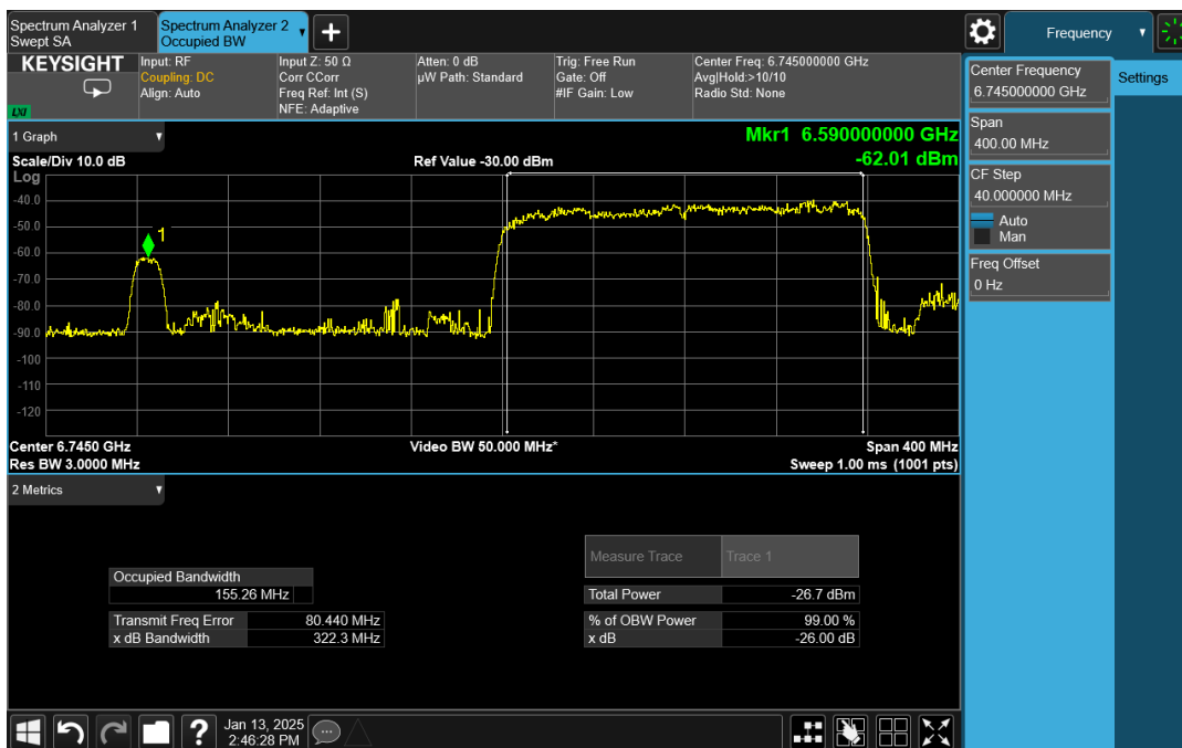
Plot 9: AWGN BW Reduction 320MHz
