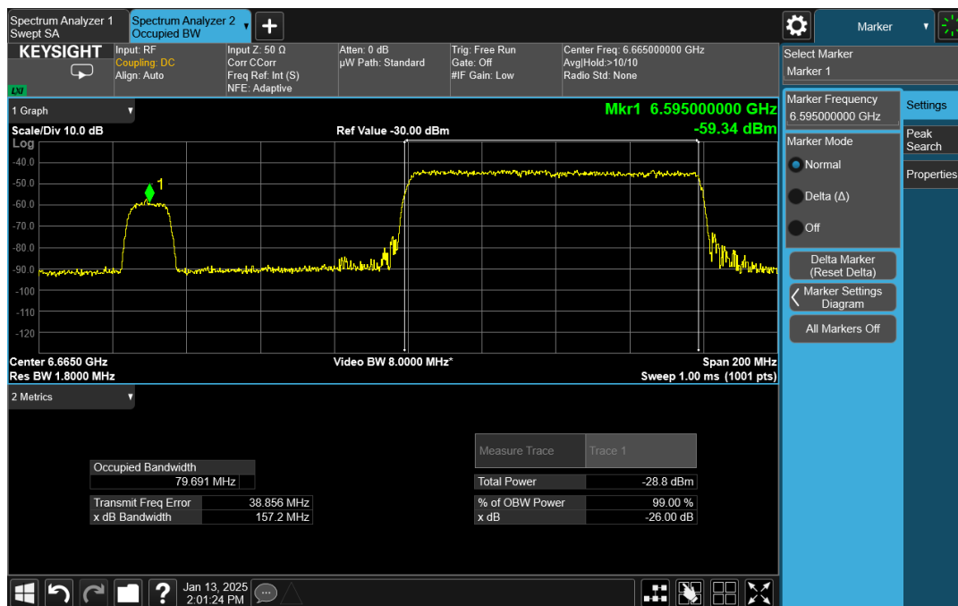
Plot 4: AWGN BW Reduction 160MHz
