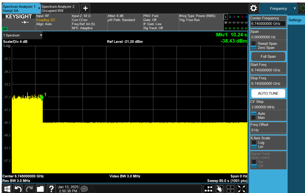
Plot 11: AWGN Signal Detection 320MHz
