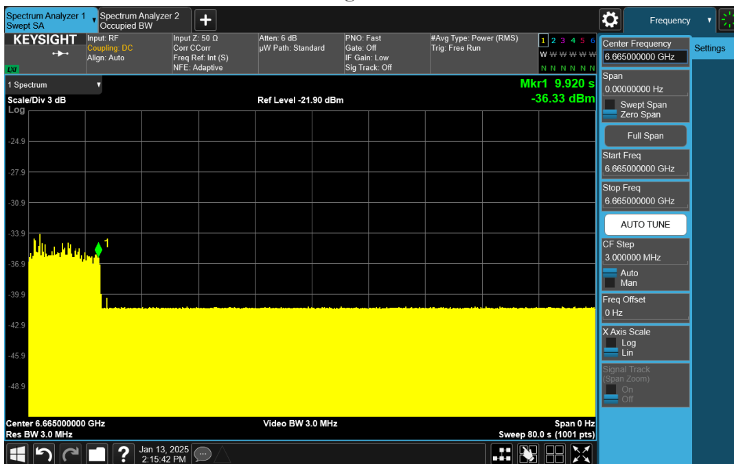
Plot 6: AWGN Signal Detection 160MHz
