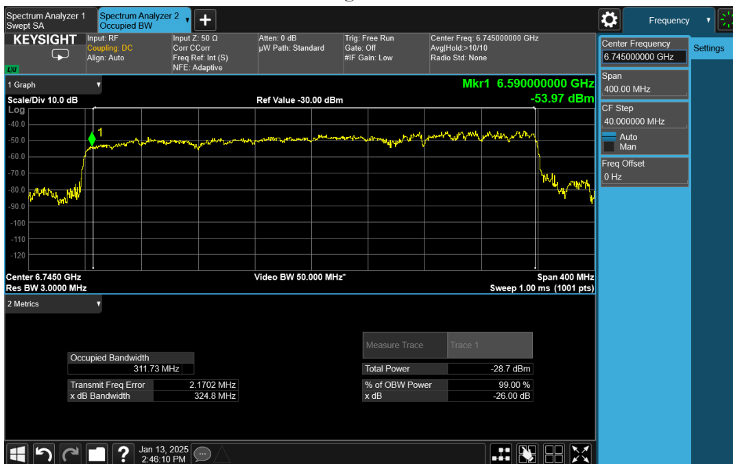
Plot 8: AWGN BW 320MHz
