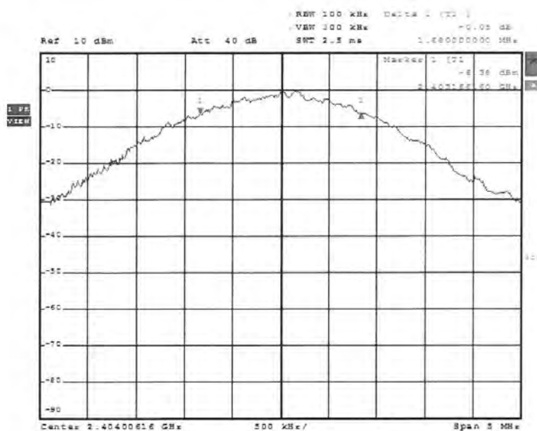
20140609 DST-24T 6dB bandwidth Low frequency
