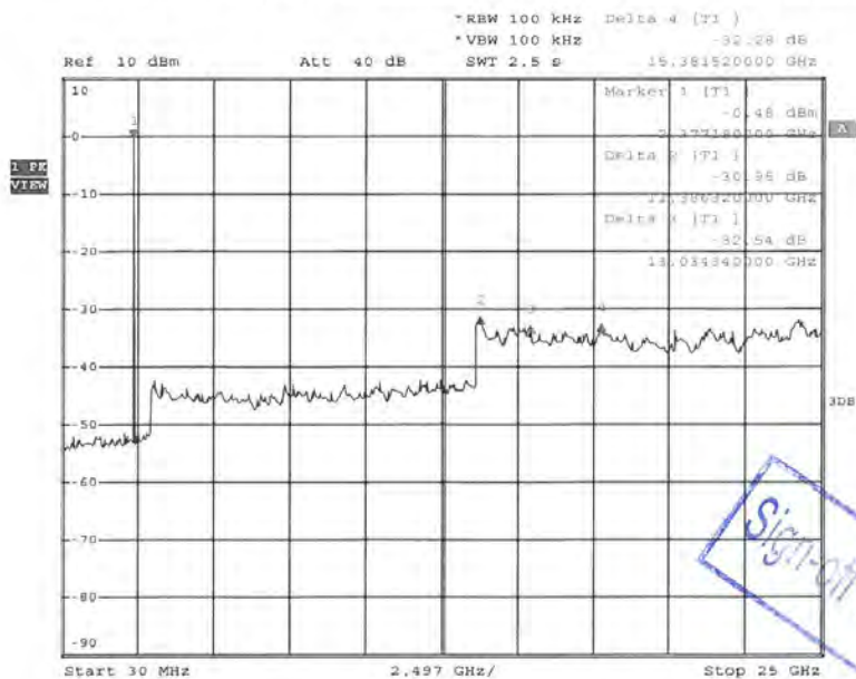
20140609 DST-24T Conducted spurious emission Low frequency
