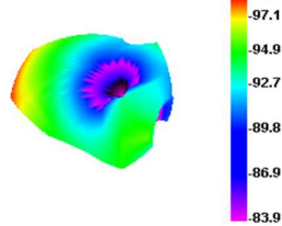
Bluetooth 78 TIS
