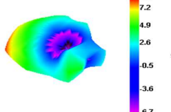
Bluetooth 78 TRP
