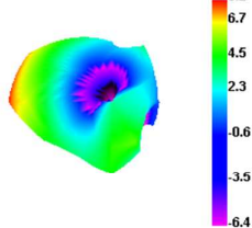
Bluetooth 78 TRP
