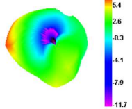
Bluetooth 0 TRP
