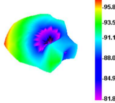
Bluetooth 0 TRP
