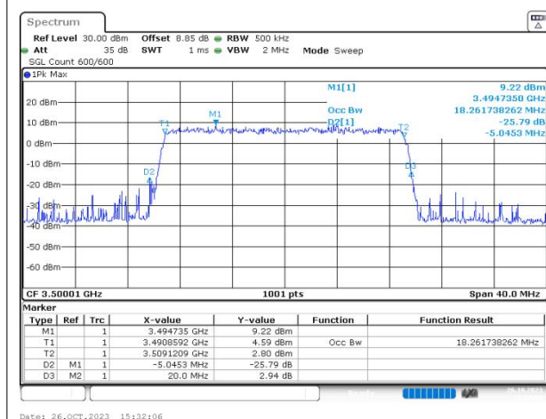
n77(3450-3550) SCS=30kHz CP_QAM256 BW=20MHz Channel=633334 RB=51@0
