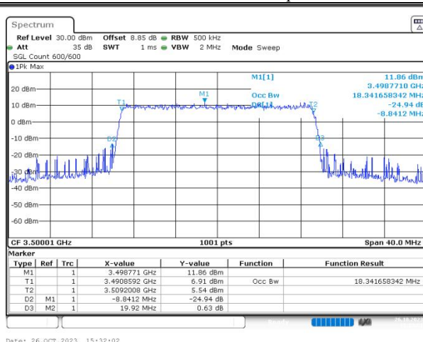
n77(3450-3550) SCS=30kHz CP_QAM64 BW=20MHz Channel=633334 RB=51@0
