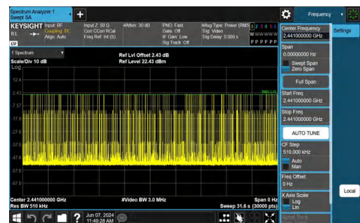
3DH5-Ant1-Hop-PASS
