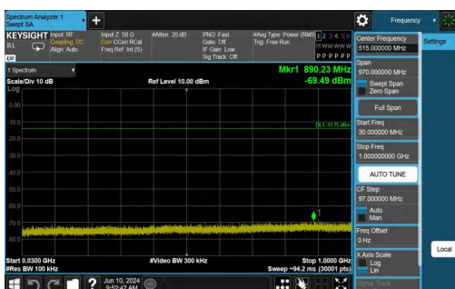
2DH5-Ant1-2480-30~1000-PASS
