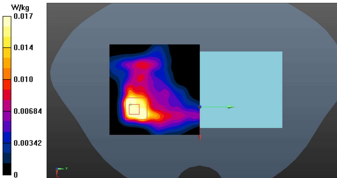
Fig.26 Bluetooth Body
