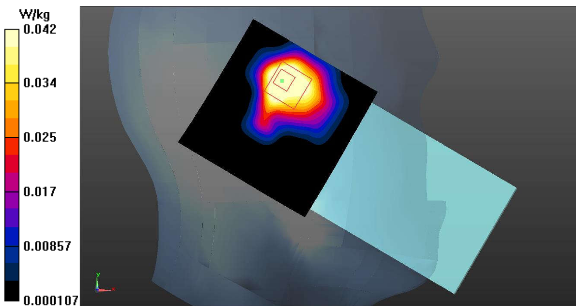
Fig.25 Bluetooth Head
