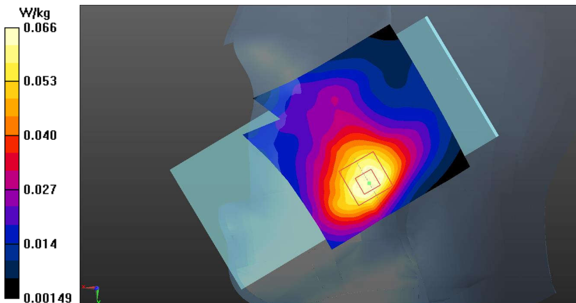
Fig.3 PCS1900 Head
