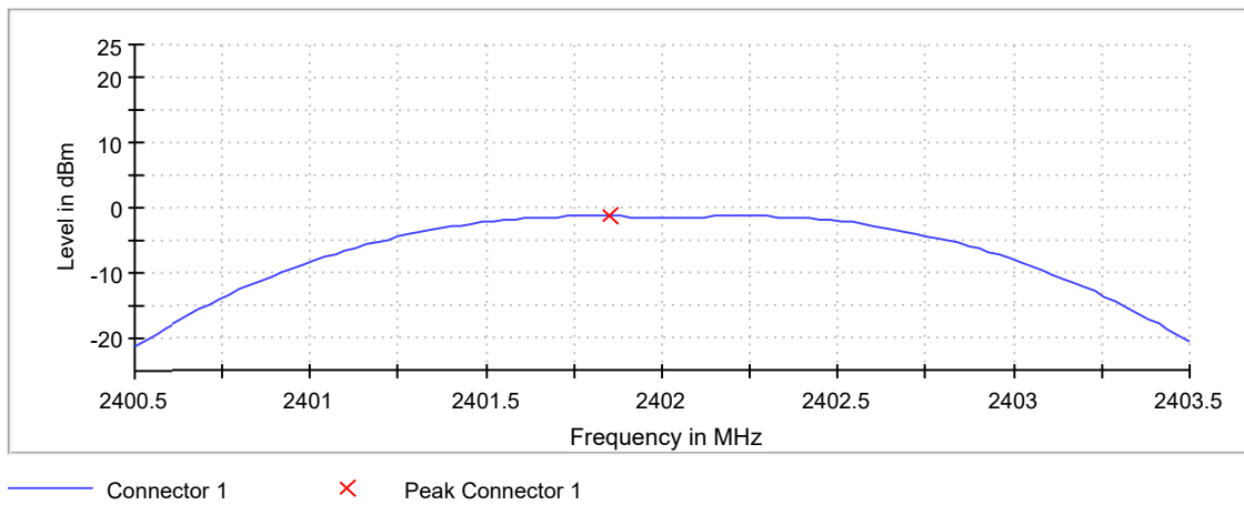
Peak Power
