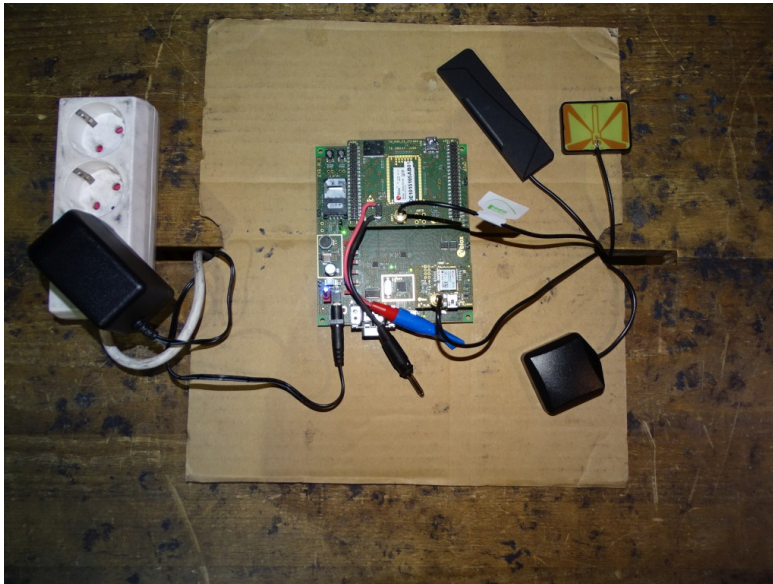
Photo 4: EUT setup
