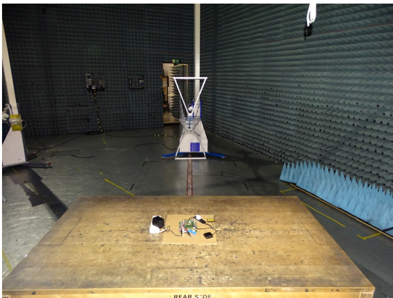
Photo 3: Test setup for radiated measurements above 1GHz
