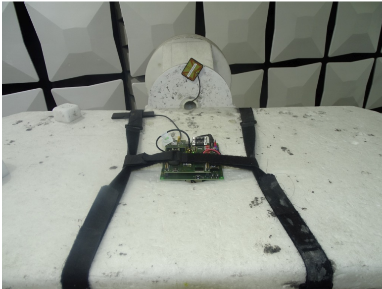
Photo 2: EUT setup
