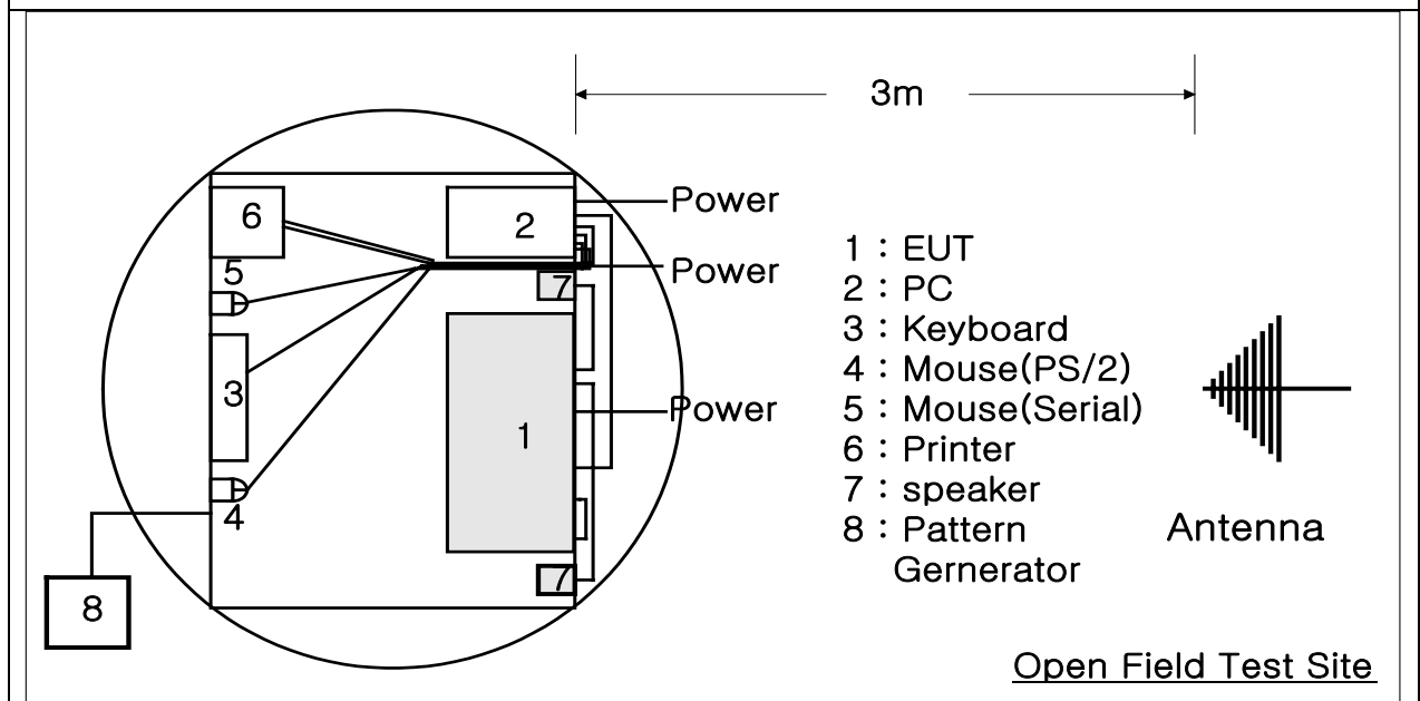
Picture 2 : Radiated emission 30MHz ~ 1000MHz
