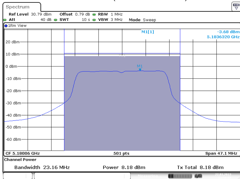
Plot A1 Antenna 1 (add 3dB for max PPST)
