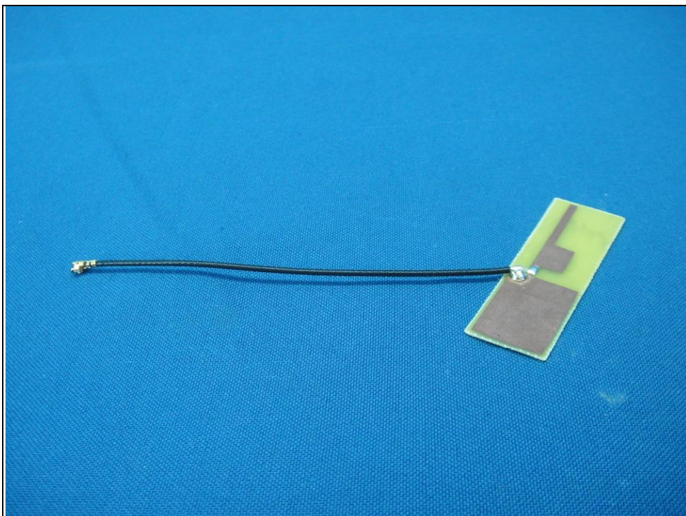
MONOPOLE antenna
