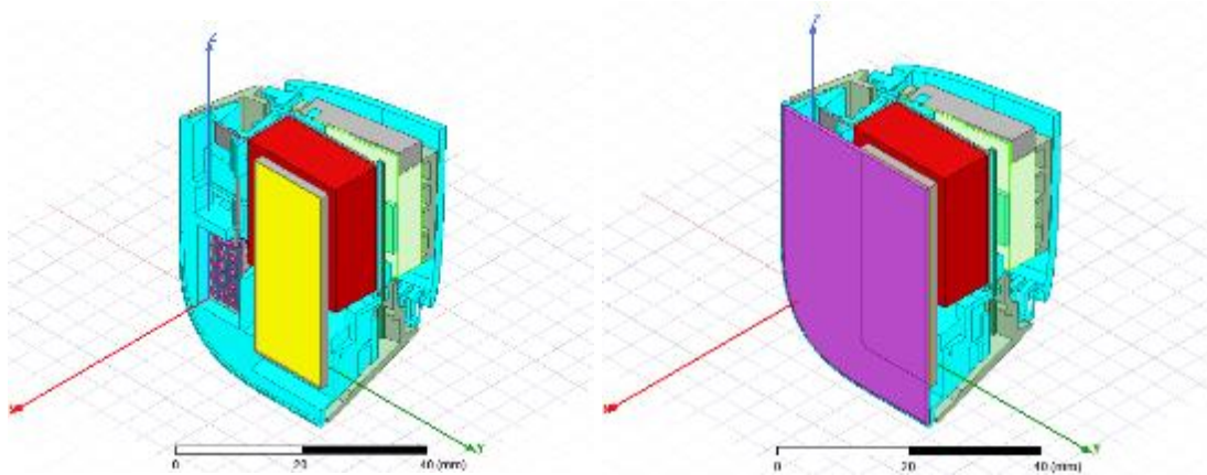
Figure C-5 Right module
