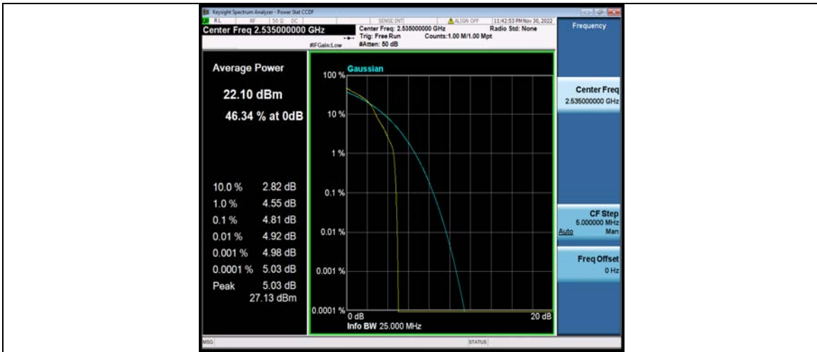
Band7-10MHz-16QAM-21100-50RB#0
