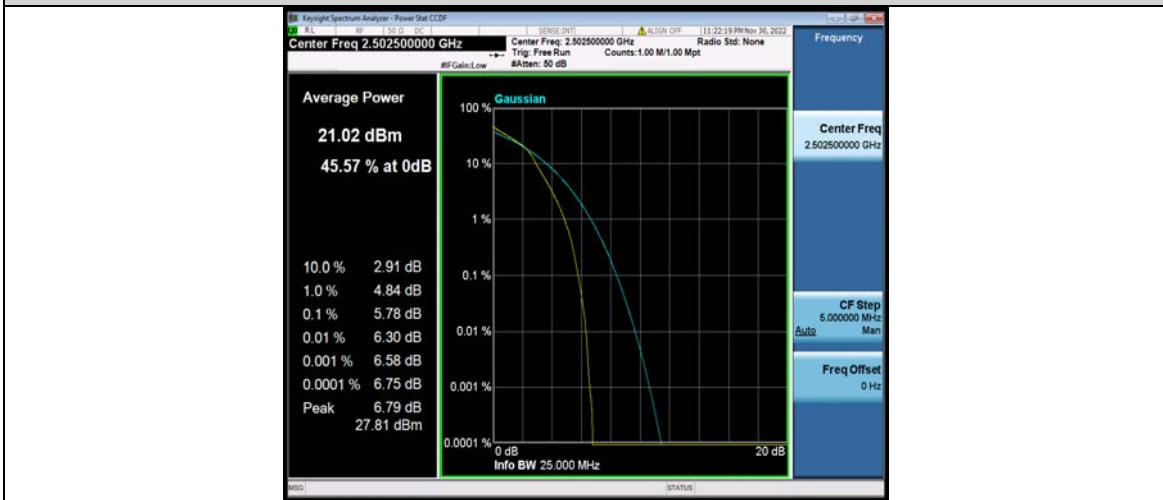
Band7-5MHz-16QAM-21100-1RB#0
