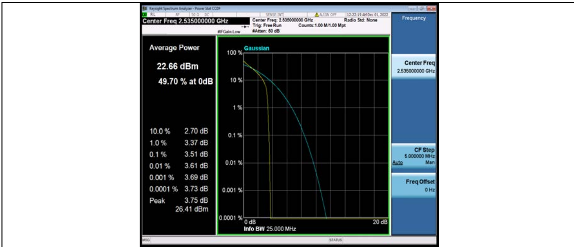
Band7-20MHz-QPSK-21100-100RB#0
