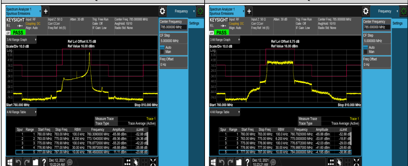
Band13-10MHz-16QAM-23230-1RB#49
