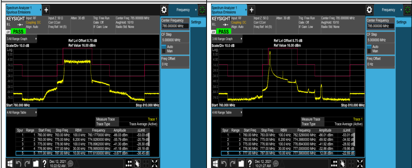
Band13-10MHz-QPSK-23230-50RB#0
