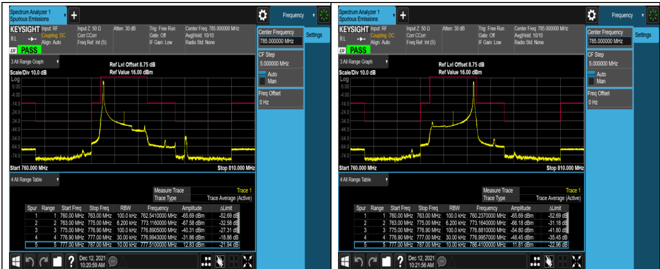
Band13-10MHz-QPSK-23230-1RB#0
