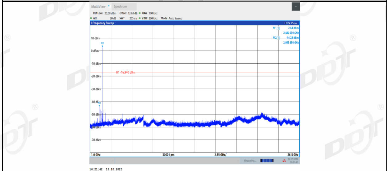
2DH5_Ant1_2402_0~Reference
