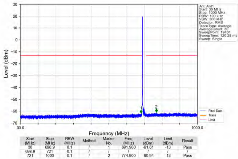
n12_15kHz_SISO_NTNV_15MHz_DFT-s-OFDM_QPSK_706.5MHz_Edge_1RB_Left
