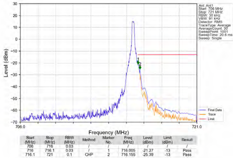
n12_15kHz_SISO_NTNV_10MHz_DFT-s-OFDM_QPSK_711MHz_Edge_1RB_Right
