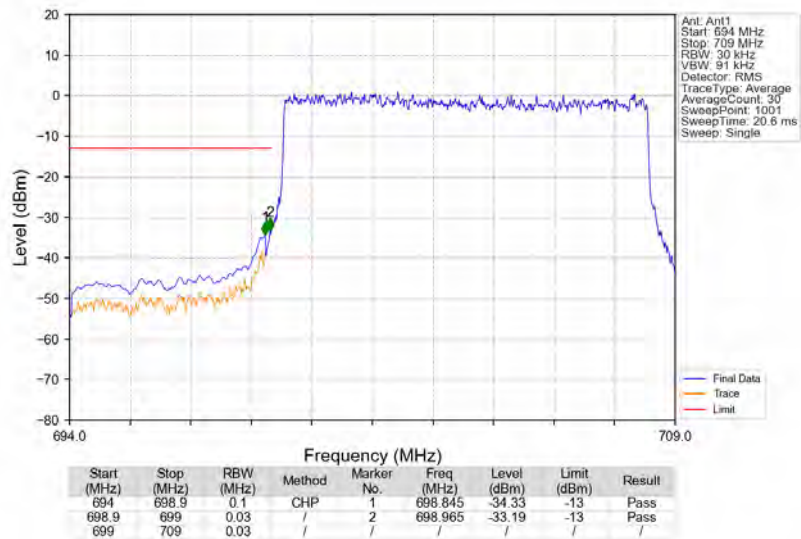
n12_15kHz_SISO_NTNV_10MHz_DFT-s-OFDM_PI/2_BPSK_704MHz_Outer_Full
