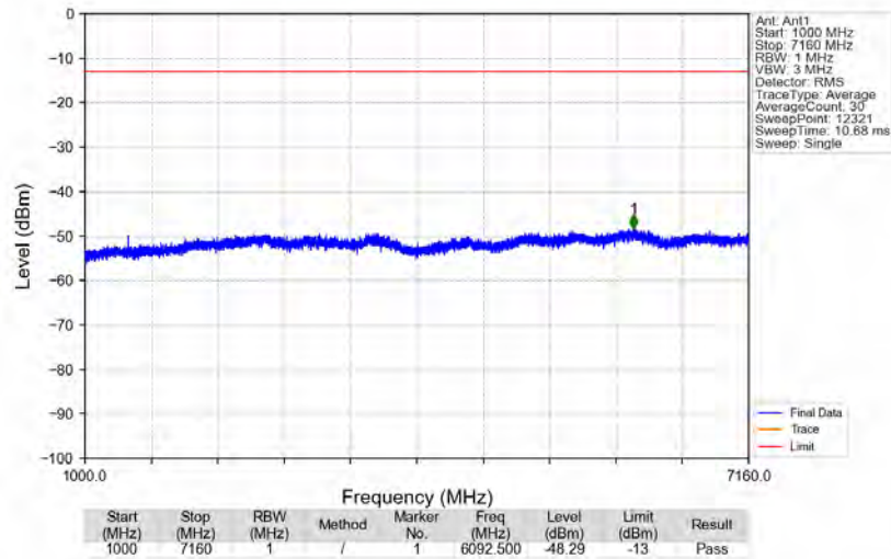
n12_15kHz_SISO_NTNV_15MHz_DFT-s-OFDM_QPSK_707.5MHz_Edge_1RB_Left
