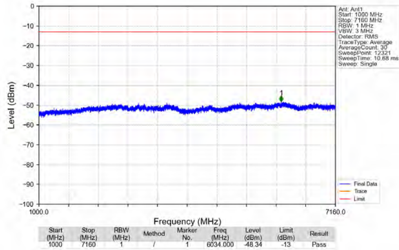
n12_15kHz_SISO_NTNV_15MHz_DFT-s-OFDM_QPSK_708.5MHz_Edge_1RB_Right
