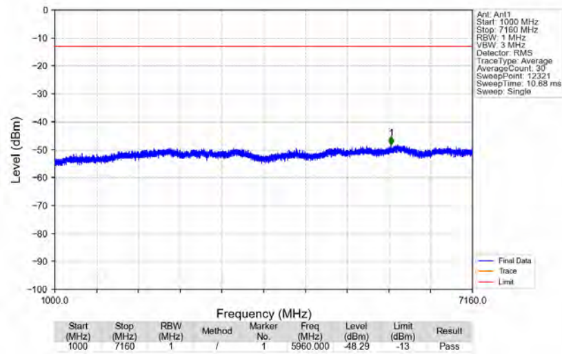
n12_15kHz_SISO_NTNV_10MHz_DFT-s-OFDM_QPSK_704MHz_Edge_1RB_Left
