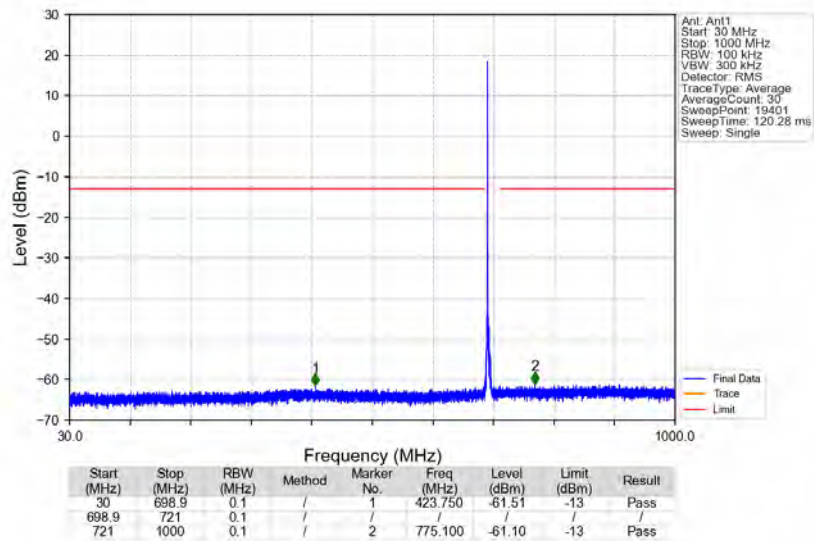
n12_15kHz_SISO_NTNV_5MHz_CP-OFDM_QPSK_701.5MHz_Edge_1RB_Left
