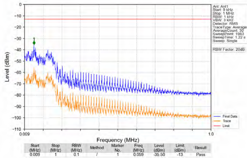
n12_15kHz_SISO_NTNV_15MHz_DFT-s-OFDM_PI/2_BPSK_707.5MHz_Edge_1RB_Left
