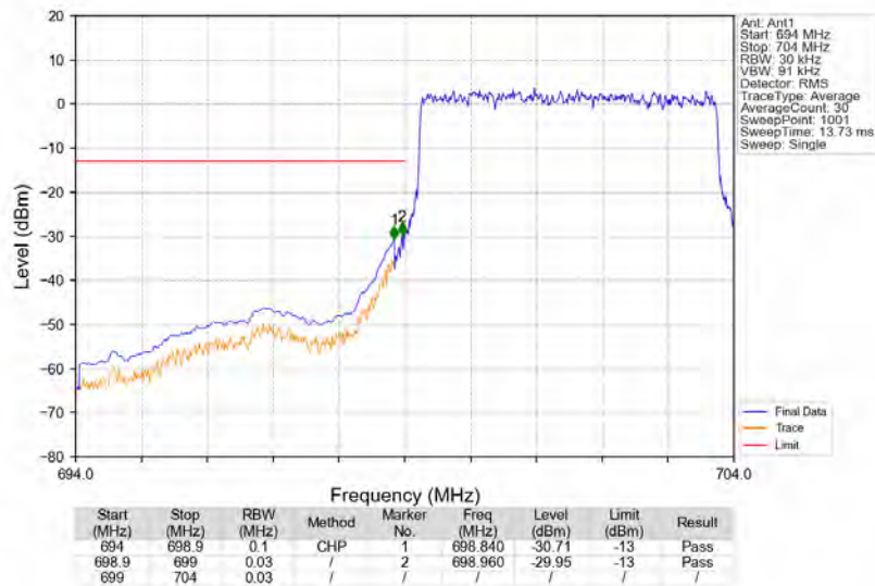
n12_15kHz_SISO_NTNV_5MHz_DFT-s-OFDM_PI/2_BPSK_701.5MHz_Outer_Full
