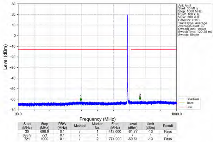
n12_15kHz_SISO_NTNV_15MHz_DFT-s-OFDM_PI/2_BPSK_706.5MHz_Edge_1RB_Left
