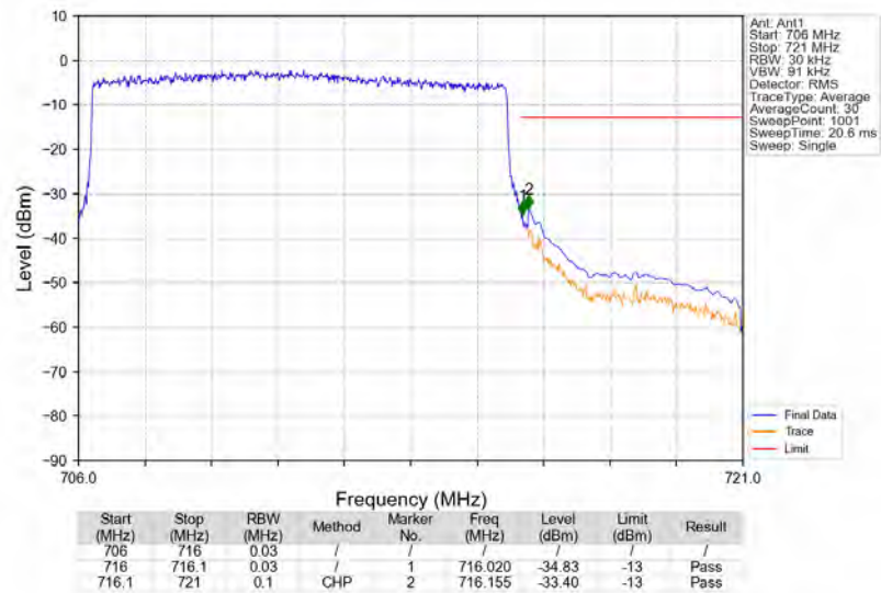
n12_15kHz_SISO_NTNV_10MHz_CP-OFDM_QPSK_711MHz_Outer_Full
