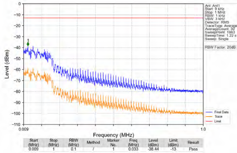
n12_15kHz_SISO_NTNV_10MHz_CP-OFDM_QPSK_707.5MHz_Edge_1RB_Left
