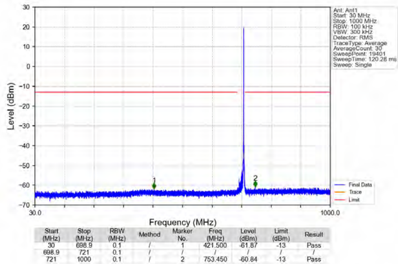
n12_15kHz_SISO_NTNV_15MHz_DFT-s-OFDM_QPSK_708.5MHz_Edge_1RB_Right
