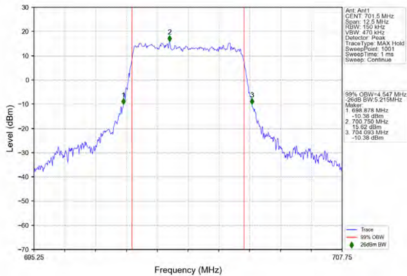
n12_15kHz_SISO_NTNV_5MHz_CP-OFDM 64 QAM 701.5MHz_Outer_Full
