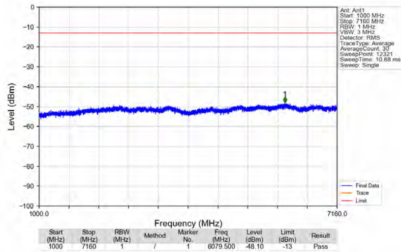
n12_15kHz_SISO_NTNV_5MHz_CP-OFDM_QPSK_713.5MHz_Edge_1RB_Right
