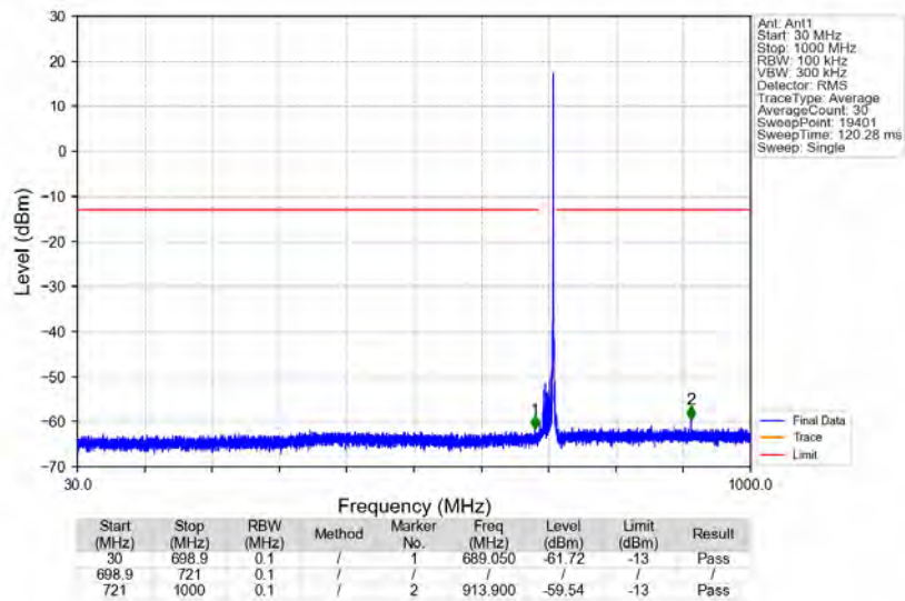
n12_15kHz_SISO_NTNV_15MHz_CP-OFDM_QPSK_708.5MHz_Edge_1RB_Right
