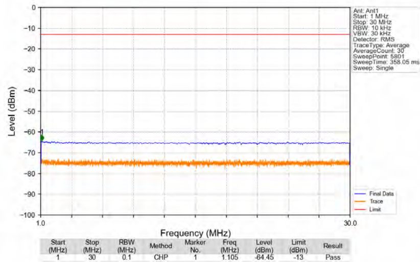
n12_15kHz_SISO_NTNV_10MHz_DFT-s-OFDM_QPSK_707.5MHz_Edge_1RB_Left
