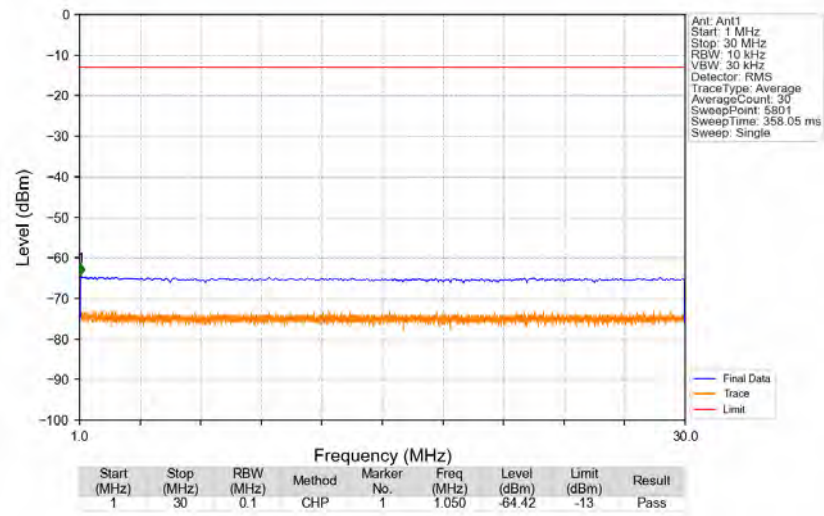
n12_15kHz_SISO_NTNV_15MHz_DFT-s-OFDM_QPSK_708.5MHz_Edge_1RB_Right
