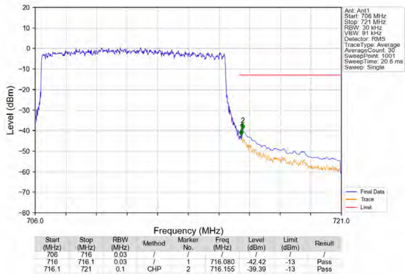
n12_15kHz_SISO_NTNV_10MHz_DFT-s-OFDM_QPSK_711MHz_Outer_Full
