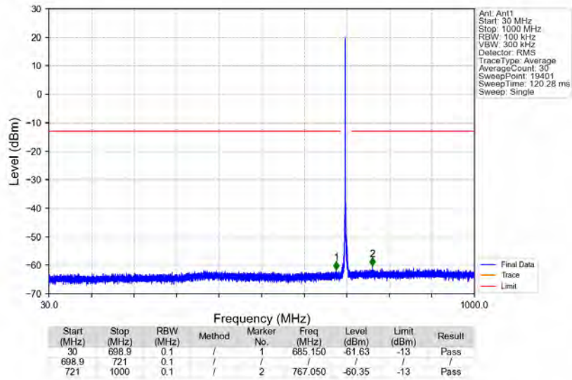
n12_15kHz_SISO_NTNV_5MHz_DFT-s-OFDM_QPSK_707.5MHz_Edge_1RB_Left
