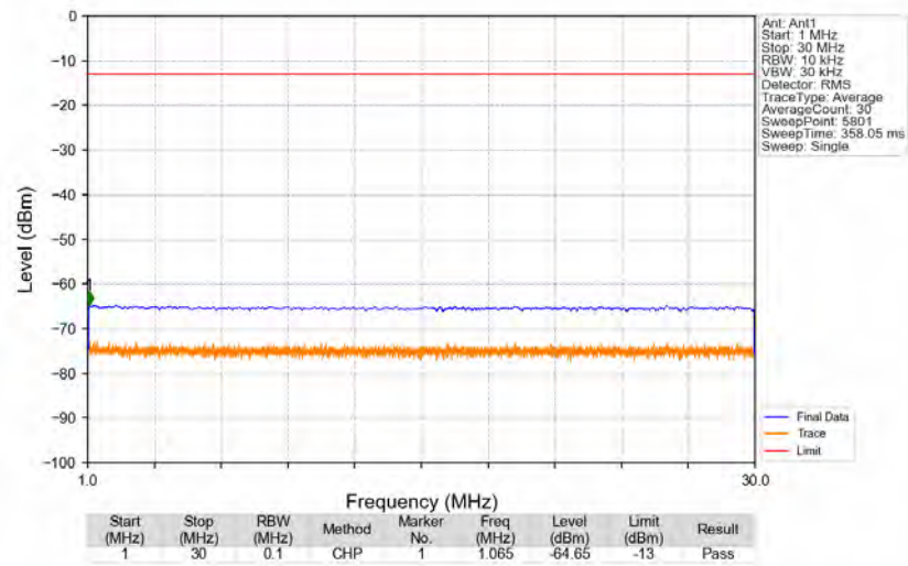
n12_15kHz_SISO_NTNV_10MHz_CP-OFDM_QPSK_704MHz_Edge_1RB_Left
