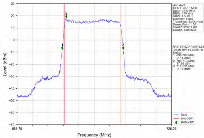
n12_15kHz_SISO_NTNV_15MHz_DFT-s-OFDM_16_QAM_707.5MHz_Outer_Full
