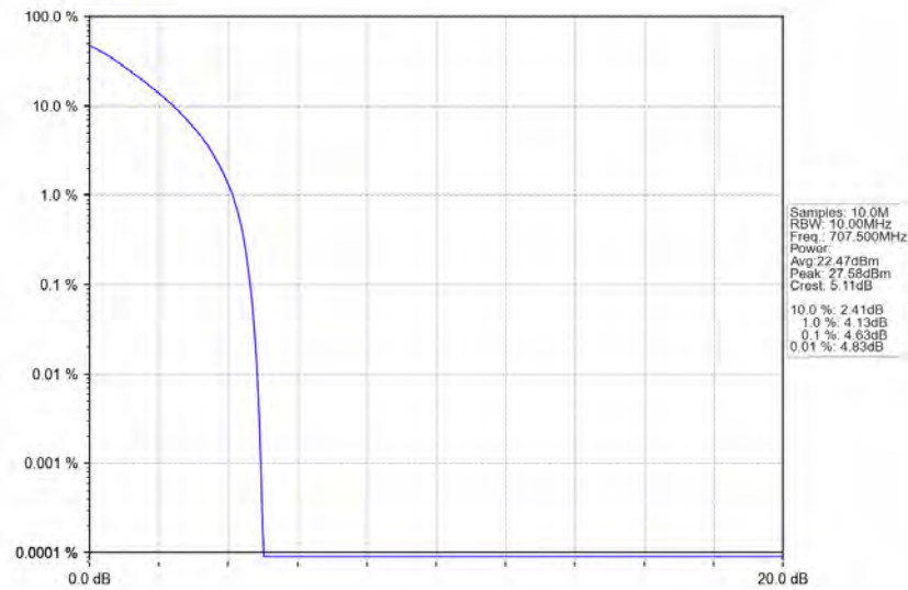
n12_15kHz_SISO_NTNV_10MHz_DFT-s-OFDM_QPSK_707.5MHz_Outer_Full
