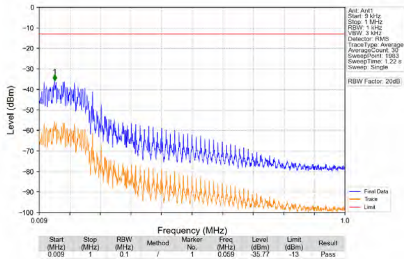
n12_15kHz_SISO_NTNV_10MHz_DFT-s-OFDM_QPSK_711MHz_Edge_1RB_Right
