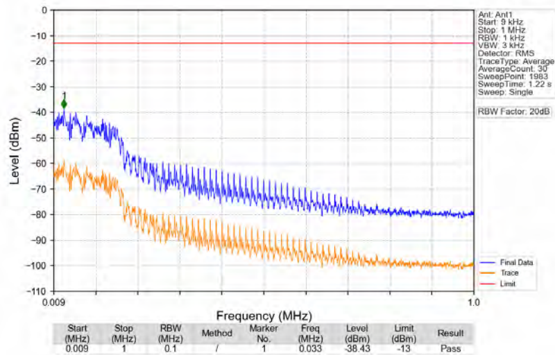
n12_15kHz_SISO_NTNV_10MHz_CP-OFDM_QPSK_704MHz_Edge_1RB_Left
