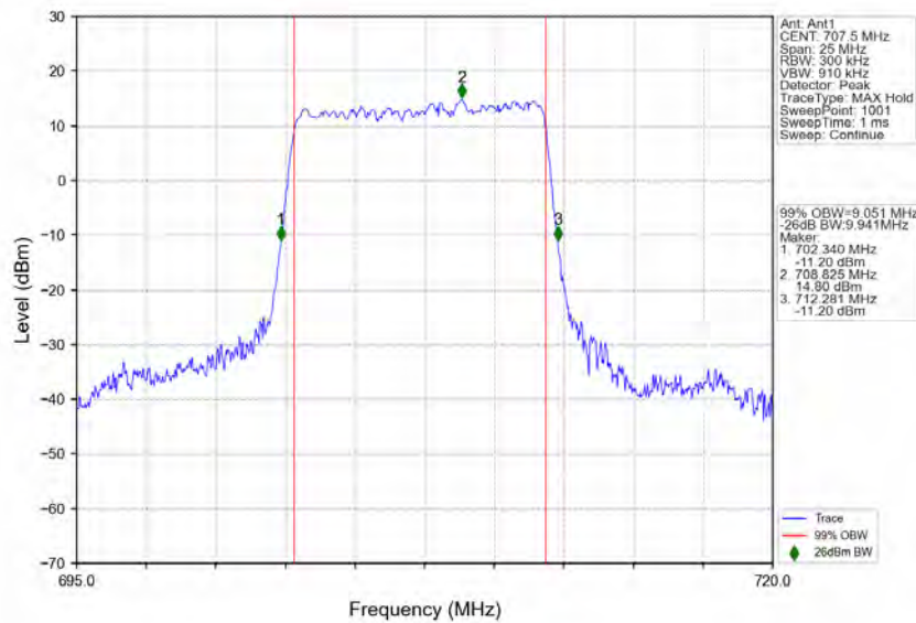
n12_15kHz_SISO_NTNV_10MHz_DFT-s-OFDM_256_QAM_707.5MHz_Outer_Full
