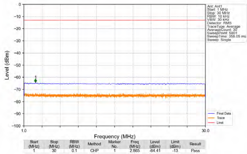
n12_15kHz_SISO_NTNV_15MHz_DFT-s-OFDM_PI/2_BPSK_706.5MHz_Edge_1RB_Left
