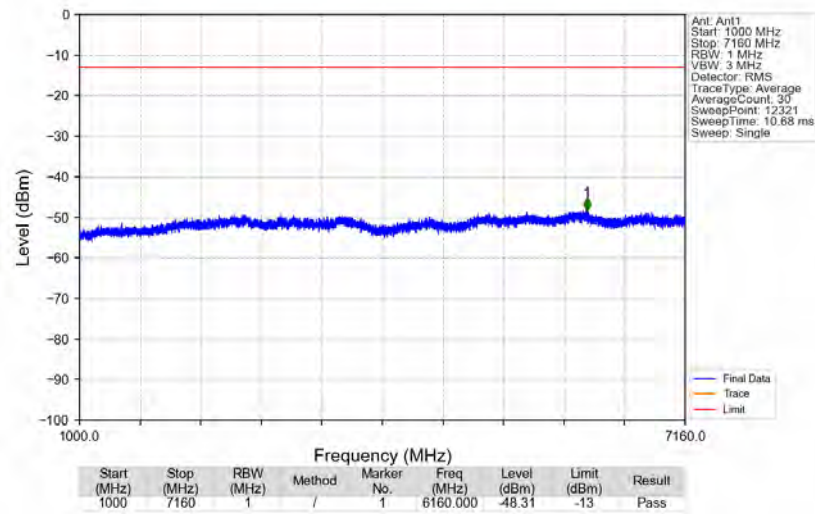
n12_15kHz_SISO_NTNV_15MHz_DFT-s-OFDM_PI/2_BPSK_708.5MHz_Edge_1RB_Right
