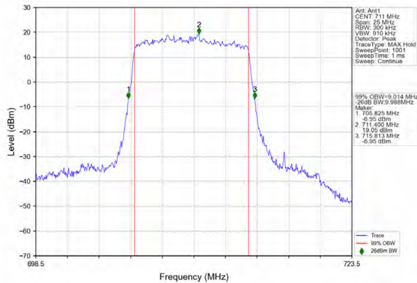
n12_15kHz_SISO_NTNV_10MHz_DFT-s-OFDM_QPSK_711MHz_Outer_Full
