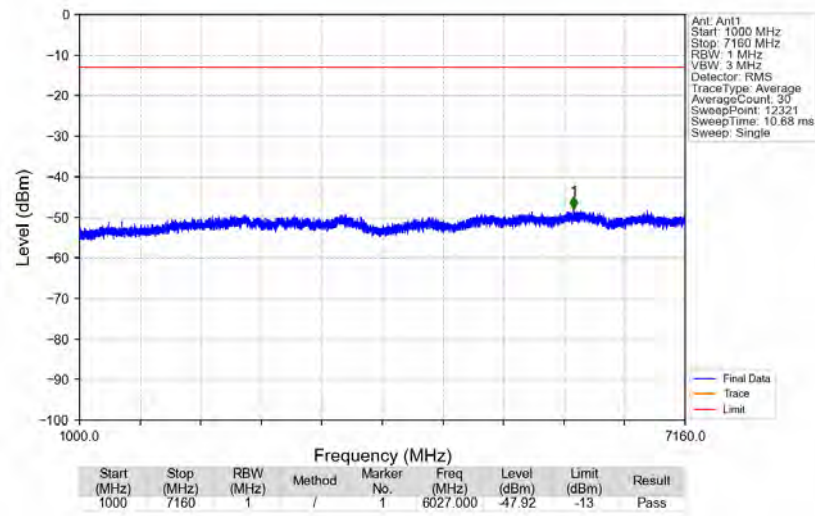
n12_15kHz_SISO_NTNV_10MHz_DFT-s-OFDM_QPSK_711MHz_Edge_1RB_Right
