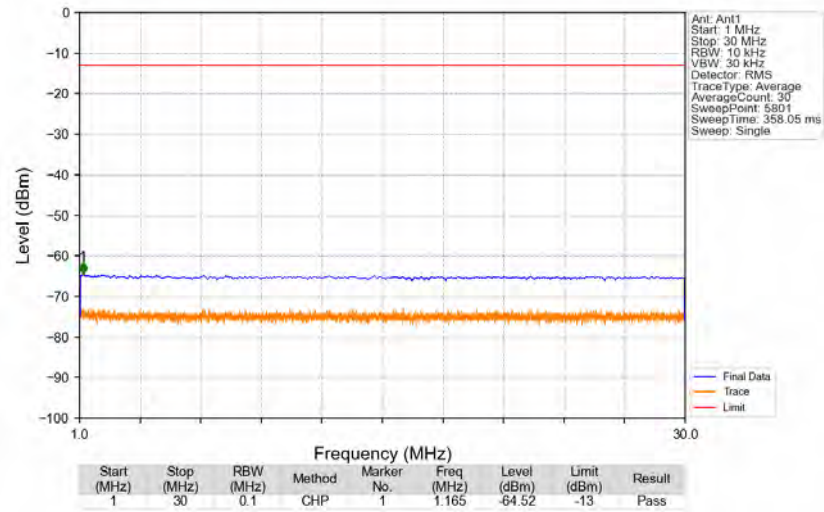
n12_15kHz_SISO_NTNV_15MHz_DFT-s-OFDM_QPSK_706.5MHz_Edge_1RB_Left
