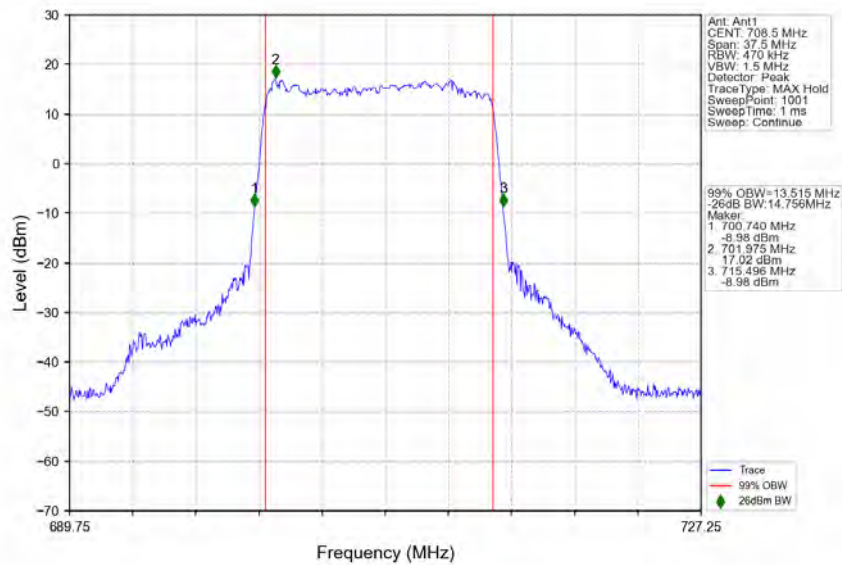
n12_15kHz_SISO_NTNV_15MHz_DFT-s-OFDM_64_QAM_708.5MHz_Outer_Full
