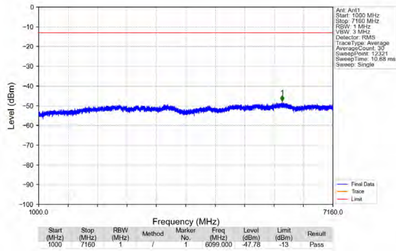
n12_15kHz_SISO_NTNV_5MHz_DFT-s-OFDM_QPSK_713.5MHz_Edge_1RB_Right
