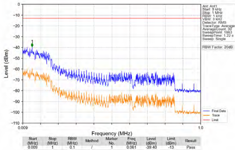
n12_15kHz_SISO_NTNV_15MHz_CP-OFDM_QPSK_708.5MHz_Edge_1RB_Right
