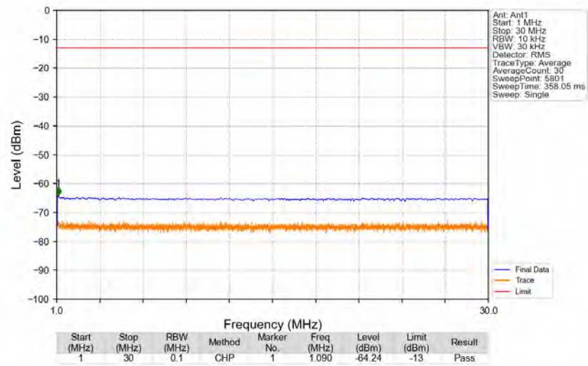
n12_15kHz_SISO_NTNV_10MHz_DFT-s-OFDM_QPSK_704MHz_Edge_1RB_Left
