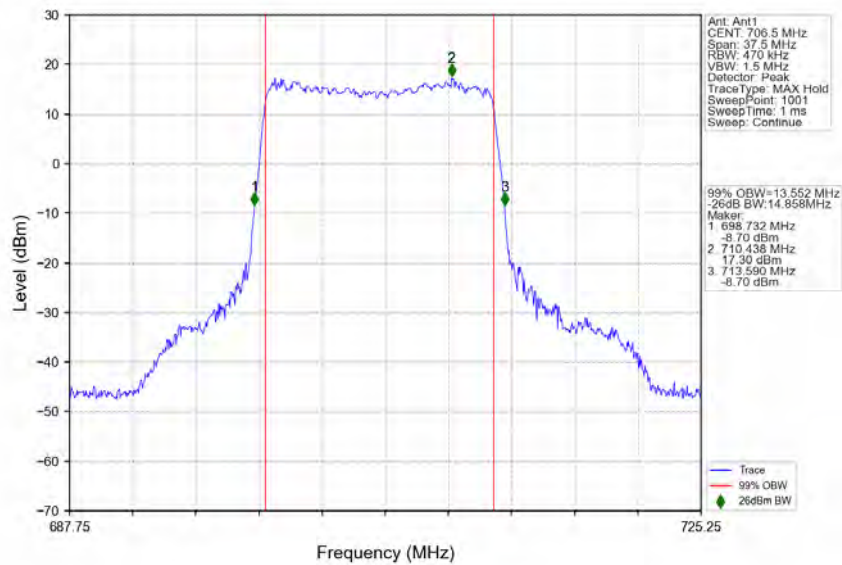
n12_15kHz_SISO_NTNV_15MHz_DFT-s-OFDM_64QAM_706.5MHz_Outer_Full
