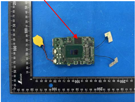
eMMC Chip
