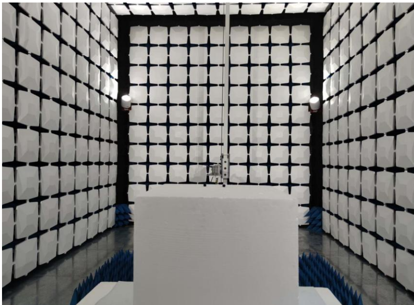
Above 1GHz for radiated emission test setup
