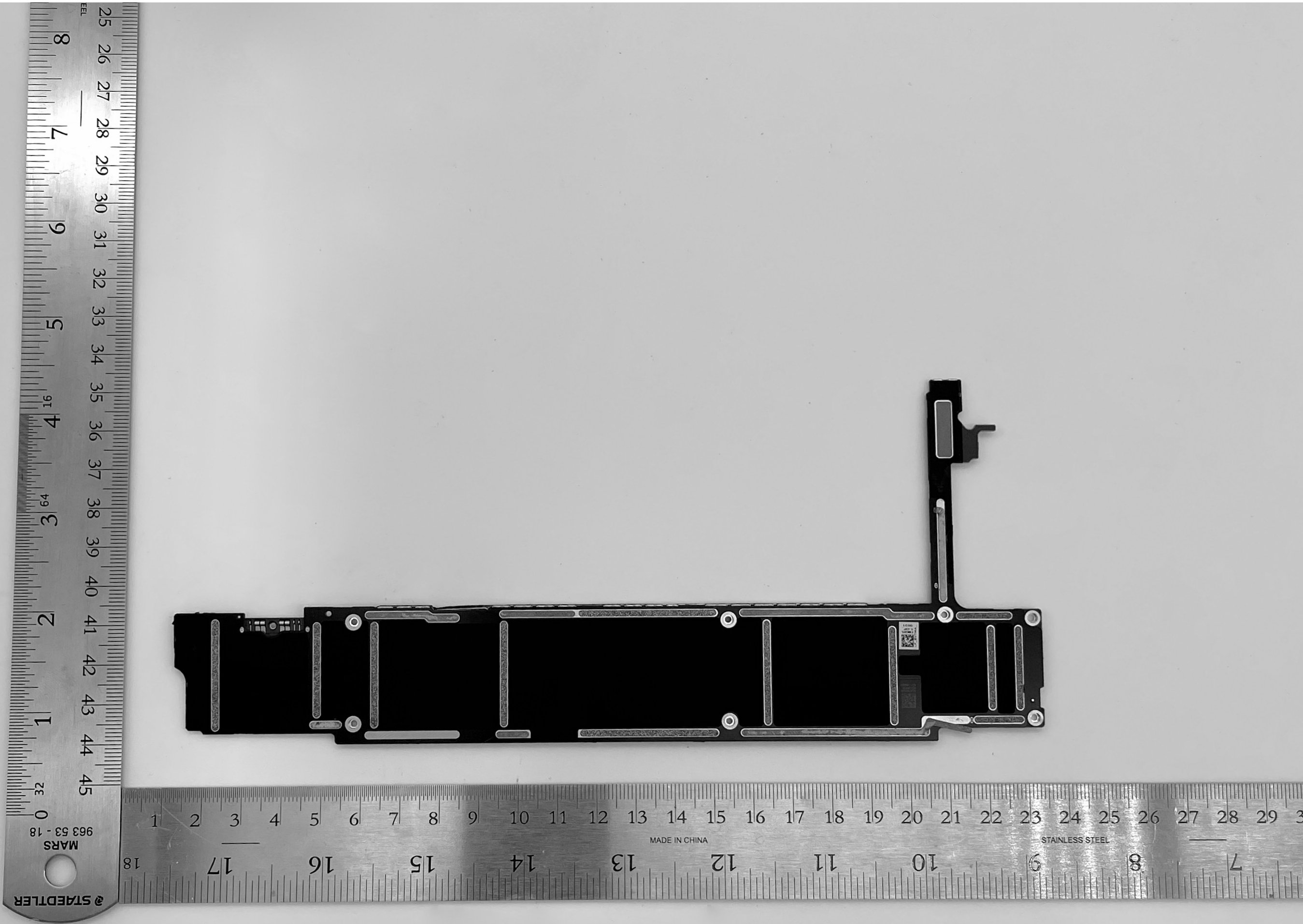
A2435 MLB - Back
