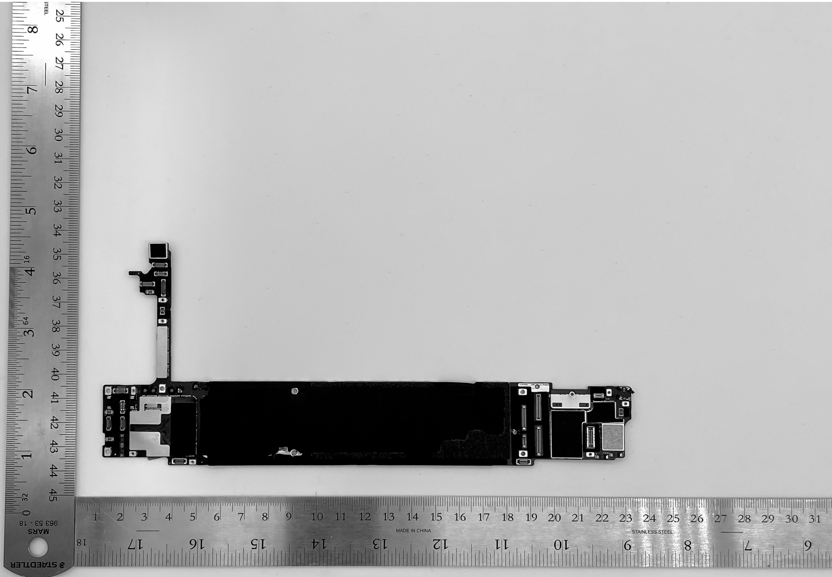
A2435 MLB with Shield - Front
