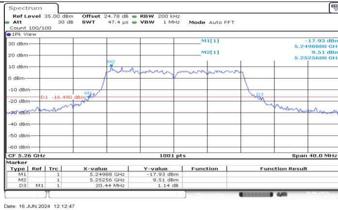
11A-CDD_Ant4_5260
