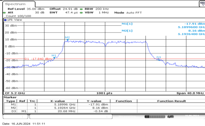
11A-CDD_Ant4_5200
