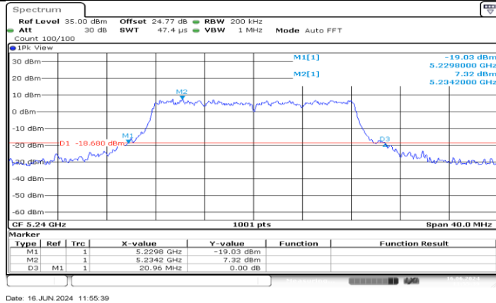
11A-CDD_Ant4_5240
