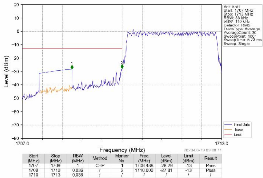
Band4_3MHz_16QAM_LCH_1711.5MHz_RB_15_0_NTNV
