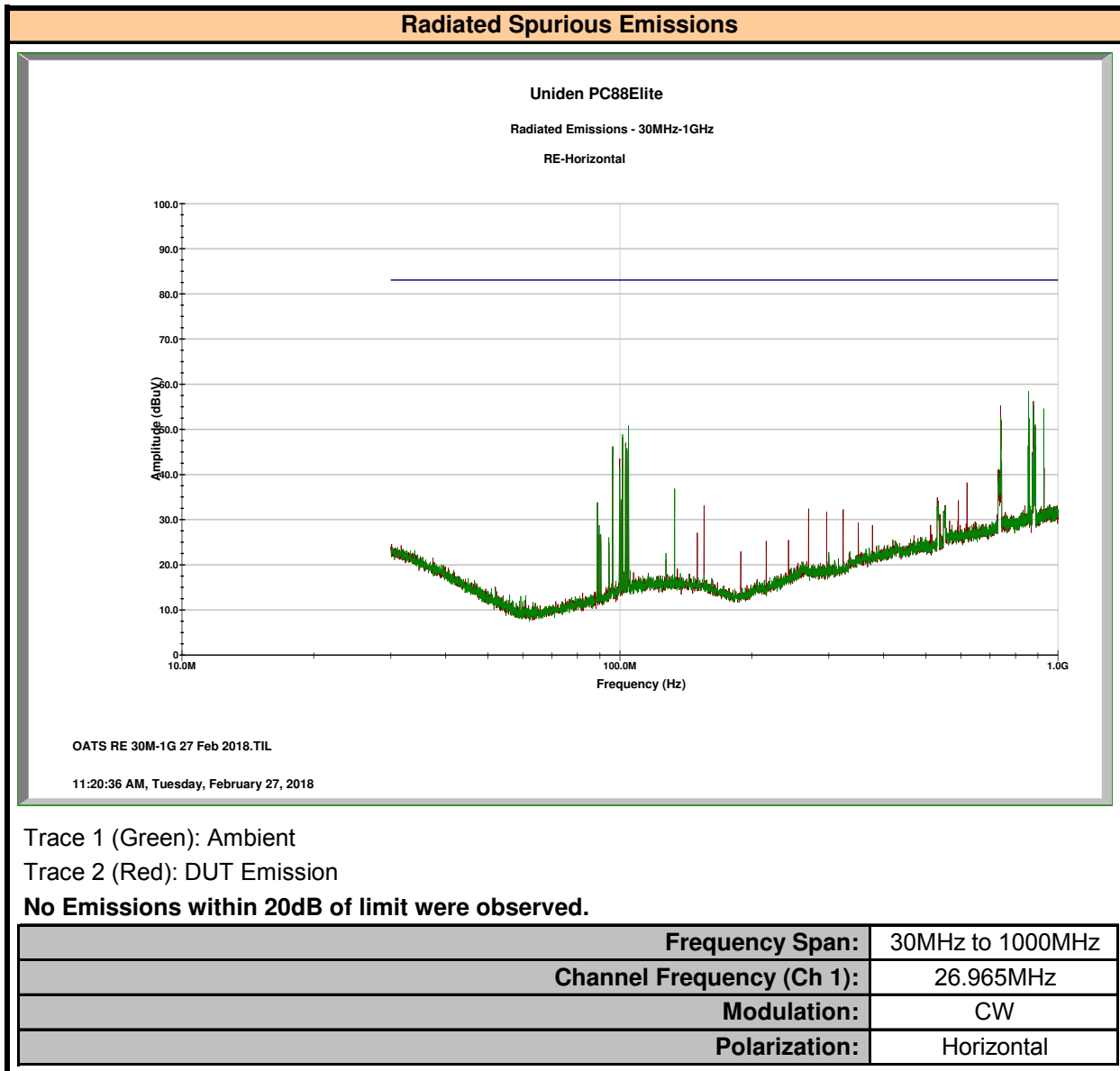
Plot 11.2 – Radiated Spurious Emissions, 30MHz – 1000MHz, Horizontal
