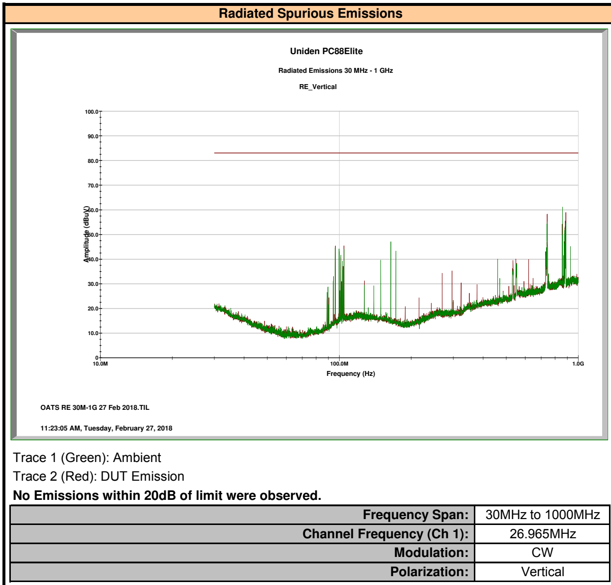
Plot 11.1 – Radiated Spurious Emissions, 30MHz – 1000MHz, Vertical
