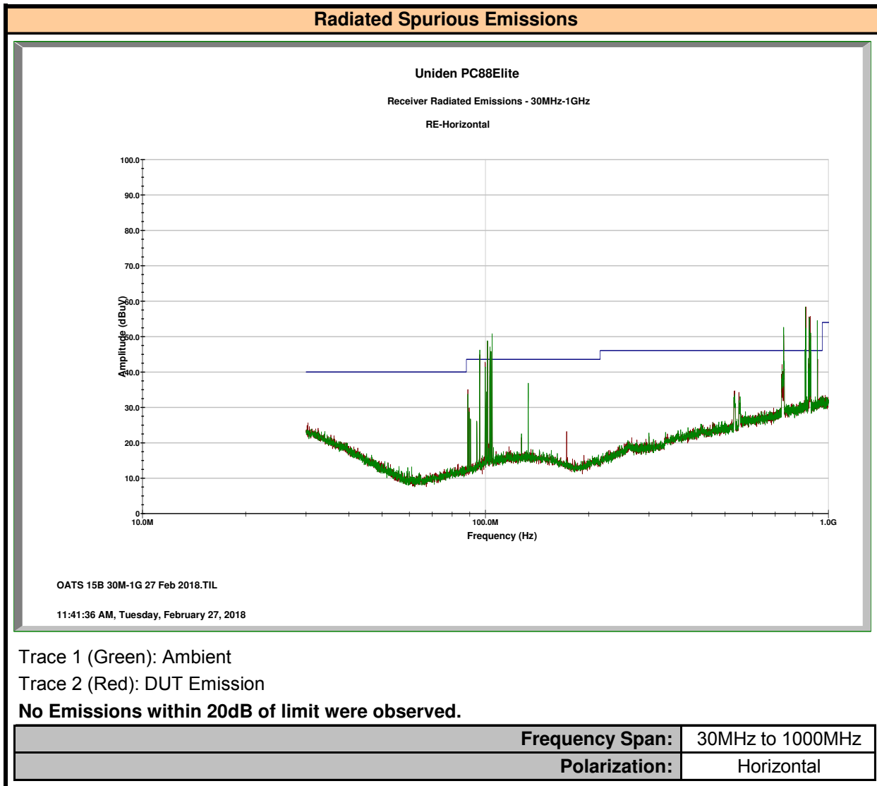
Plot 13.2 – Receiver Radiated Emissions - Horizontal
