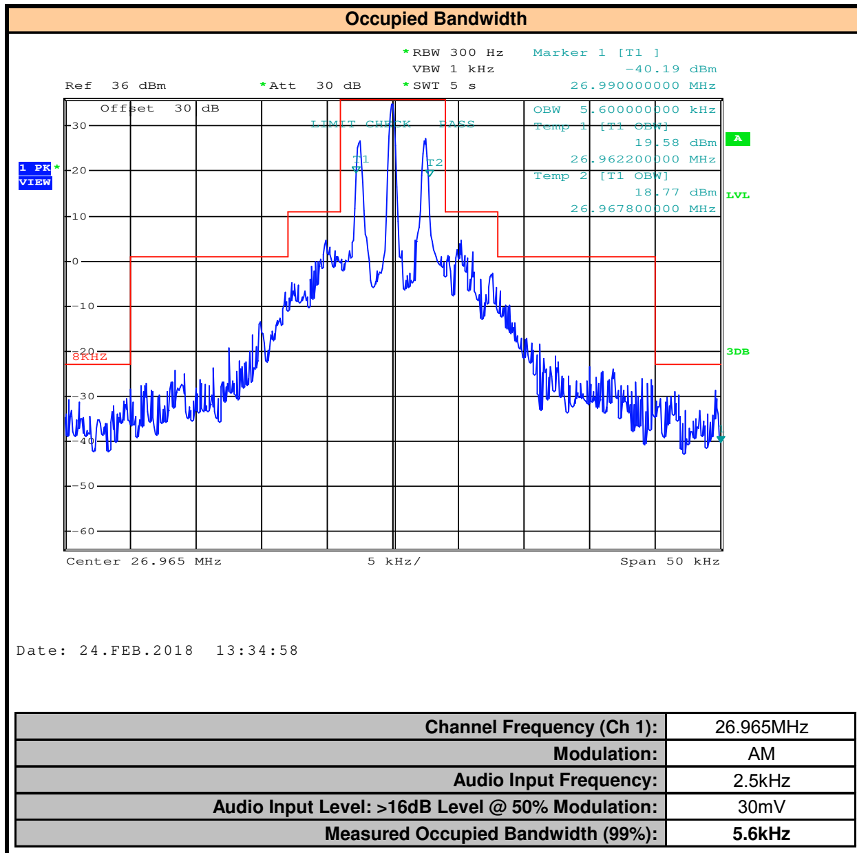
Plot 9.1 – Occupied Bandwidth Channel 1
