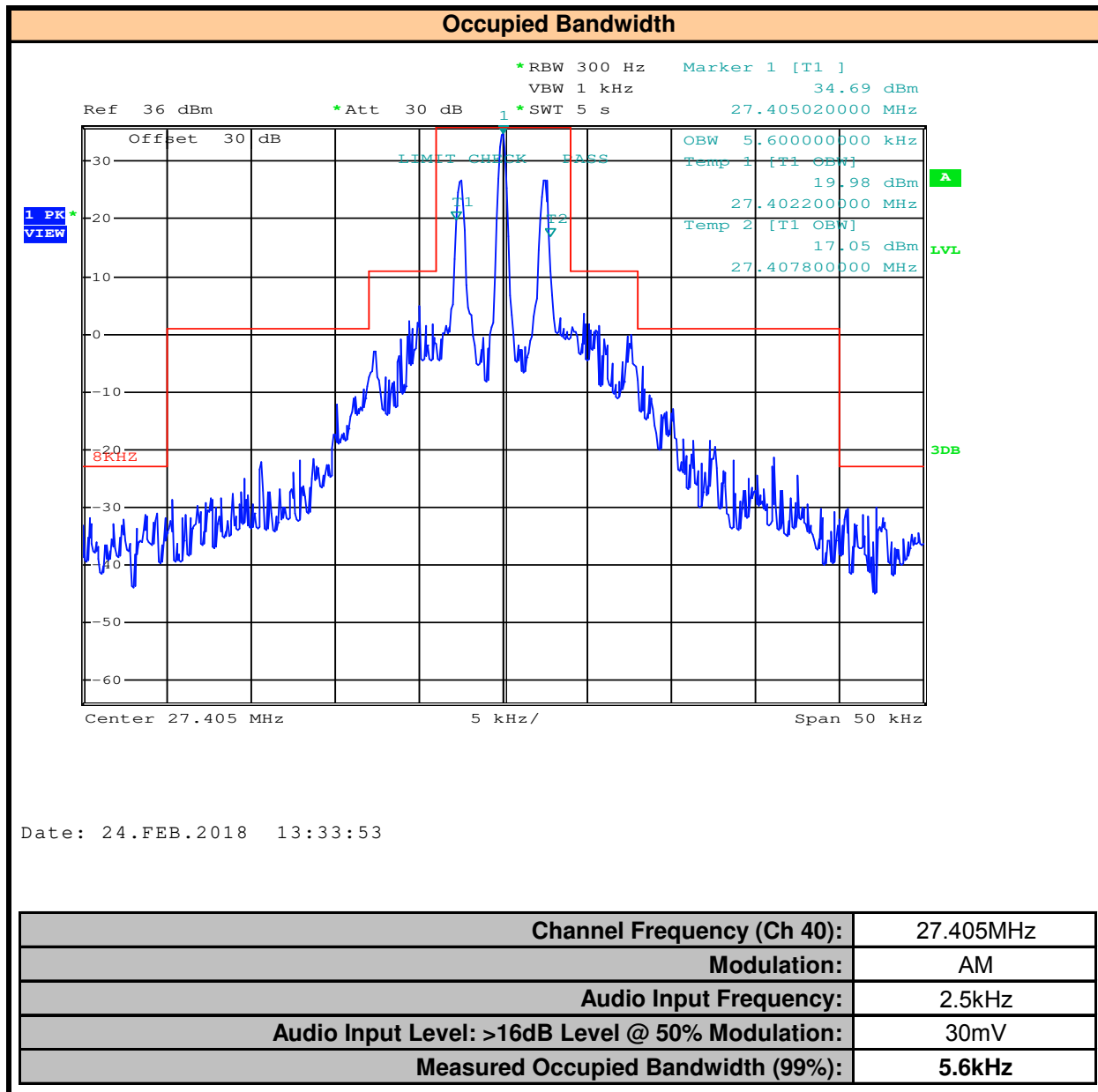
Plot 9.3 – Occupied Bandwidth Channel 40
