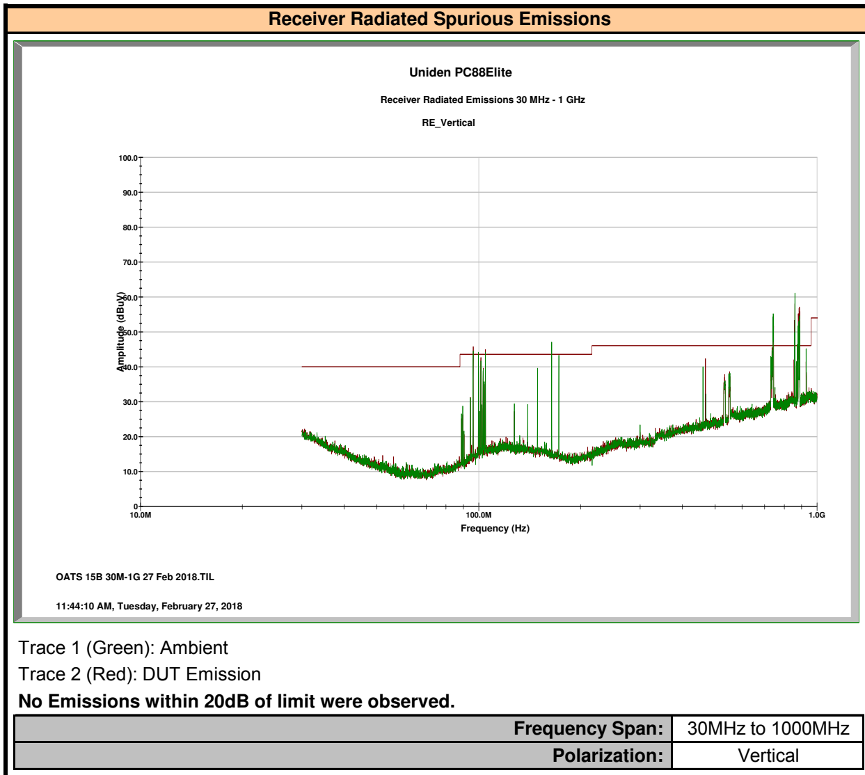
Plot 13.1 – Receiver Radiated Emissions - Vertical
