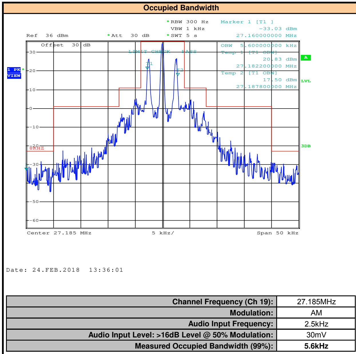
Plot 9.2 – Occupied Bandwidth Channel 19
