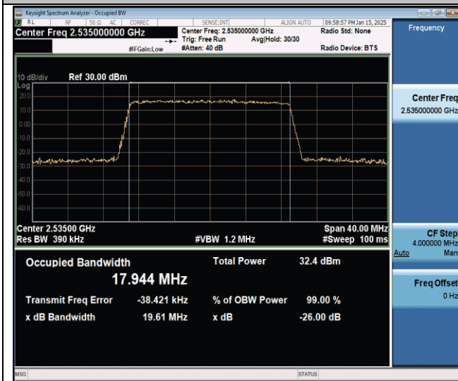
Band7-20MHz-QPSK-21100-100RB#0-PASS
