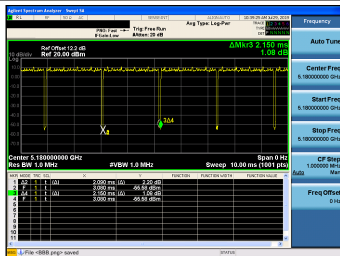
Mode 3: IEEE 802.11ac 20 MHz Continuous TX mode
