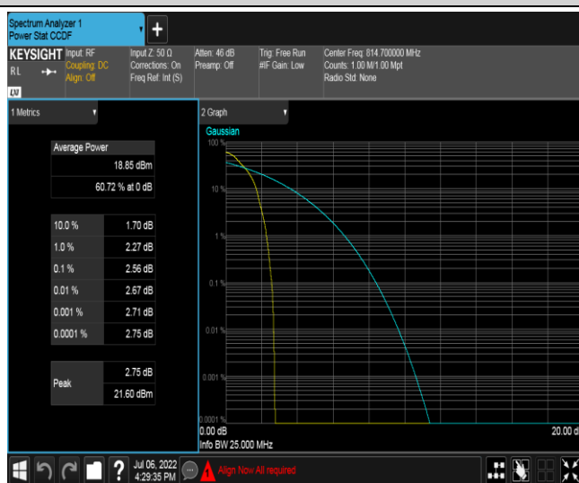
Band26-1.4MHz-QPSK-26697-6RB#0
