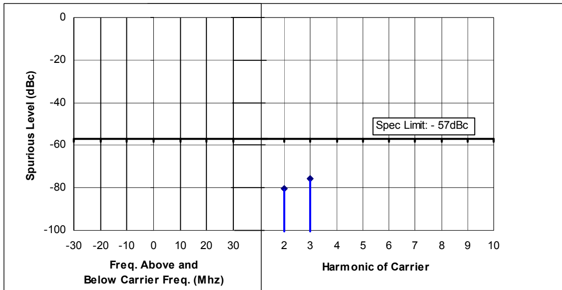
Figure 6F-10: 25 Watts, 136.25 MHz, 25 kHz Channel Spacing
