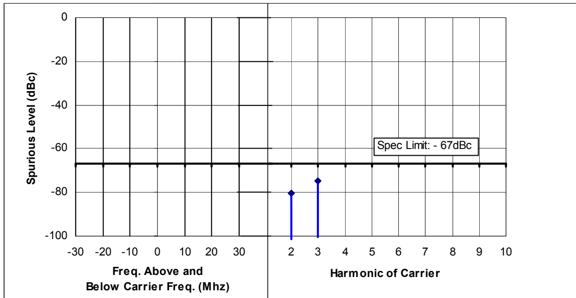
Figure 6F-1: 45 Watts, 136.25 MHz, 12.5 kHz Channel Spacing
