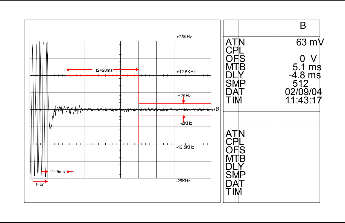
Figure 6I-5: 25 Watts, 12.5 kHz Key-Up Attack Time
