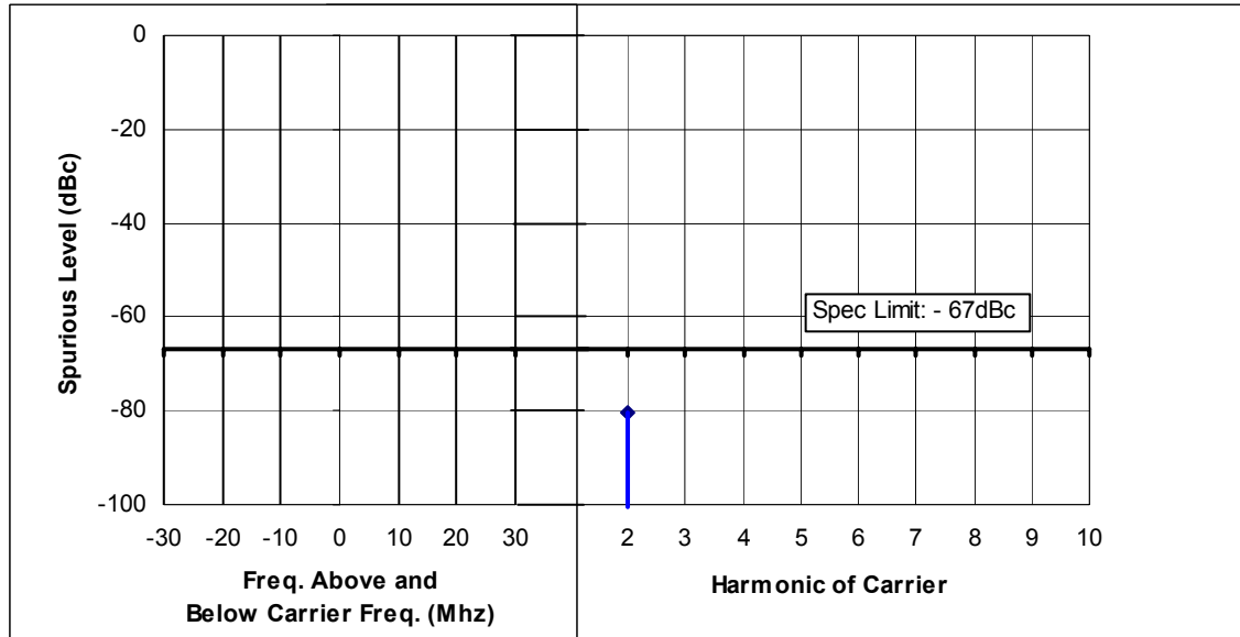
Figure 6F-3: 45 Watts, 161.75 MHz, 12.5 kHz Channel Spacing
