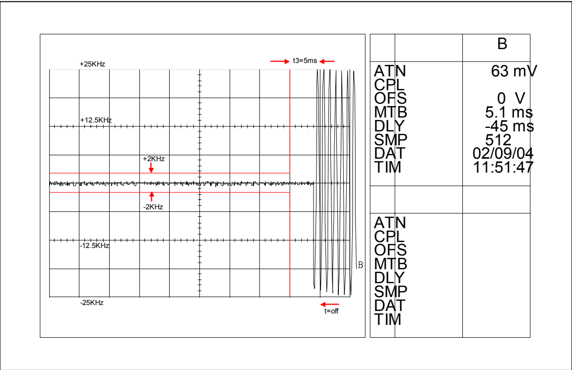
Figure 6I-2: 45 Watts, 12.5 kHz De-Key Decay Time
