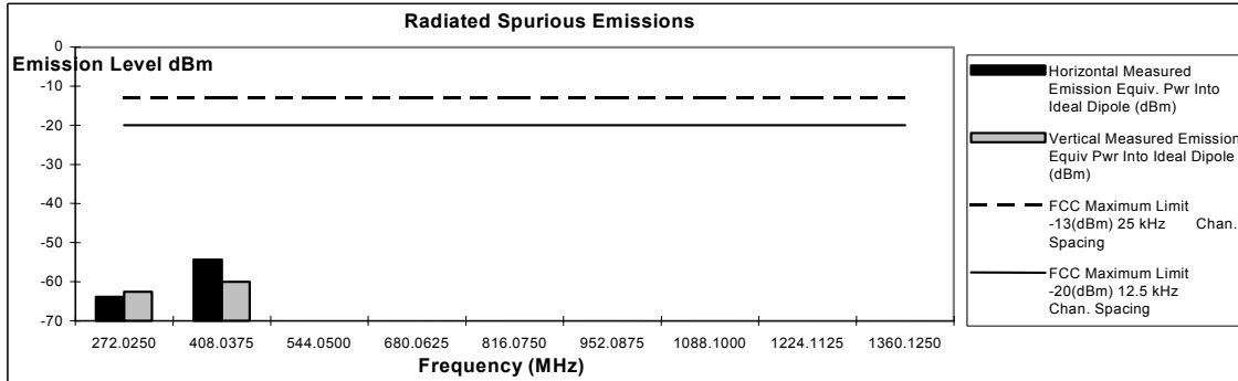
Figure 6G-4 – 25 Watts, 136.0125 MHz
