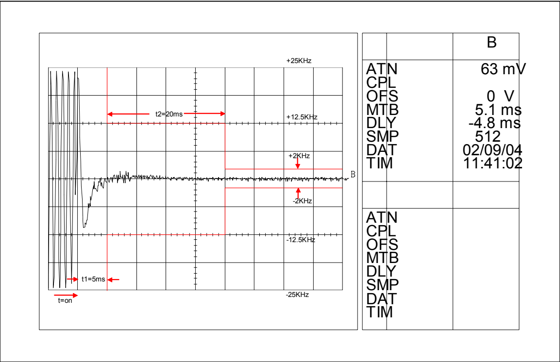
Figure 6I-3: 45 Watts, 25 kHz Key-Up Attack Time
