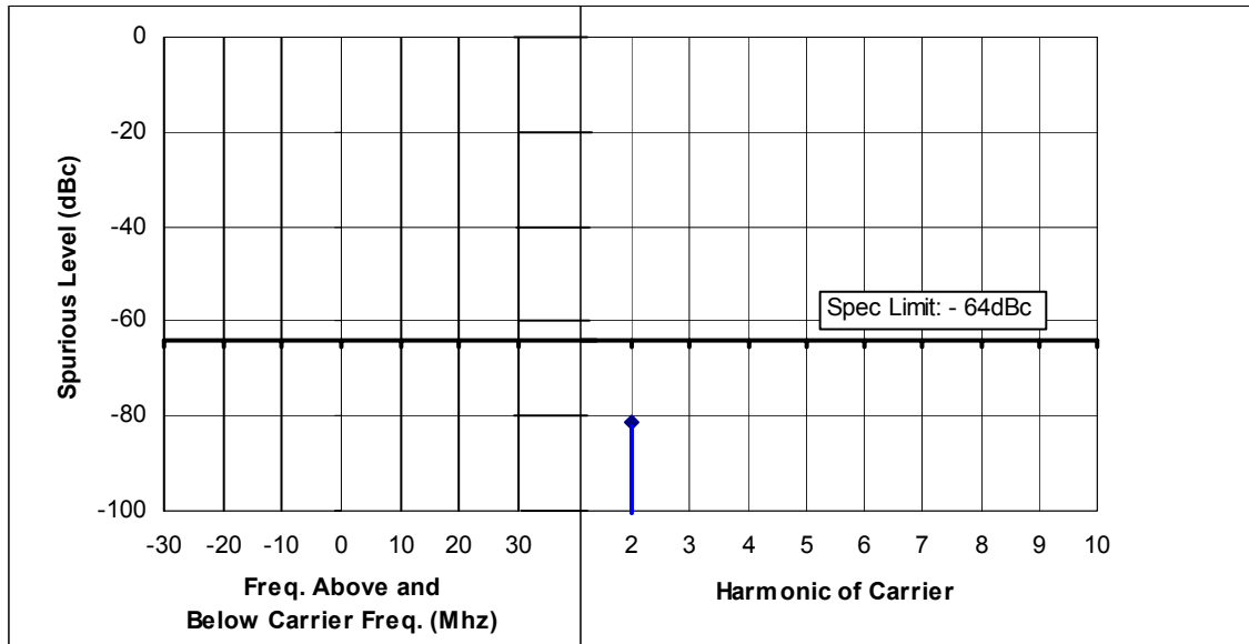
Figure 6F-9: 25 Watts, 161.75 MHz, 12.5 kHz Channel Spacing
