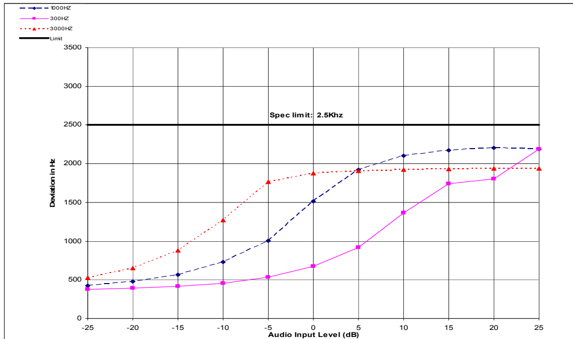
Figure 6D-2: 12.5 kHz Channel Spacing, Tone Private Line (TPL) Mode
