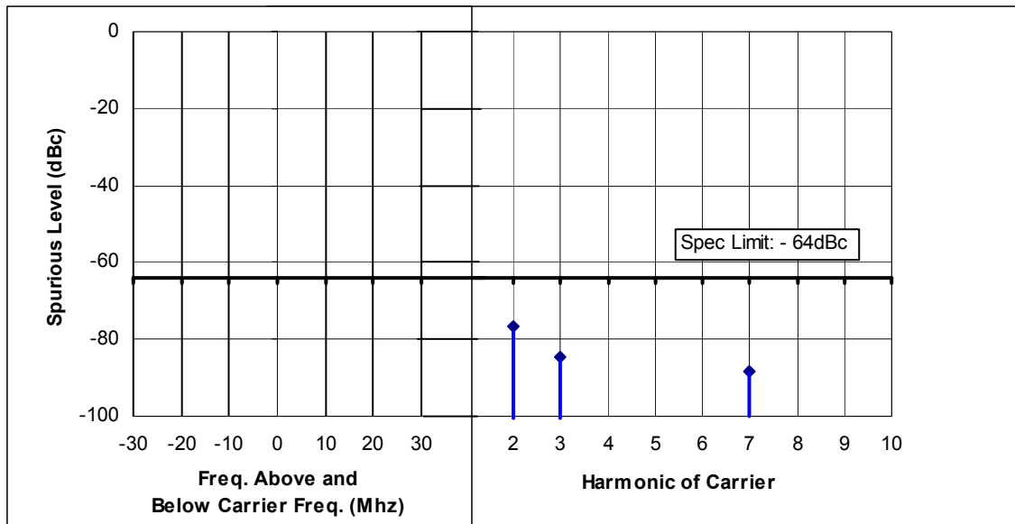
Figure 6F-8: 25 Watts, 149.00 MHz, 12.5 kHz Channel Spacing
