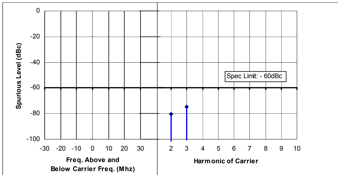
Figure 6F-4: 45 Watts, 136.25 MHz, 25 kHz Channel Spacing
