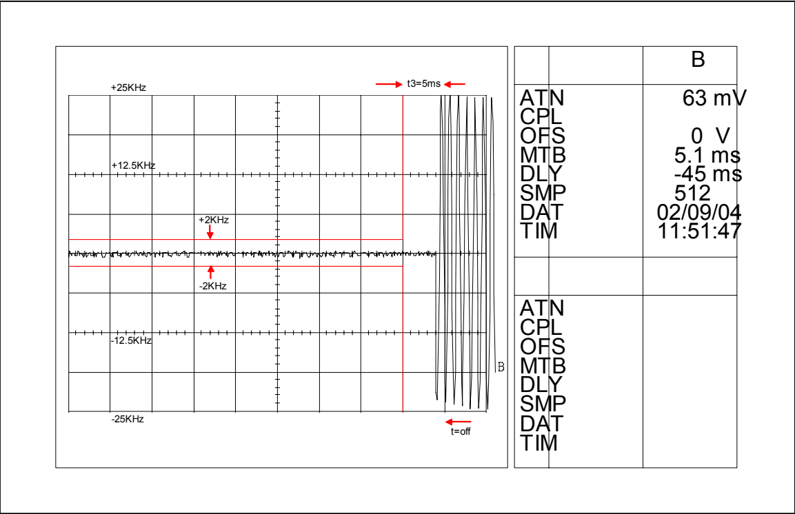
Figure 6I-4: 45 Watts, 25 kHz De-Key Decay Time
