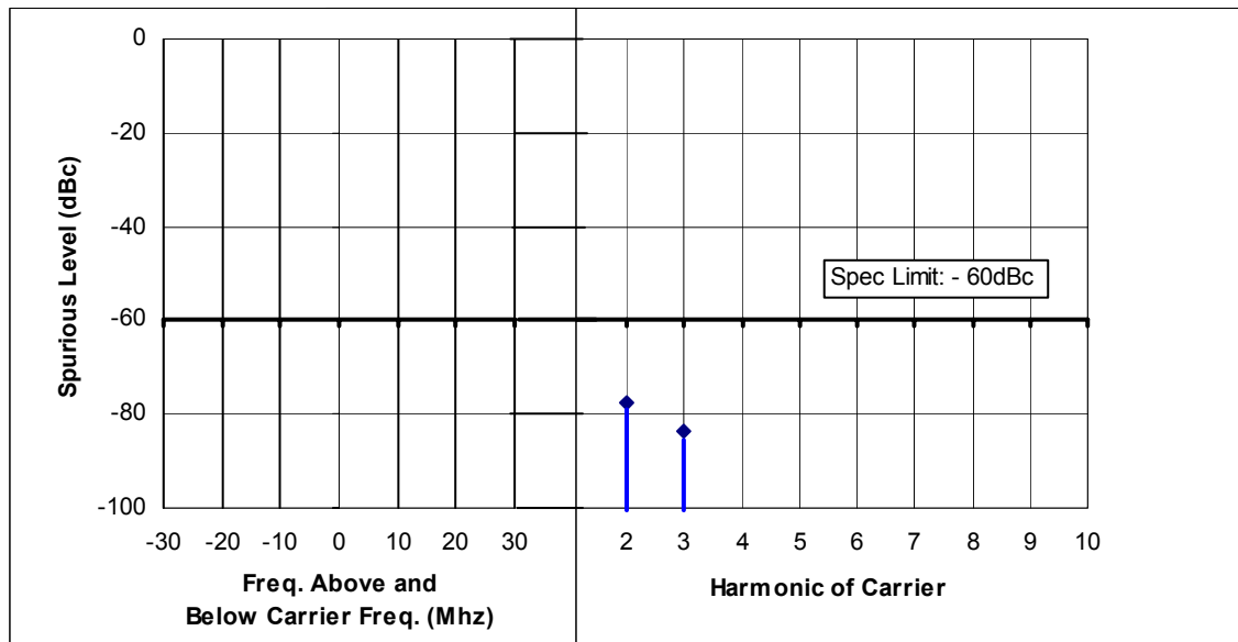
Figure 6F-5: 45 Watts, 149.00MHz, 25 kHz Channel Spacing
