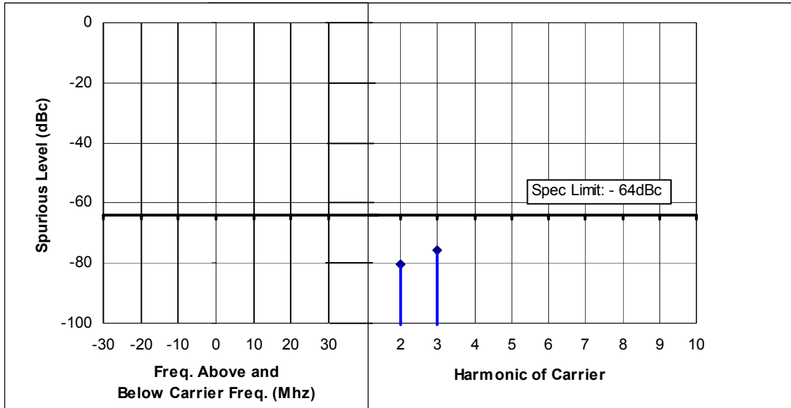
Figure 6F-7: 25 Watts, 136.25 MHz, 12.5 kHz Channel Spacing
