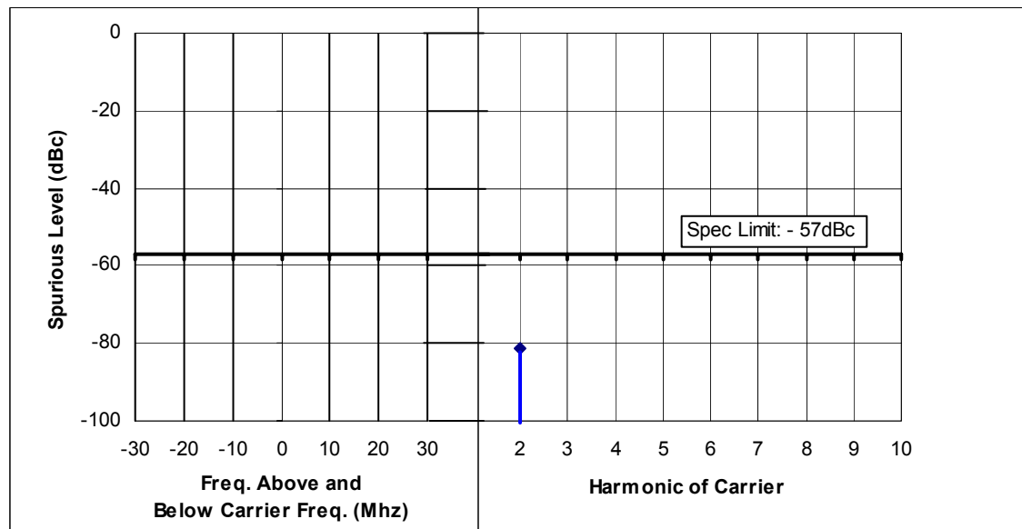
Figure 6F-12: 25 Watts, 161.75 MHz, 25 kHz Channel Spacing
