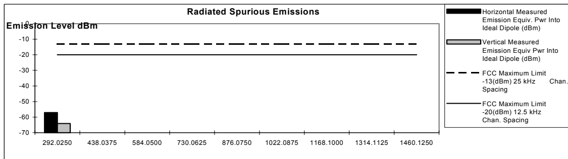
Figure 6G-2 – 45 Watts, 146.0125 MHz
