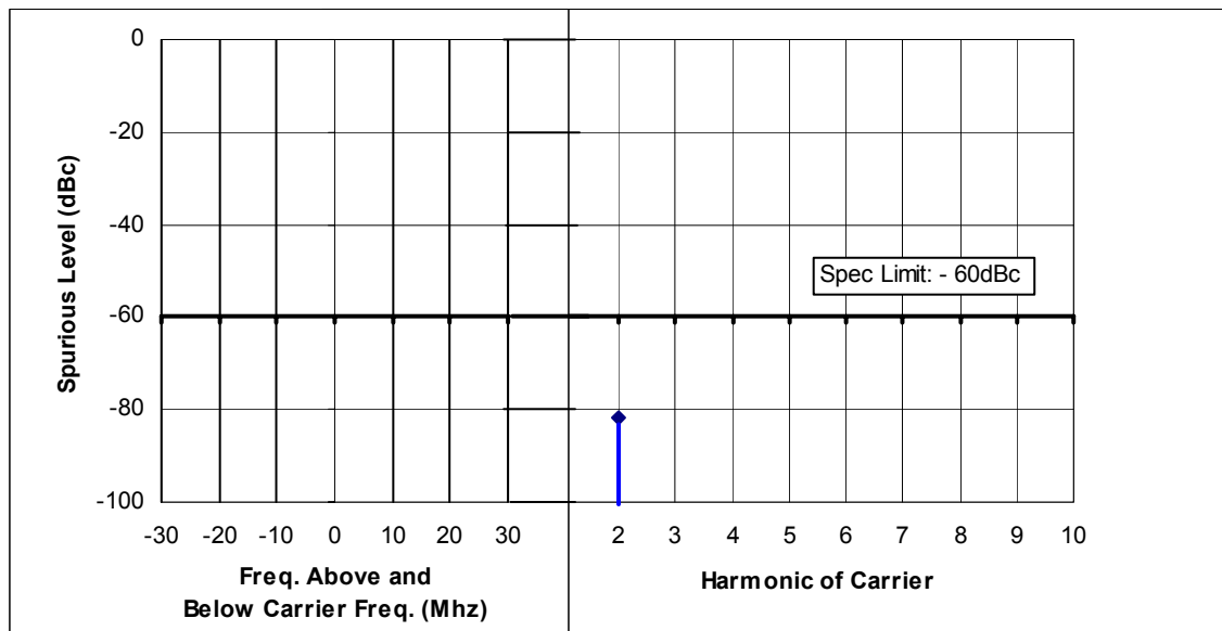
Figure 6F-6: 45 Watts, 161.75 MHz, 25 kHz Channel Spacing
