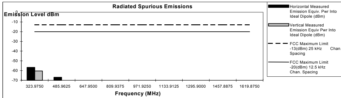
Figure 6G-3 – 45 Watts, 161.9875 MHz
