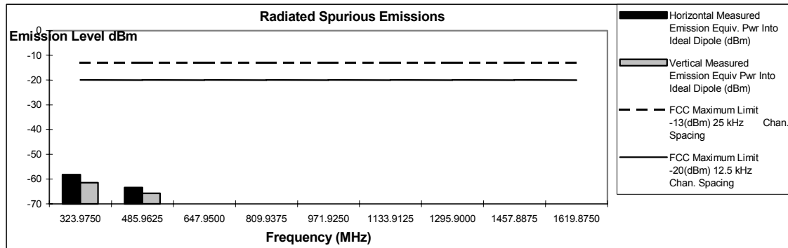
Figure 6G-6 – 25 Watts, 161.9875 MHz
