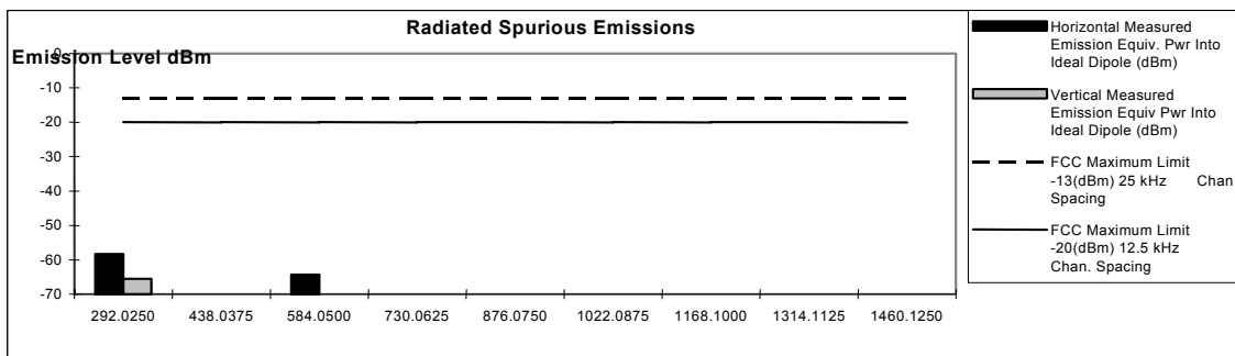
Figure 6G-5 – 25 Watts, 146.0125 MHz
