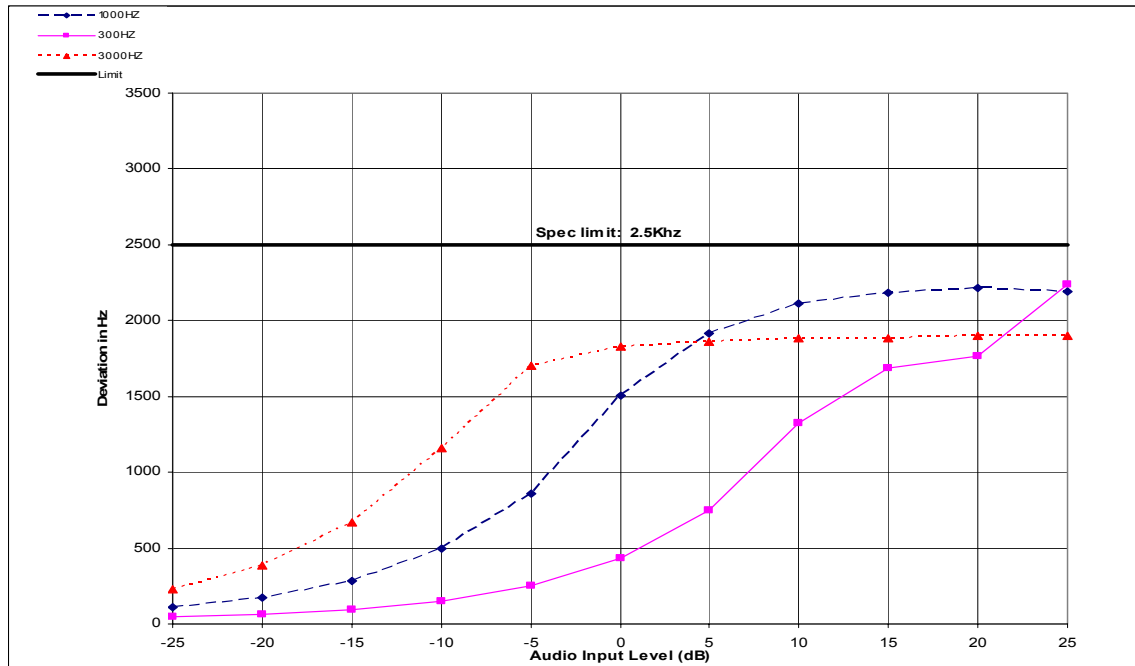
Figure 6D-1: 12.5 kHz Channel Spacing, Carrier Squelch Mode
