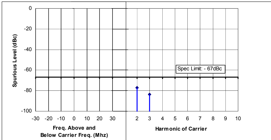
Figure 6F-2: 45 Watts, 149.00 MHz, 12.5 kHz Channel Spacing
