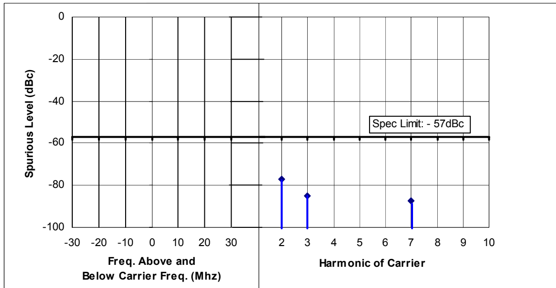
Figure 6F-11: 25 Watts, 149.00 MHz, 25 kHz Channel Spacing
