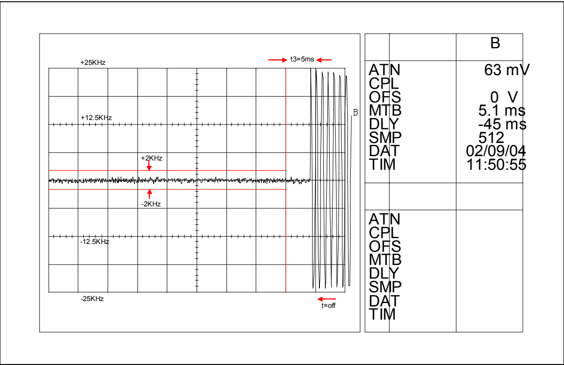
Figure 6I-6: 25 Watts, 12.5 kHz De-Key Decay Time
