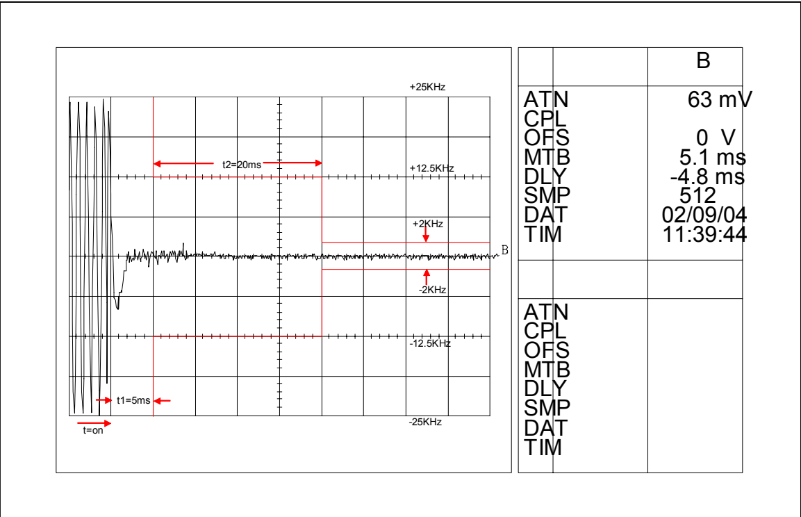
Figure 6I-1: 45 Watts, 12.5 kHz Key-Up Attack Time
