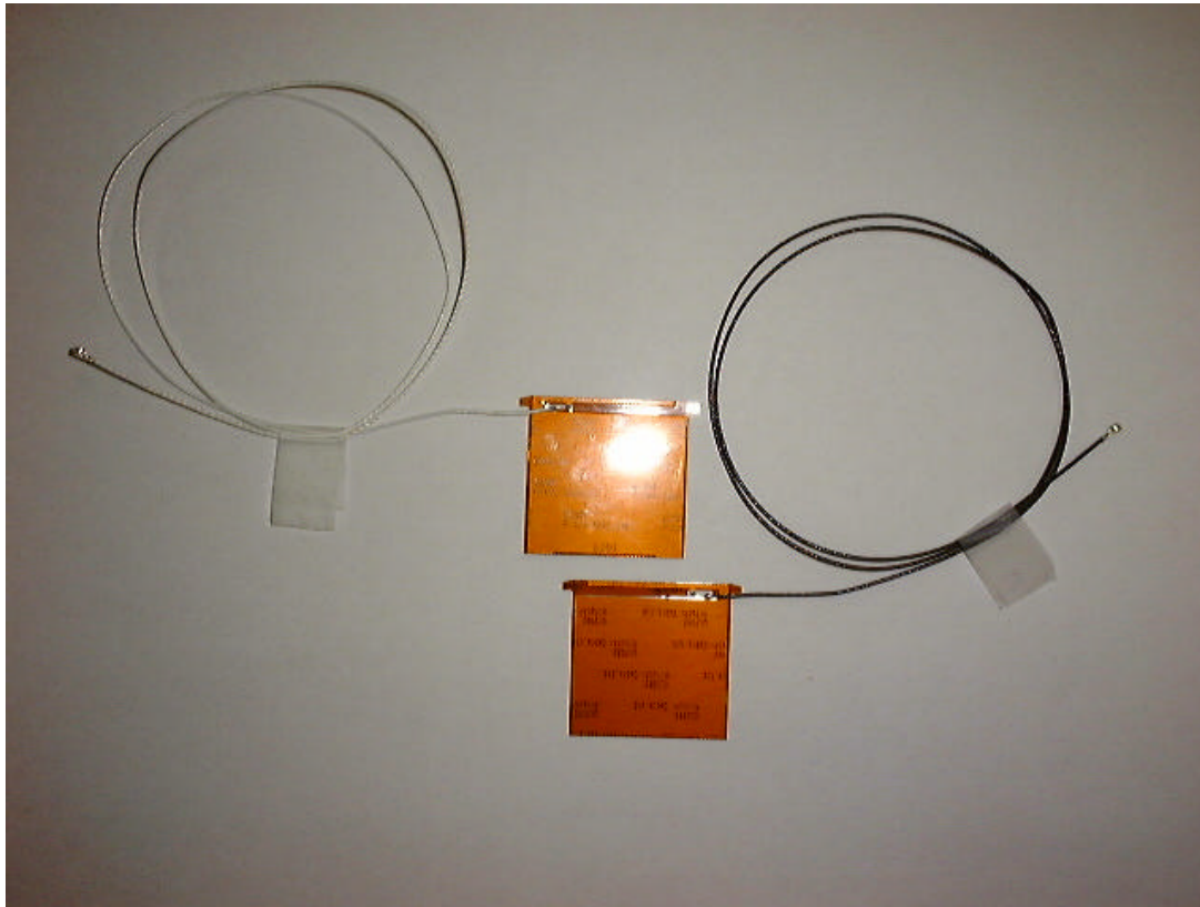
Front and rear view 'Film Antenna'
