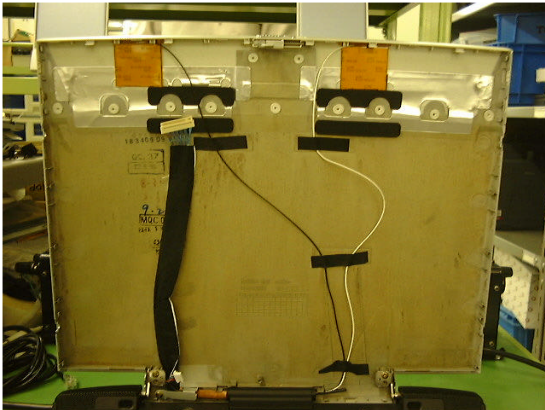
positioning of 'Film Antenna'
