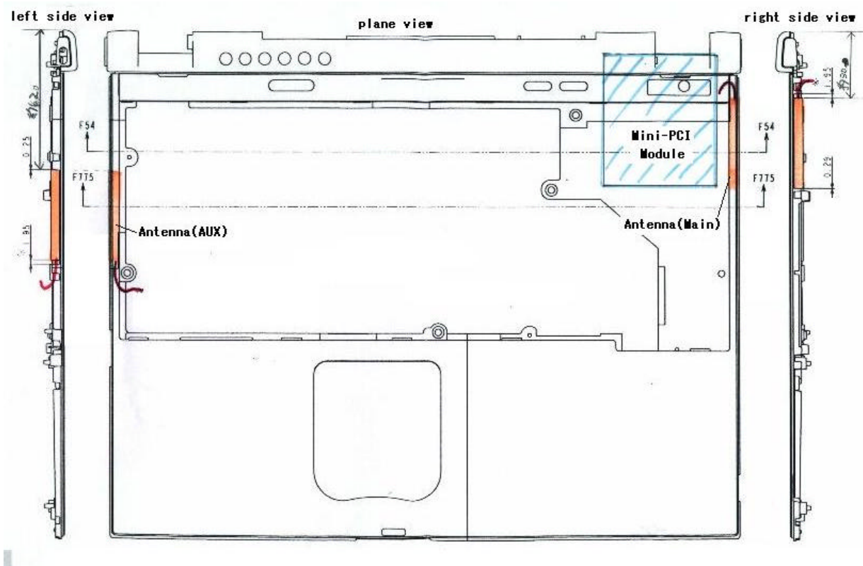
positioning of 'Stick On Antenna'
