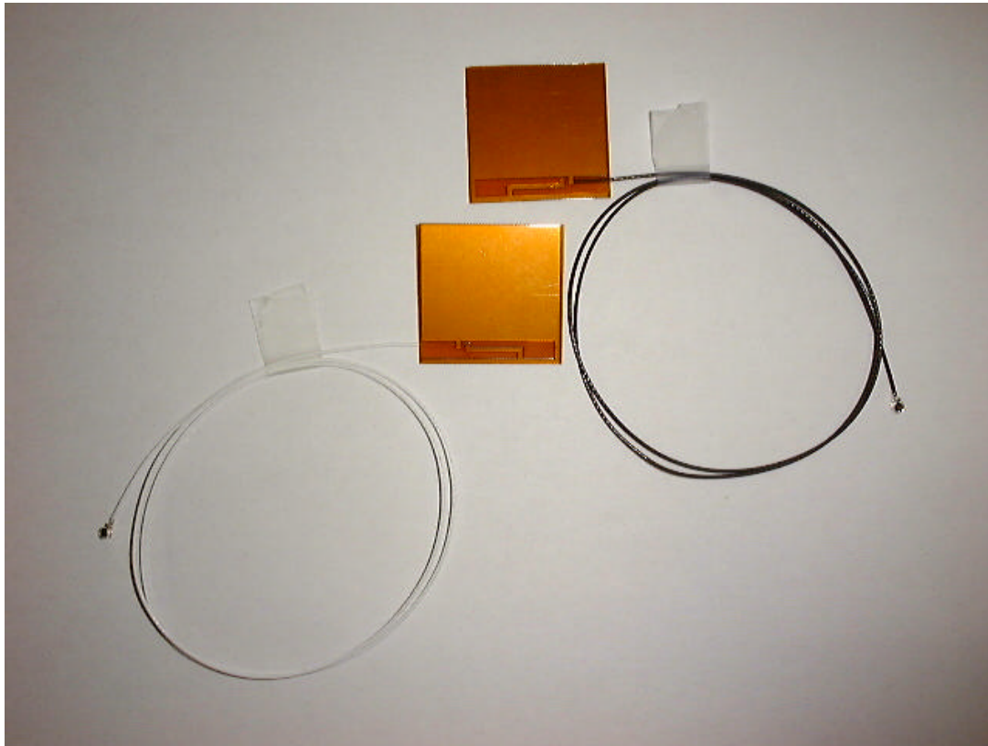
Front and rear view 'Dual Film Antenna'
