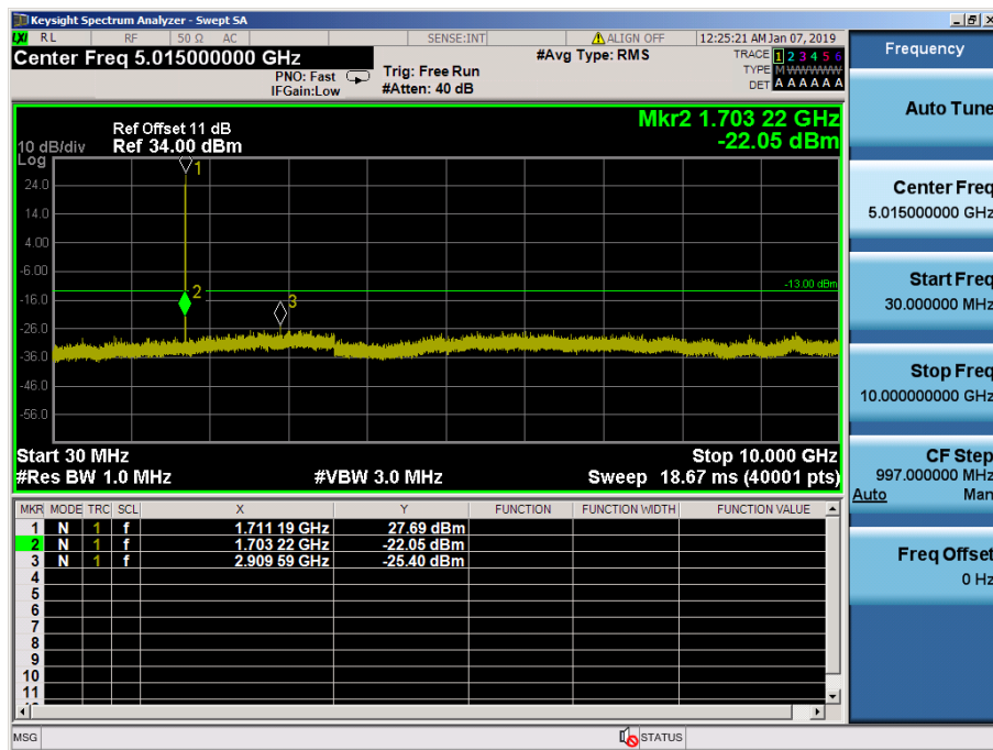
LTE Band 66, 4 / 1.4MHz / 64QAM - RB Size/Offset (6/0) – Low Channel
