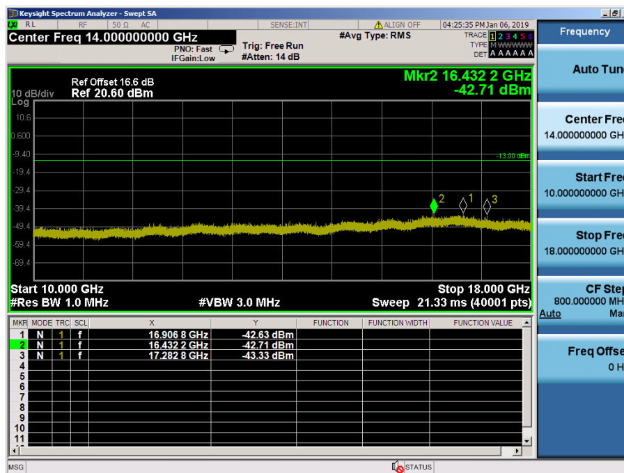
LTE Band 66, 4 / 1.4MHz / QPSK - RB Size/Offset (3/2) – High Channel
