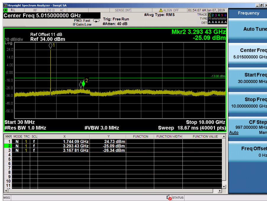
LTE Band 66, 4 / 5MHz / 64QAM - RB Size/Offset (25/0) – Mid Channel
