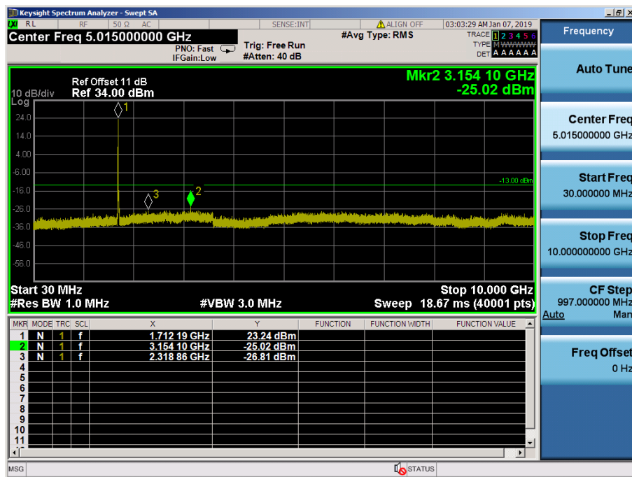
LTE Band 66, 4 / 15MHz / 64QAM - RB Size/Offset (36/0)–Low Channel
