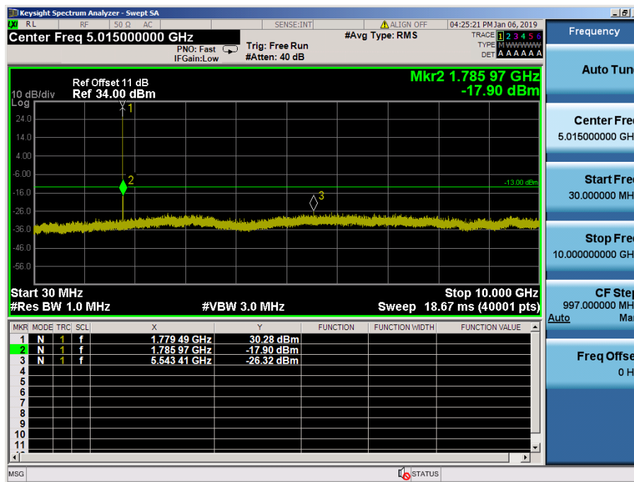
LTE Band 66, 4 / 1.4MHz / QPSK - RB Size/Offset (3/2) – High Channel
