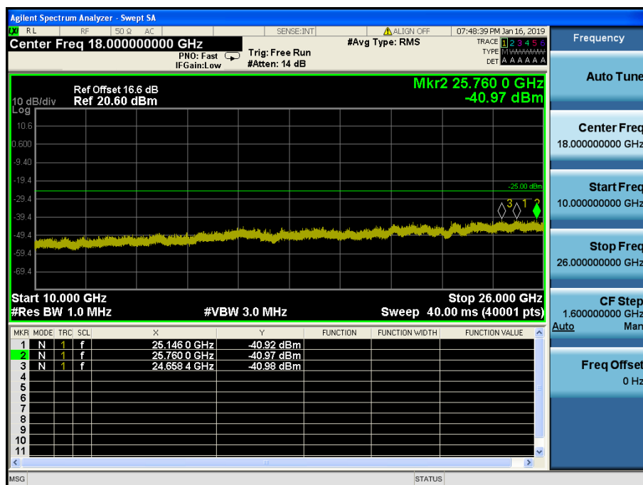
LTE Band 7 / 5MHz / QPSK - RB Size/Offset (1/12) – High Channel
