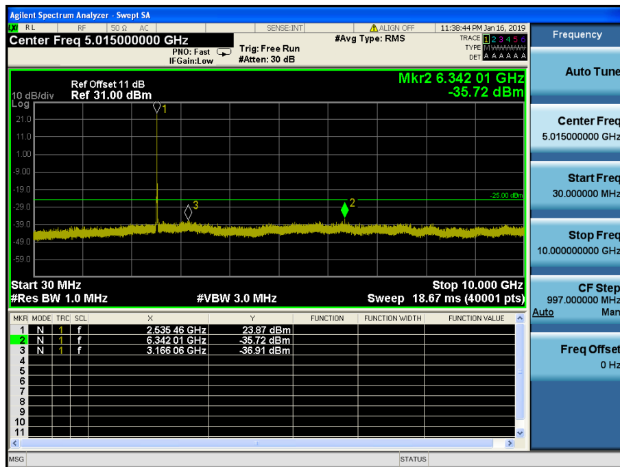
LTE Band 7 / 5MHz / 64QAM - RB Size/Offset (25/0) – Mid Channel
