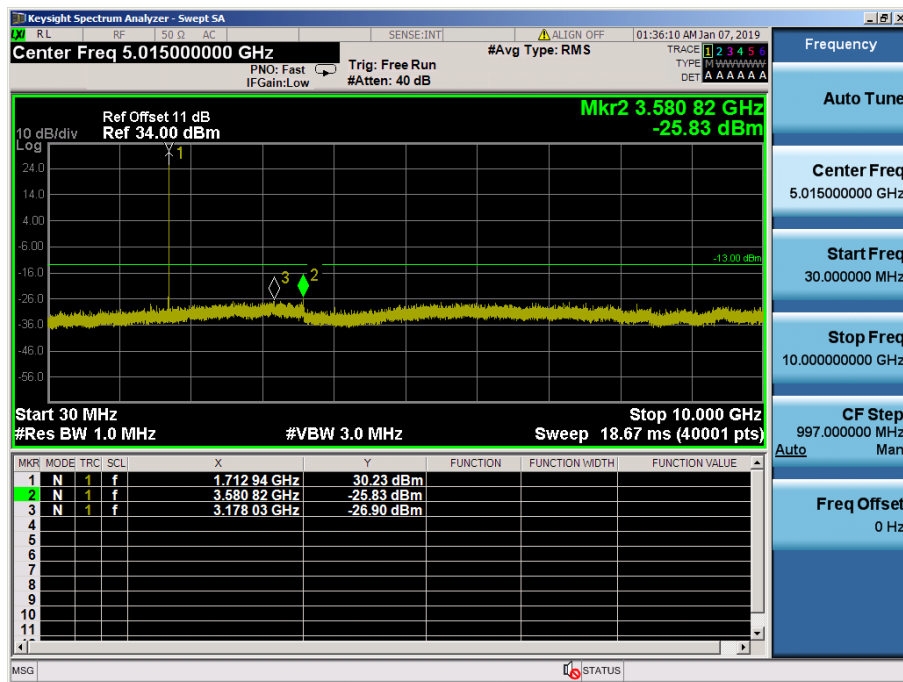
LTE Band 66, 4 / 5MHz / 64QAM - RB Size/Offset (1/12) – Low Channel
