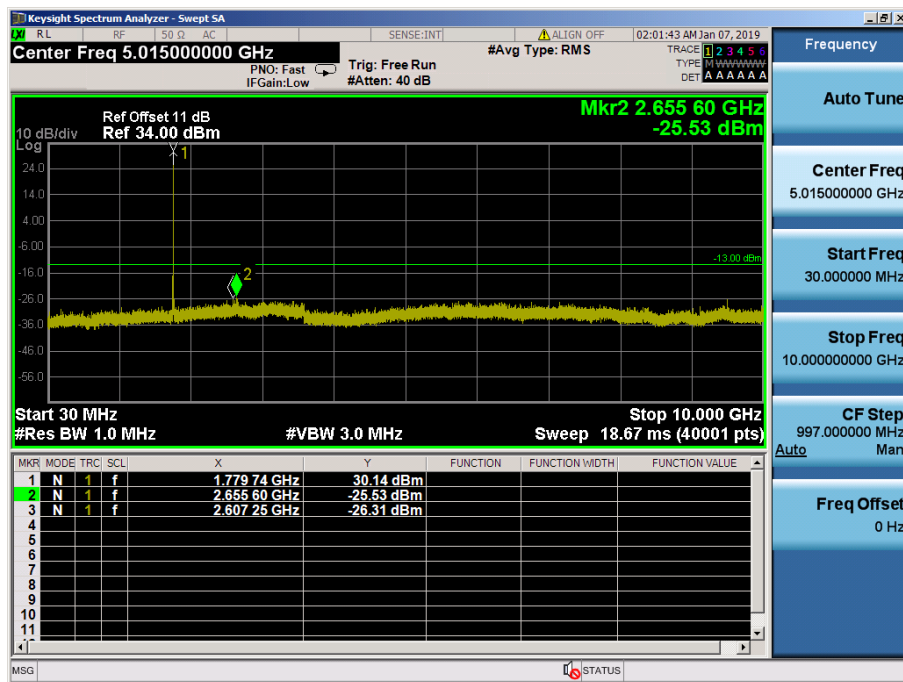
LTE Band 66, 4 / 5MHz / 64QAM - RB Size/Offset (1/24) – High Channel
