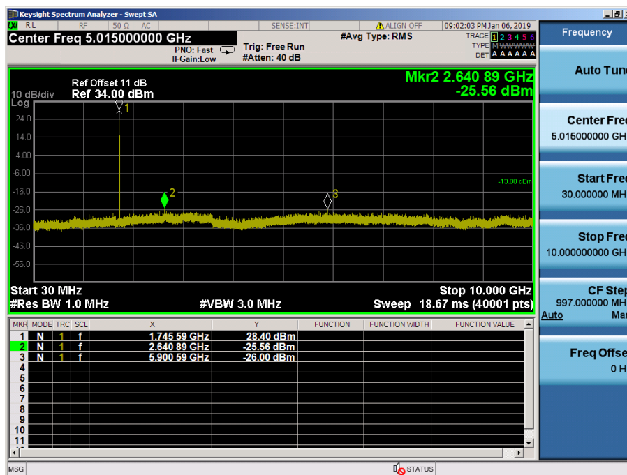
LTE Band 66, 4 / 3MHz / 16QAM - RB Size/Offset (8/4) – Mid Channel
