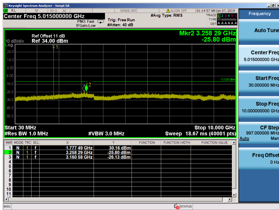
LTE Band 66, 4 / 3MHz / 64QAM - RB Size/Offset (1/0) – High Channel
