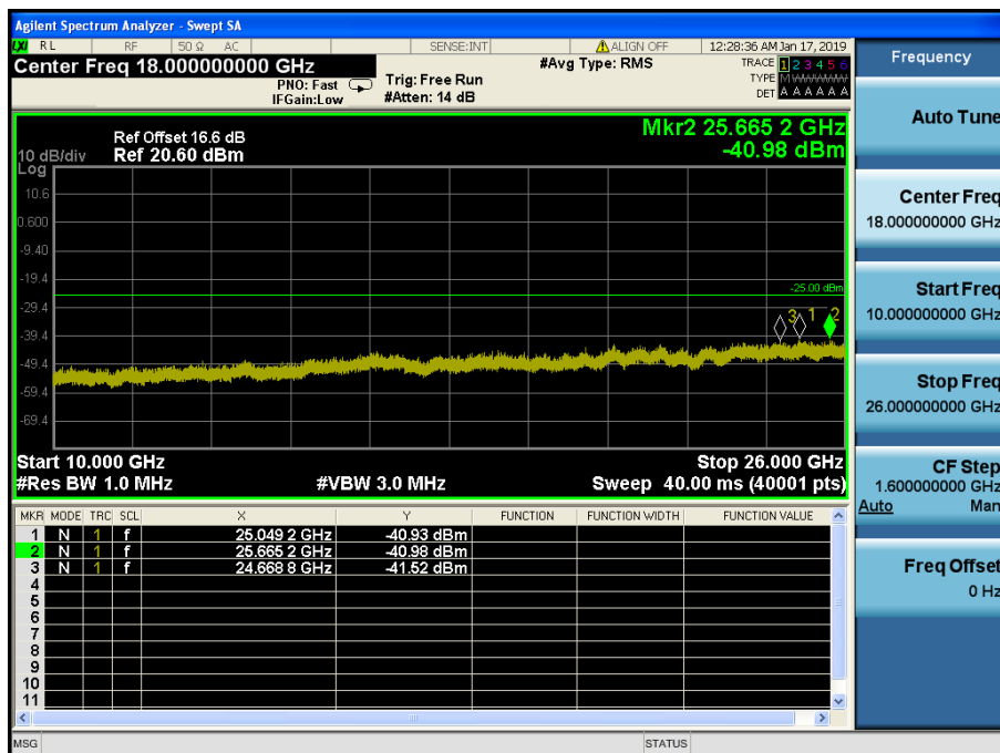
LTE Band 7 / 15MHz / 64QAM - RB Size/Offset (1/0) – Mid Channel
