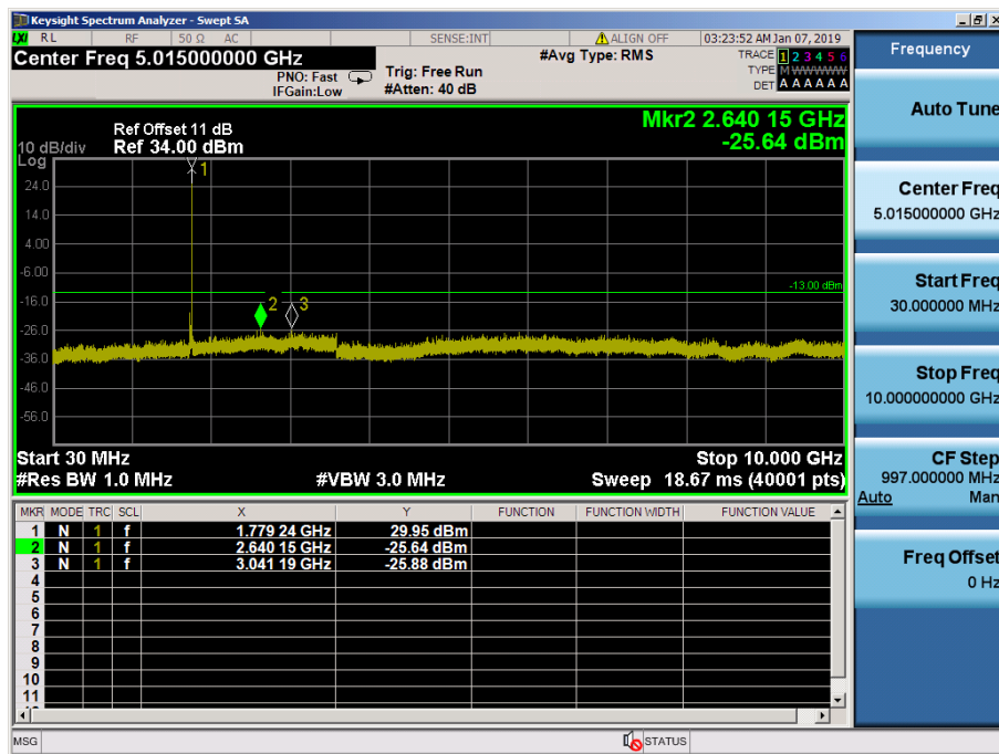
LTE Band 66, 4 / 15MHz / 64QAM - RB Size/Offset (1/74) – High Channel
