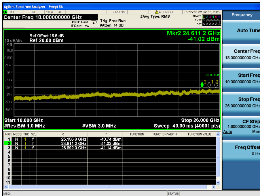
LTE Band 7 / 10MHz / 16QAM - RB Size/Offset (1/49) – Low Channel
