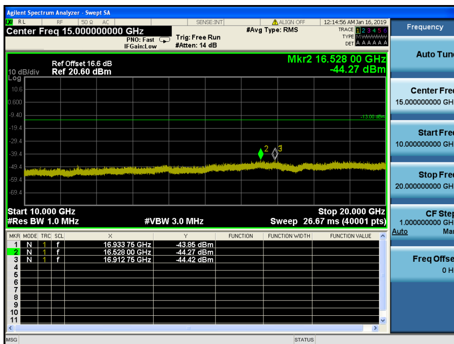
LTE Band 2 / 10MHz / QPSK - RB Size/Offset (50/0) – Mid Channel
