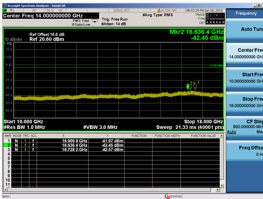
LTE Band 66, 4 / 3MHz / 16QAM - RB Size/Offset (1/0) – Low Channel
