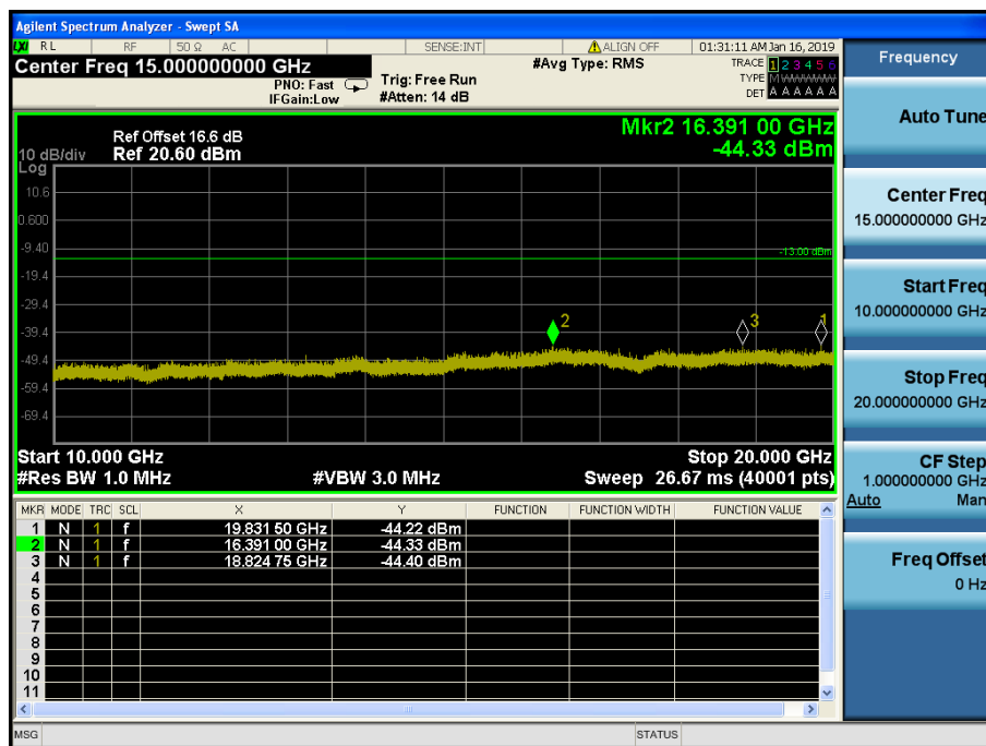
LTE Band 2 / 20MHz / QPSK - RB Size/Offset (50/50) –Low Channel
