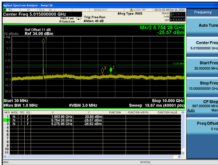
LTE Band 2 / 15MHz / 64QAM - RB Size/Offset (75/0)–Low Channel
