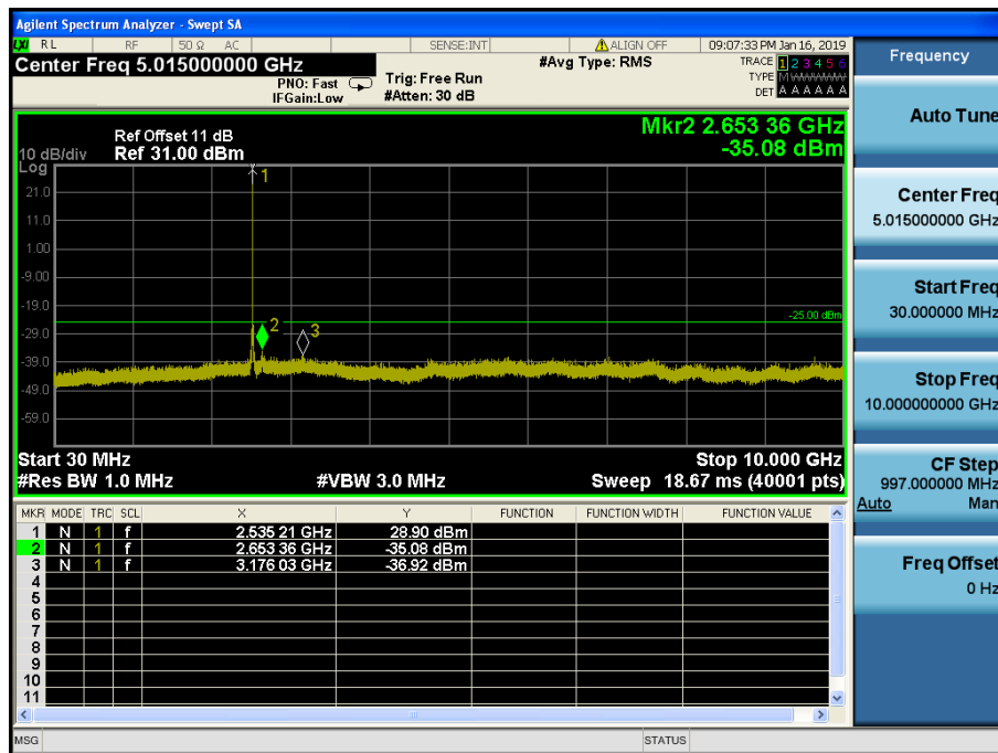
LTE Band 7 / 20MHz / QPSK - RB Size/Offset (1/50) – Mid Channel
