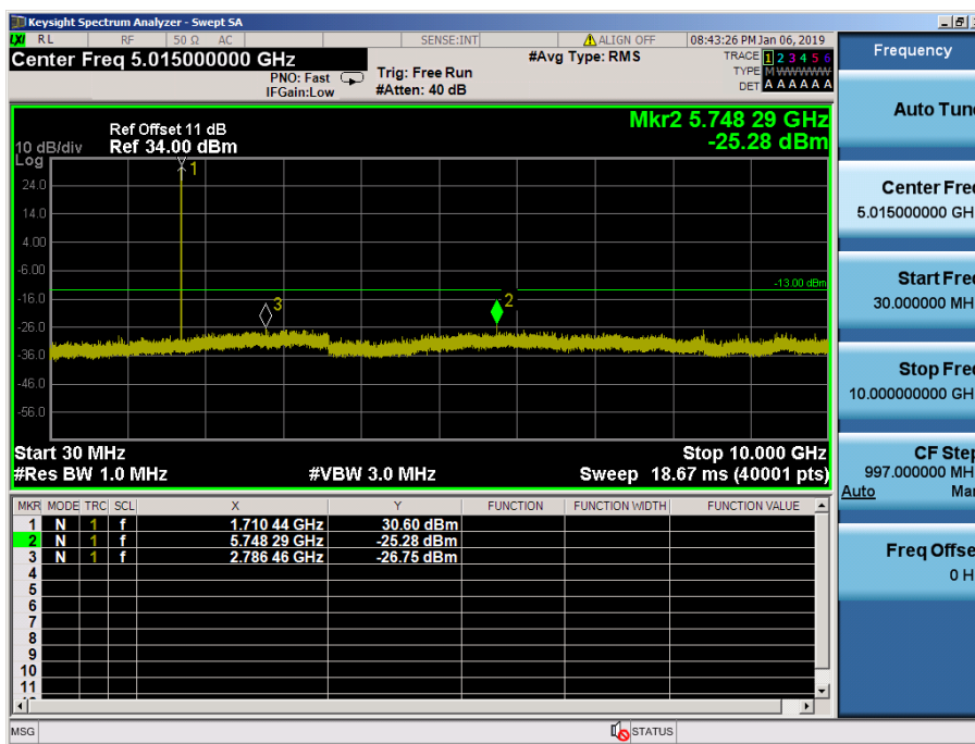
LTE Band 66, 4 / 3MHz / 16QAM - RB Size/Offset (1/0) – Low Channel
