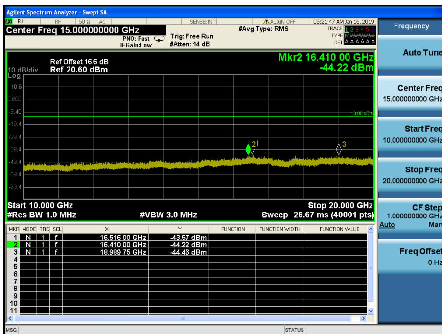
LTE Band 2 / 15MHz / 16QAM - RB Size/Offset (36/0) – High Channel
