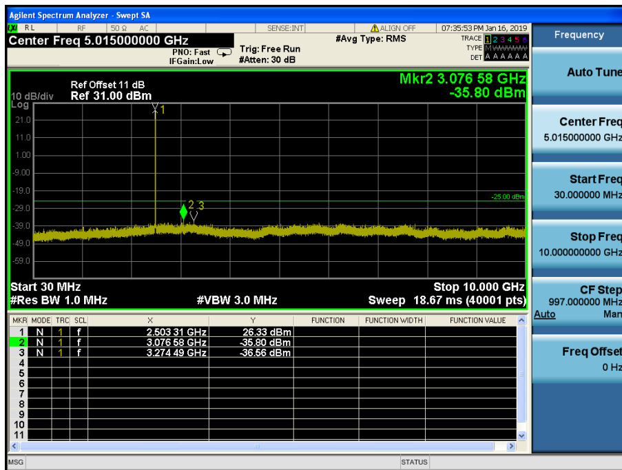
LTE Band 7 / 5MHz / QPSK - RB Size/Offset (12/13) – Low Channel
