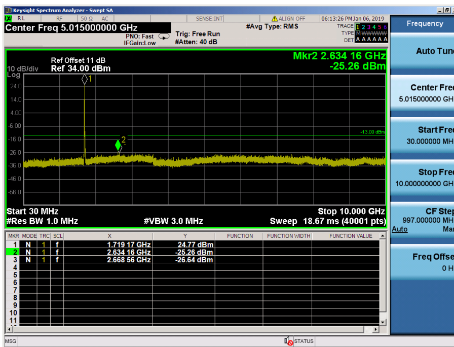
LTE Band 66, 4 / 10MHz / QPSK - RB Size/Offset (50/0) – Low Channel
