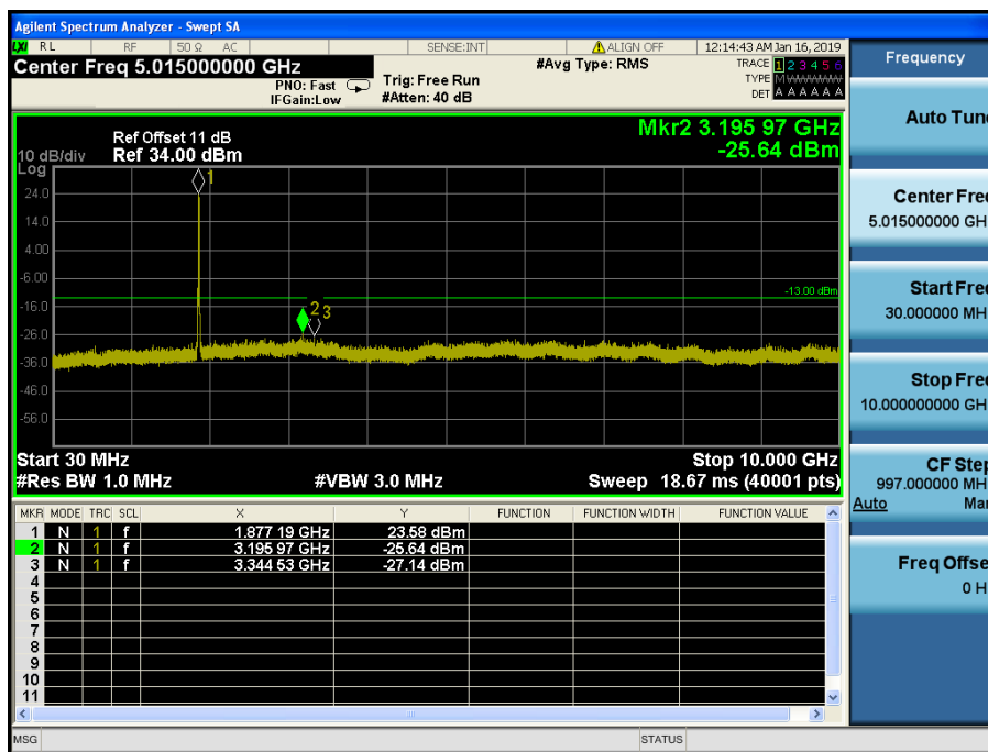
LTE Band 2 / 10MHz / QPSK - RB Size/Offset (50/0) – Mid Channel
