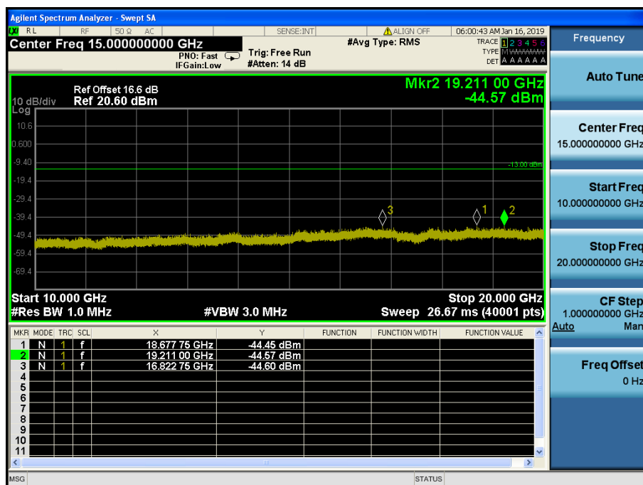
LTE Band 2 / 20MHz / 16QAM - RB Size/Offset (1/99) – High Channel
