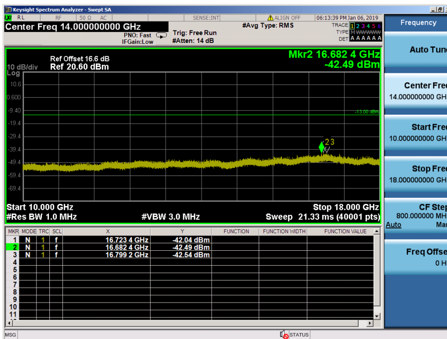
LTE Band 66, 4 / 10MHz / QPSK - RB Size/Offset (50/0) – Low Channel
