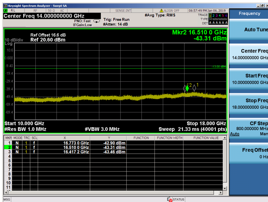
LTE Band 66, 4 / 15MHz / QPSK - RB Size/Offset (36/18) – Mid Channel
