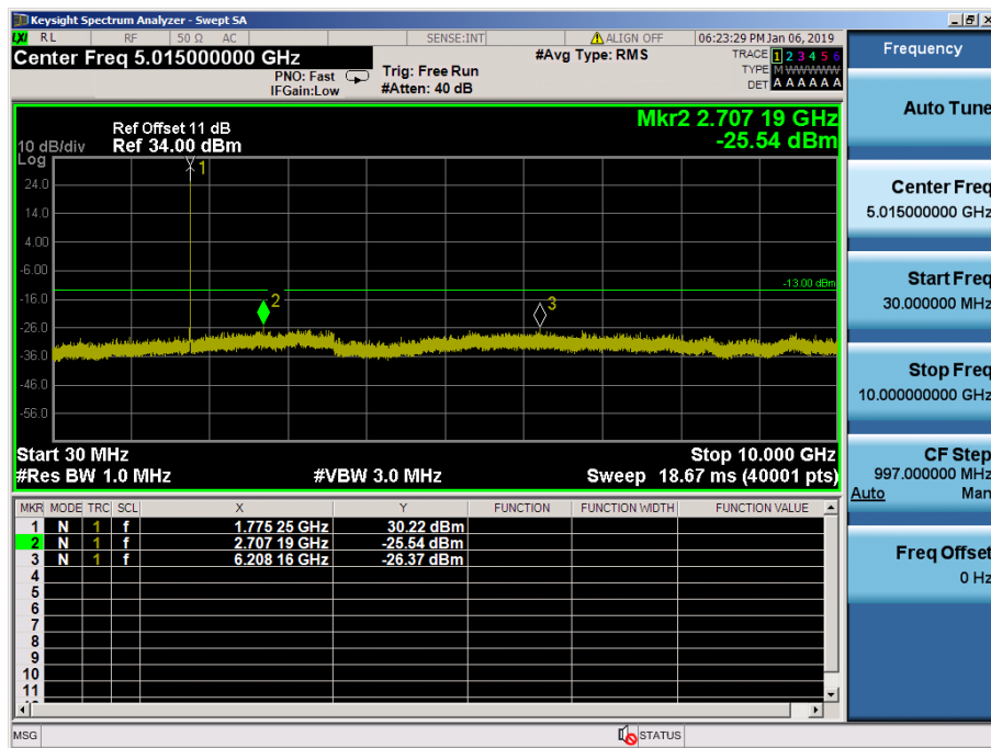
LTE Band 66, 4 / 10MHz / QPSK - RB Size/Offset (1/25) – High Channel
