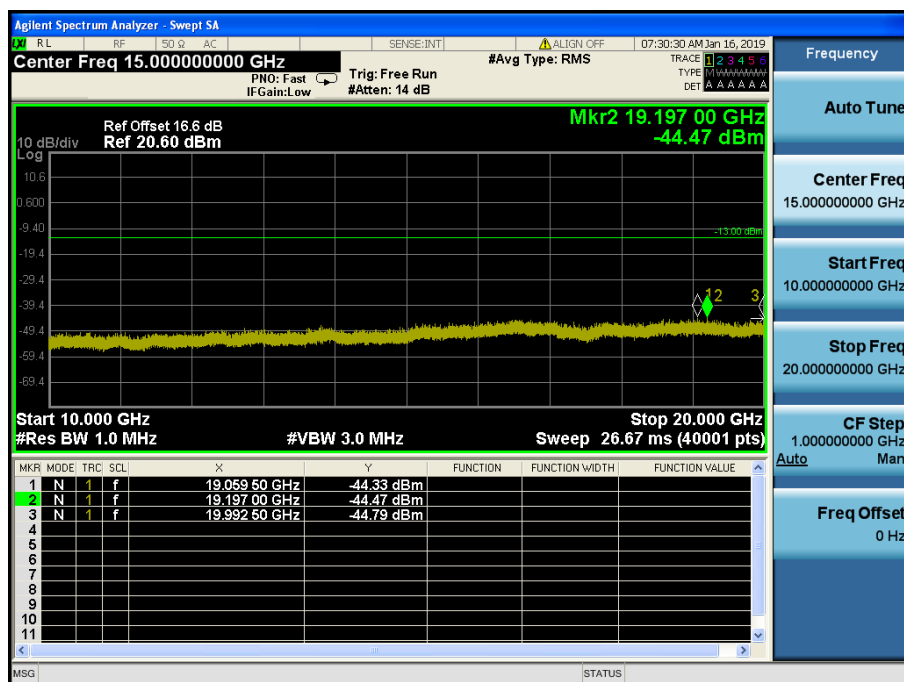
LTE Band 2 / 3MHz / 64QAM - RB Size/Offset (8/0) – High Channel
