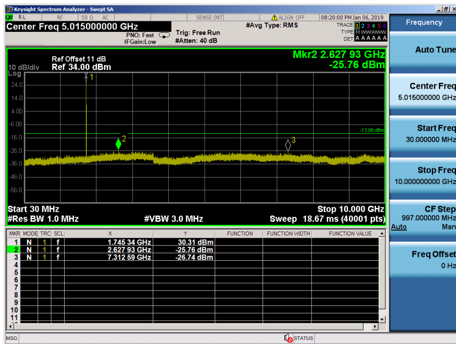
LTE Band 66, 4 / 1.4MHz / 16QAM - RB Size/Offset (3/2) – Mid Channel
