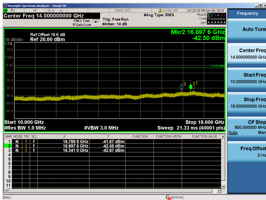
LTE Band 66, 4 / 10MHz / 16QAM - RB Size/Offset (25/12) – Mid Channel
