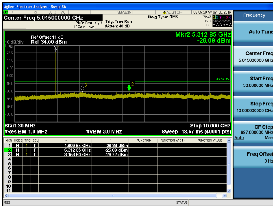
LTE Band 2 / 5MHz / 64QAM - RB Size/Offset (1/24) – High Channel
