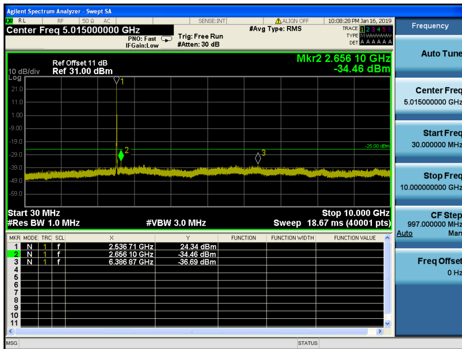
LTE Band 7 / 10MHz / 16QAM - RB Size/Offset (25/25) – Mid Channel
