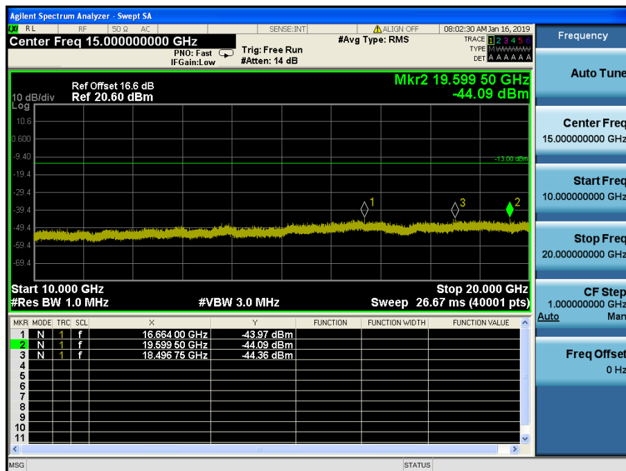
LTE Band 2 / 5MHz / 64QAM - RB Size/Offset (25/0) – Mid Channel
