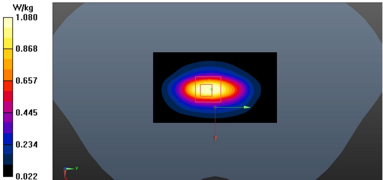
Fig.8 WCDMA Band 4 Body
