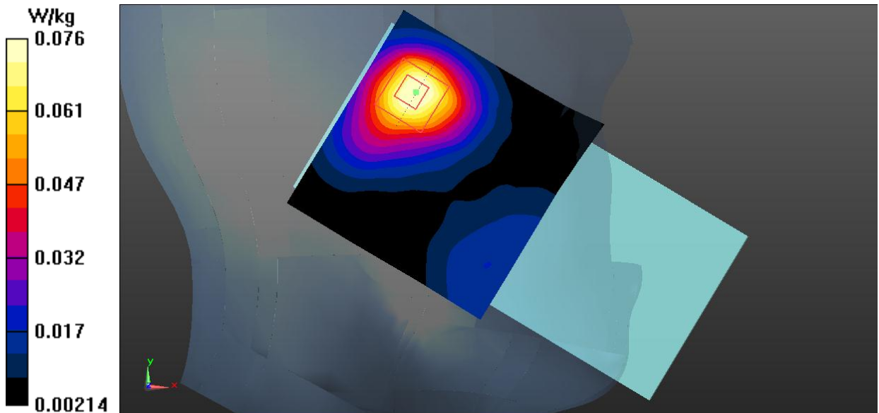
Fig.3 PCS1900 Head
