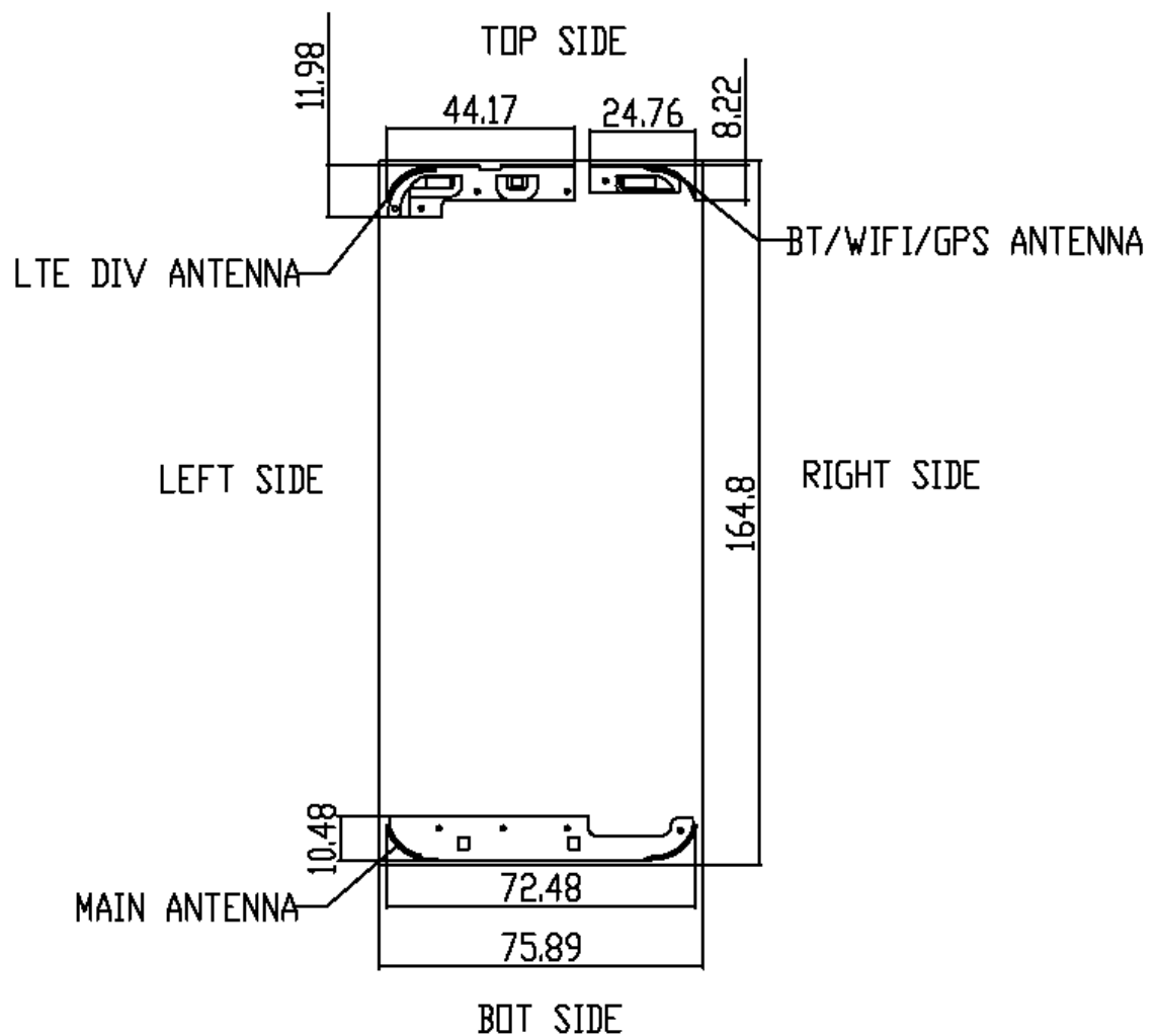
Picture 11.1 Antenna Locations (Front View)
