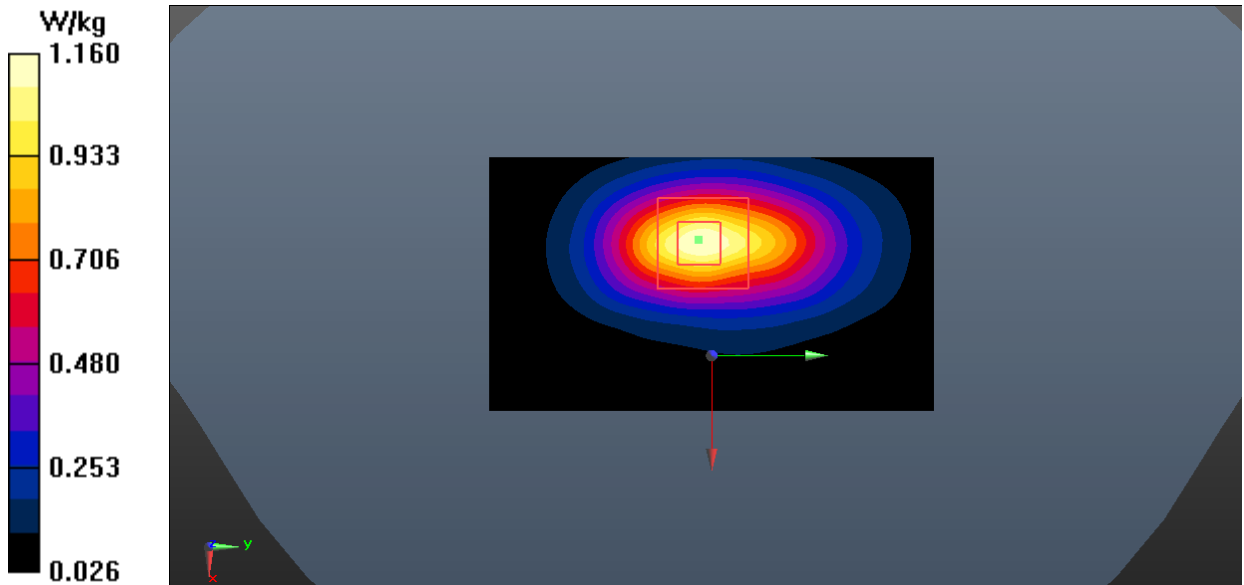
Fig.4 PCS1900 Body
