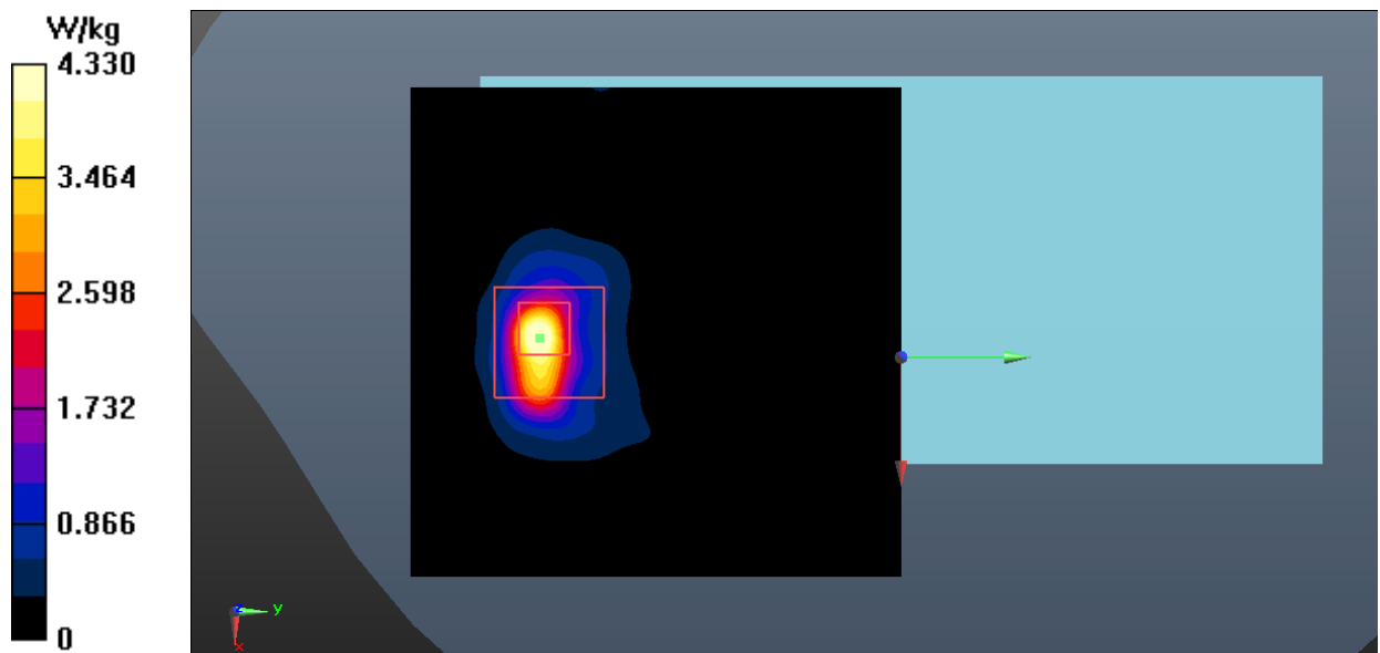
Fig.31 WLAN 5GHz Extremity
