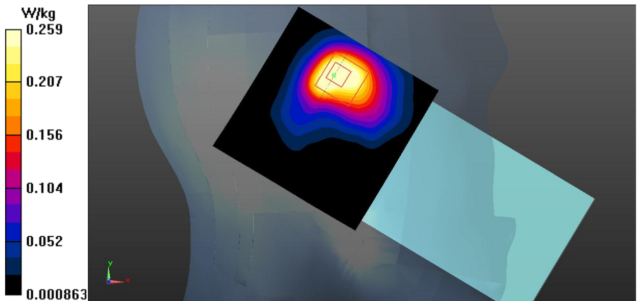
Fig.27 WLAN 2.4GHz Head
