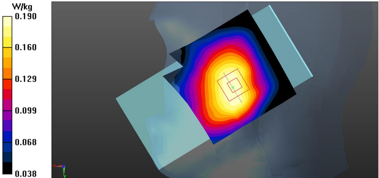
Fig.21 LTE Band 28 Head
