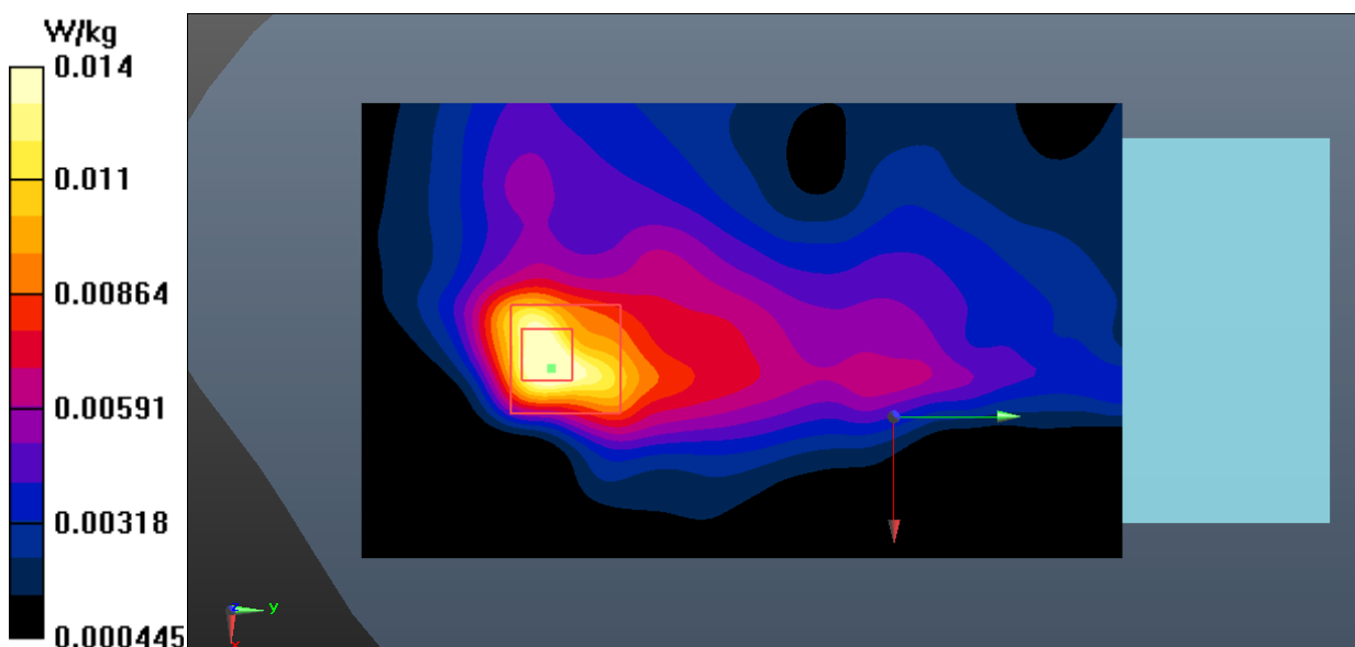
Fig.26 Bluetooth Body
