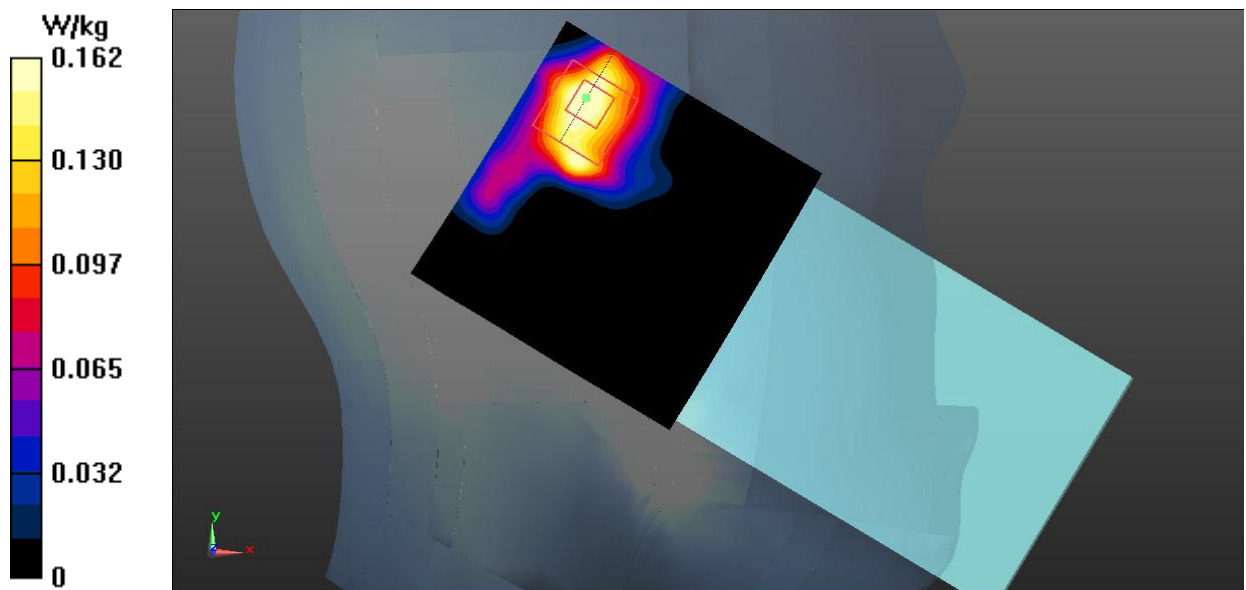
Fig.29 WLAN 5GHz Head
