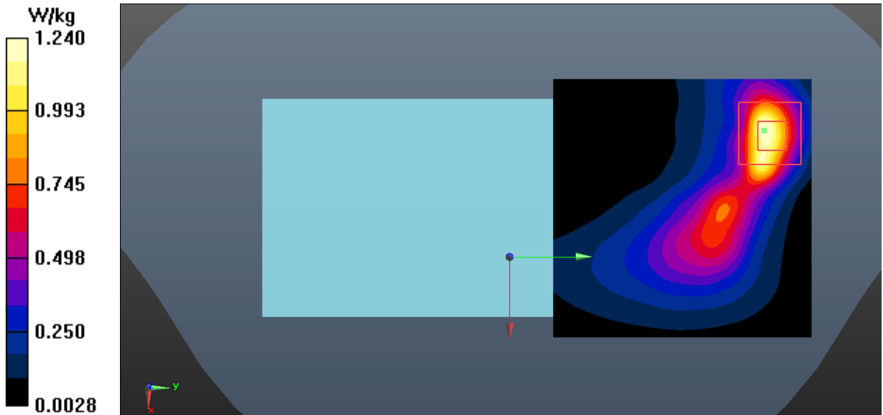
Fig.16 LTE Band 7 Body
