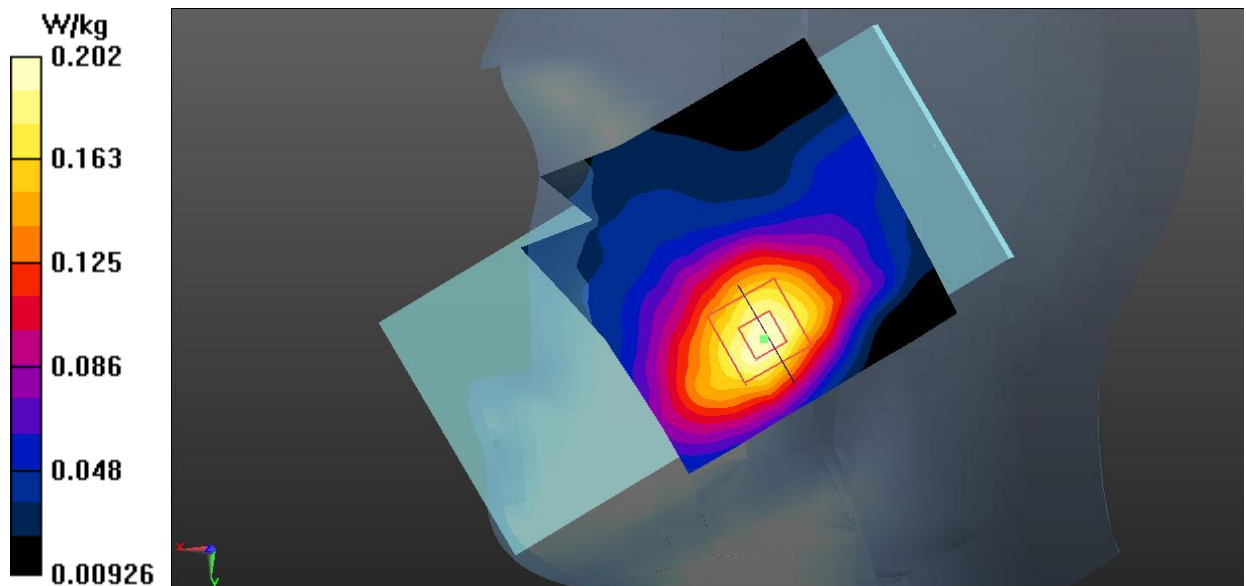
Fig.7 WCDMA Band 4 Head
