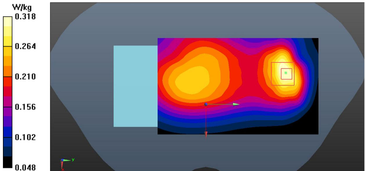
Fig.14 LTE Band 5 Body
