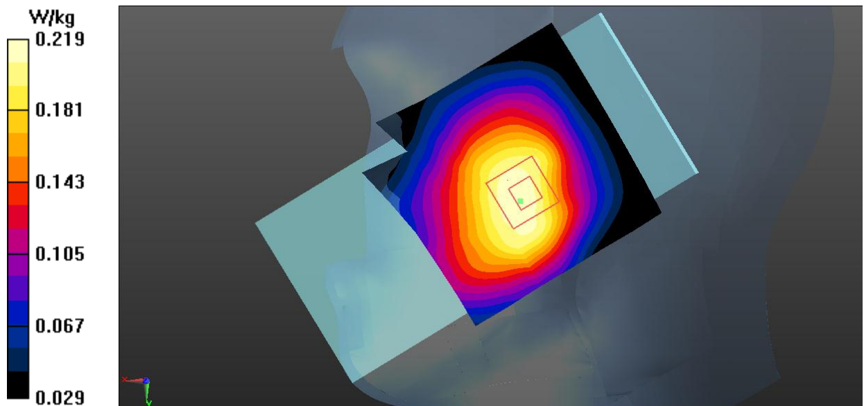
Fig.9 WCDMA Band 5 Head
