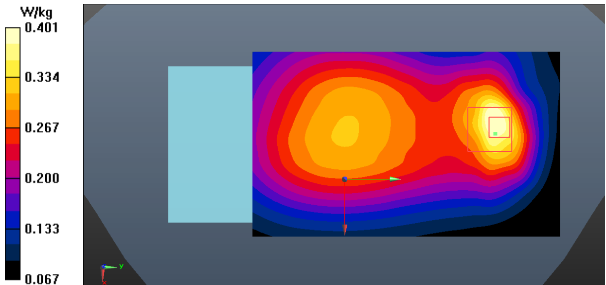
Fig.22 LTE Band 28 Body
