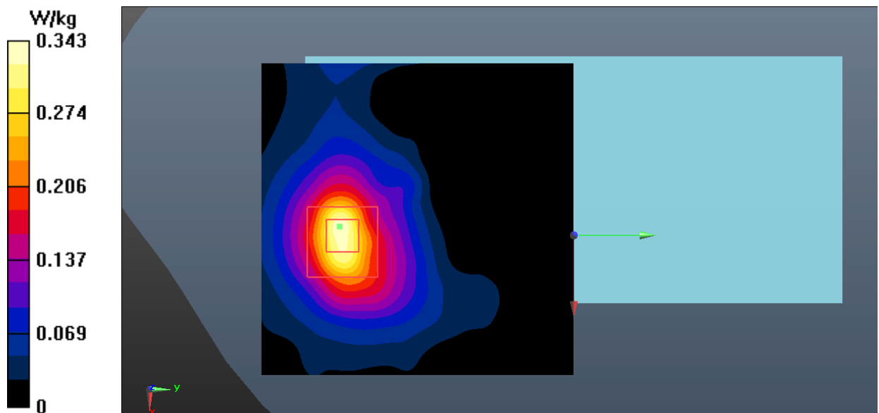
Fig.30 WLAN 5GHz Body
