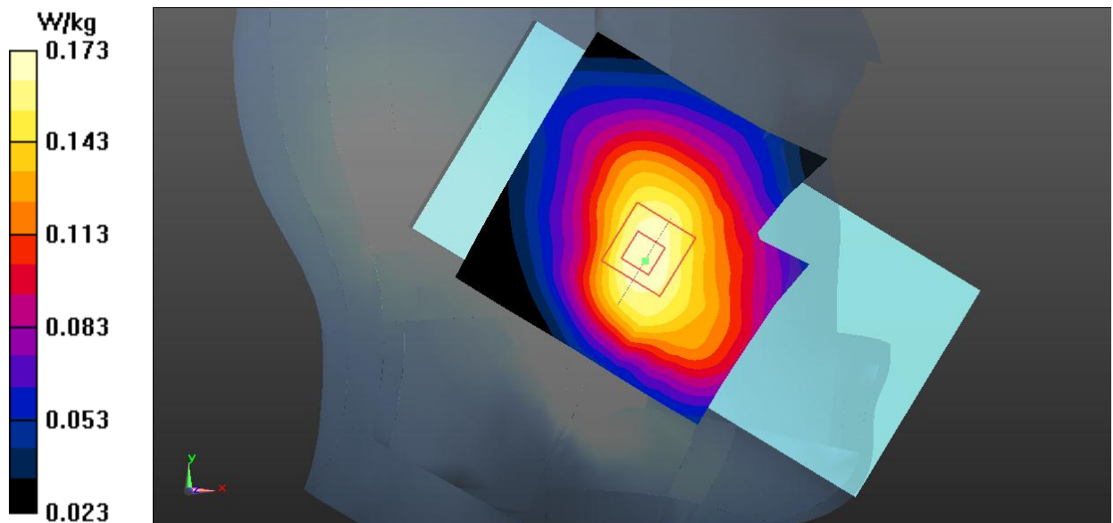
Fig.19 LTE Band 13 Head
