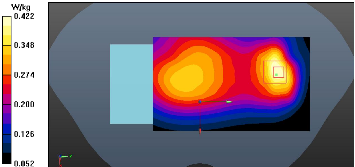
Fig.2 GSM850 Body
