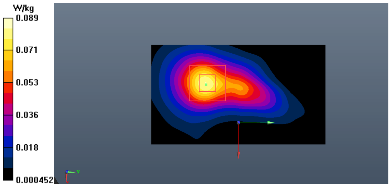
Fig.28 WLAN 2.4GHz Body
