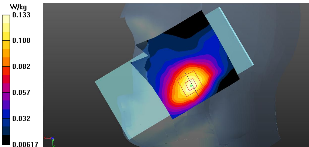
Fig.23 LTE Band 66 Head
