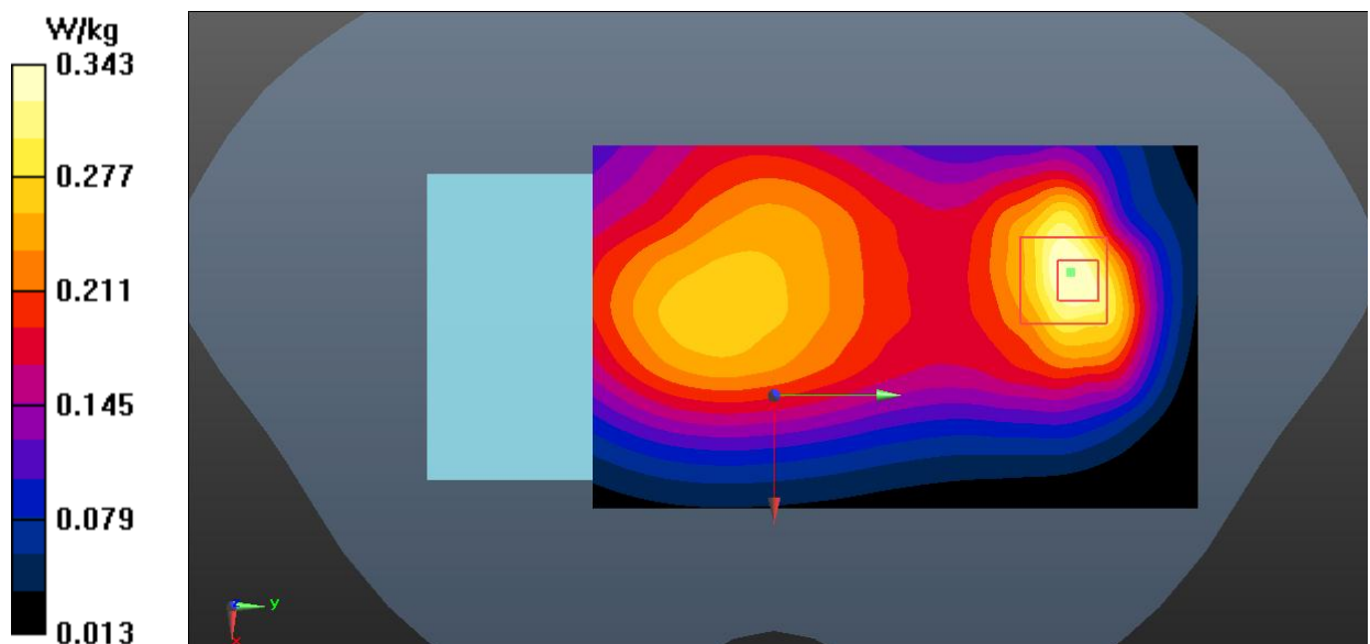
Fig.10 WCDMA Band 5 Body
