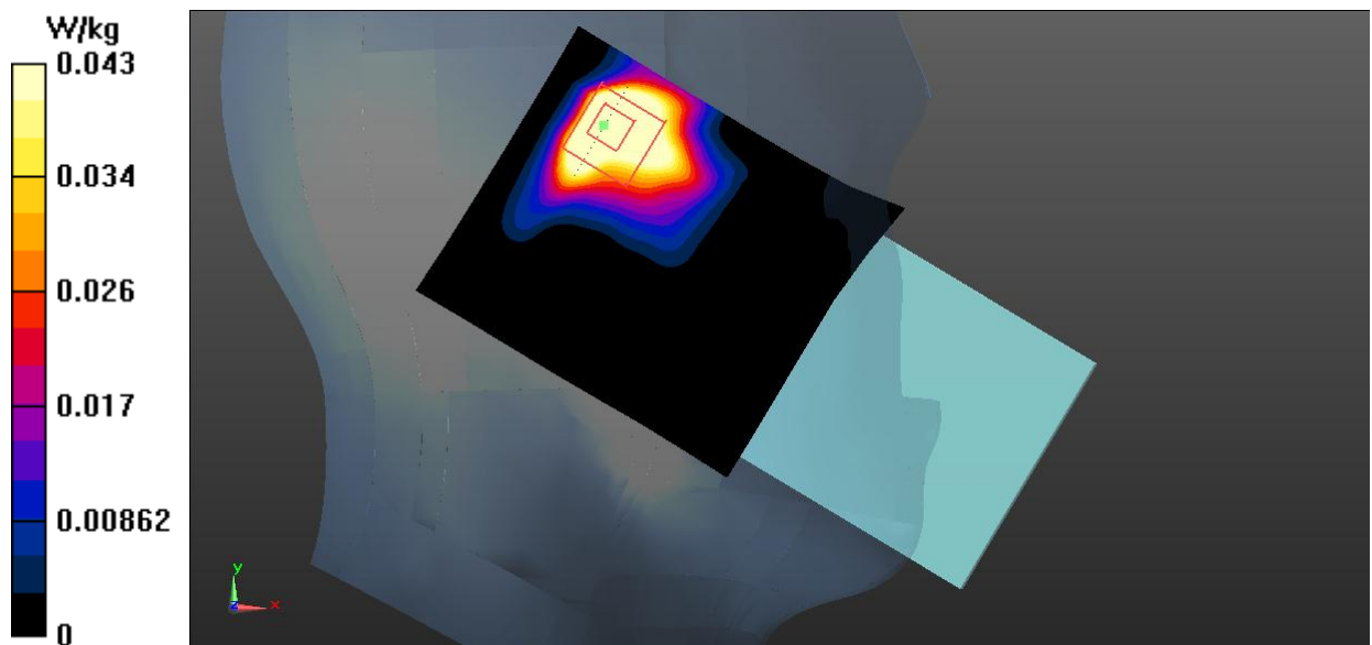
Fig.25 Bluetooth Head
