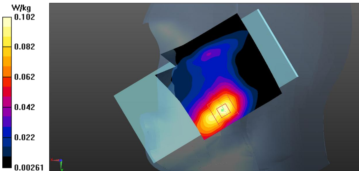
Fig.15 LTE Band 7 Head
