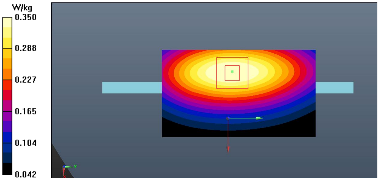
Fig.18 LTE Band 12 Body
