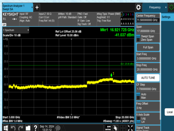
Band7-10MHz-QPSK-21100-1RB#0-3000~20000-PASS
