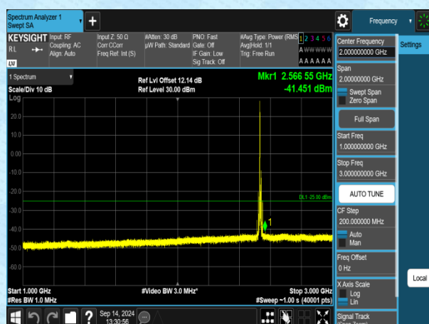
Band7-10MHz-QPSK-21100-1RB#0-1000~3000-PASS
