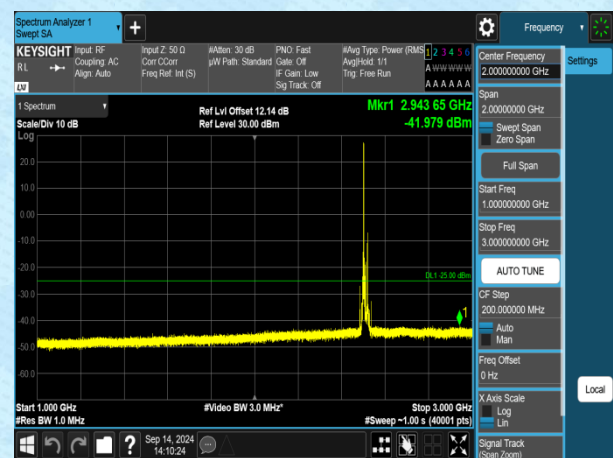
Band7-20MHz-QPSK-20850-1RB#0-1000~3000-PASS
