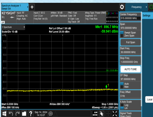
Band7-20MHz-QPSK-20850-1RB#0-30~1000-PASS
