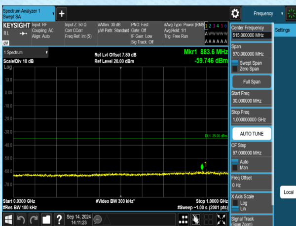
Band7-20MHz-QPSK-21100-1RB#0-30~1000-PASS
