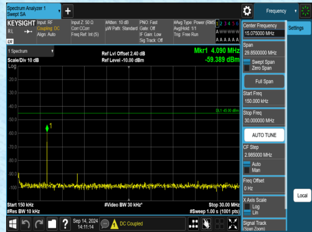
Band7-20MHz-QPSK-21100-1RB#0-0.15~30-PASS
