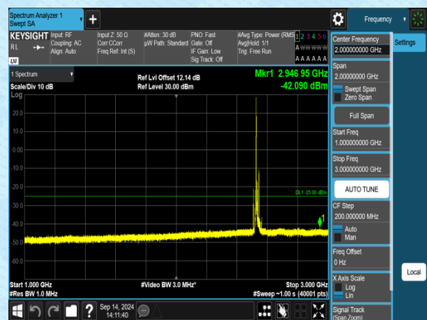
Band7-20MHz-QPSK-21100-1RB#0-1000~3000-PASS
