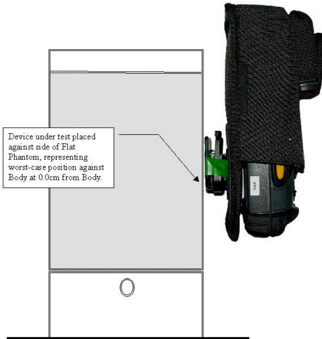
Figure 14. – MC9062 Test position for body assessment in declared normal use position; holster belt clip 0.0 cm from phantom side.
