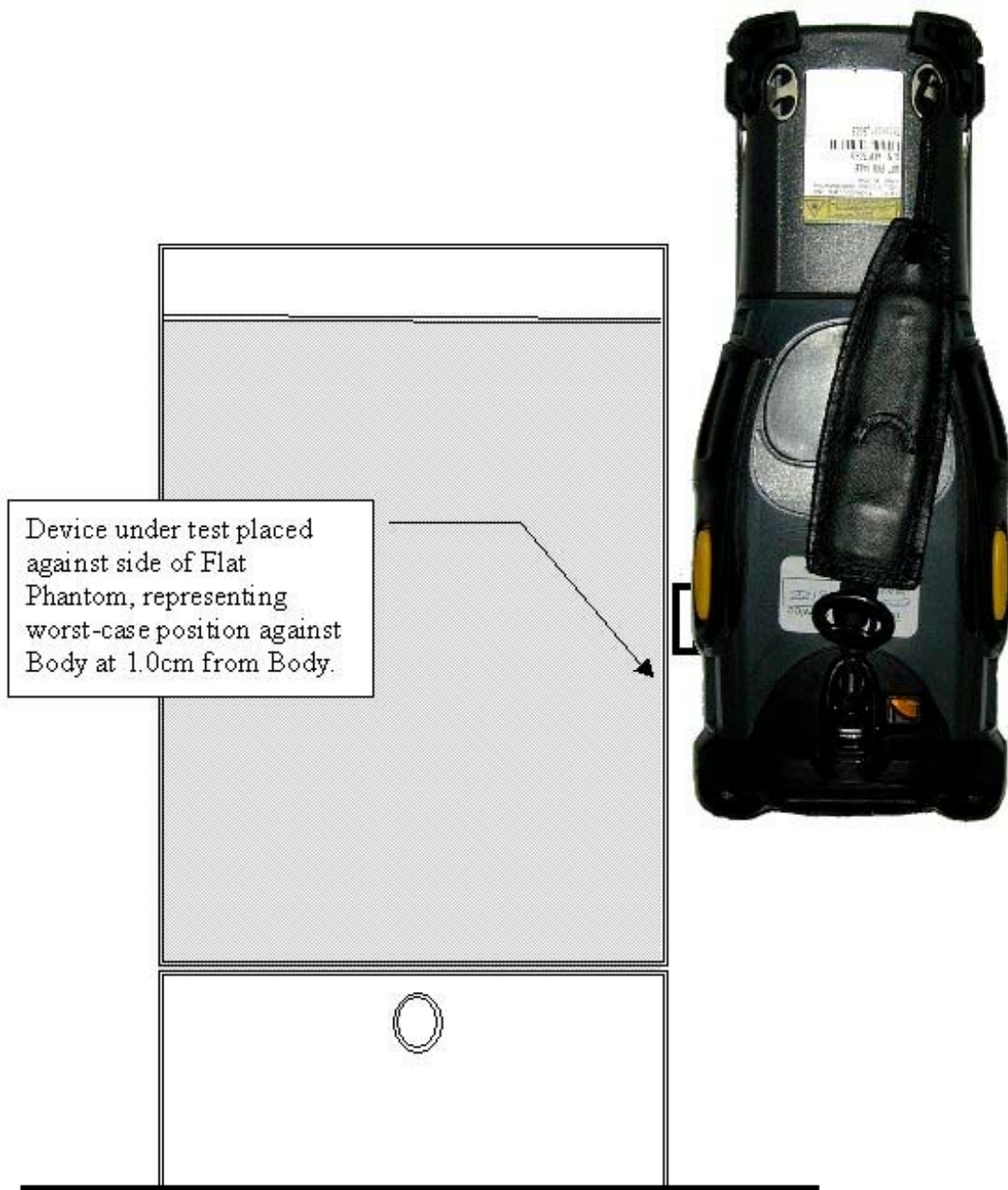
Figure 15. – MC9062 Test Position for WLAN Mode; 1.0 cm from phantom side
