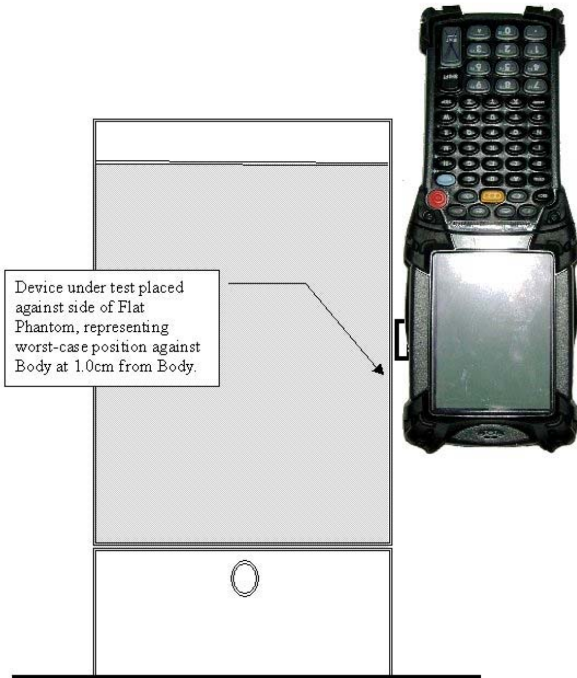
Figure 16. – MC9062 Test Position for Bluetooth Mode; 1.0 cm from phantom side
